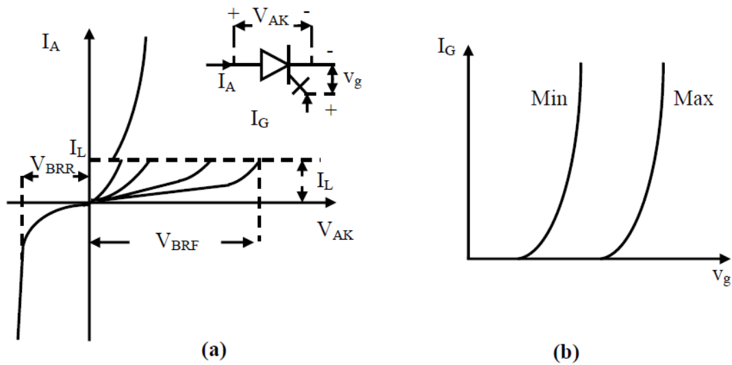
Fig. 5.3: Steady state characteristics of a GTO (a) Output characteristics; (b) Gate characteristics.
