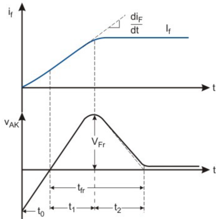
Forward current and voltage waveforms of a power diode during Turn On operation.
