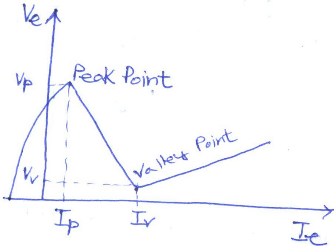
V-I characteristics of UJT
