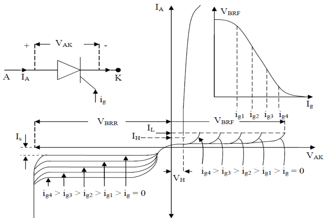
Fig. 4.3: Static output characteristics of a Thyristor
