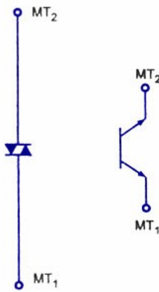
Schematic Symbols
