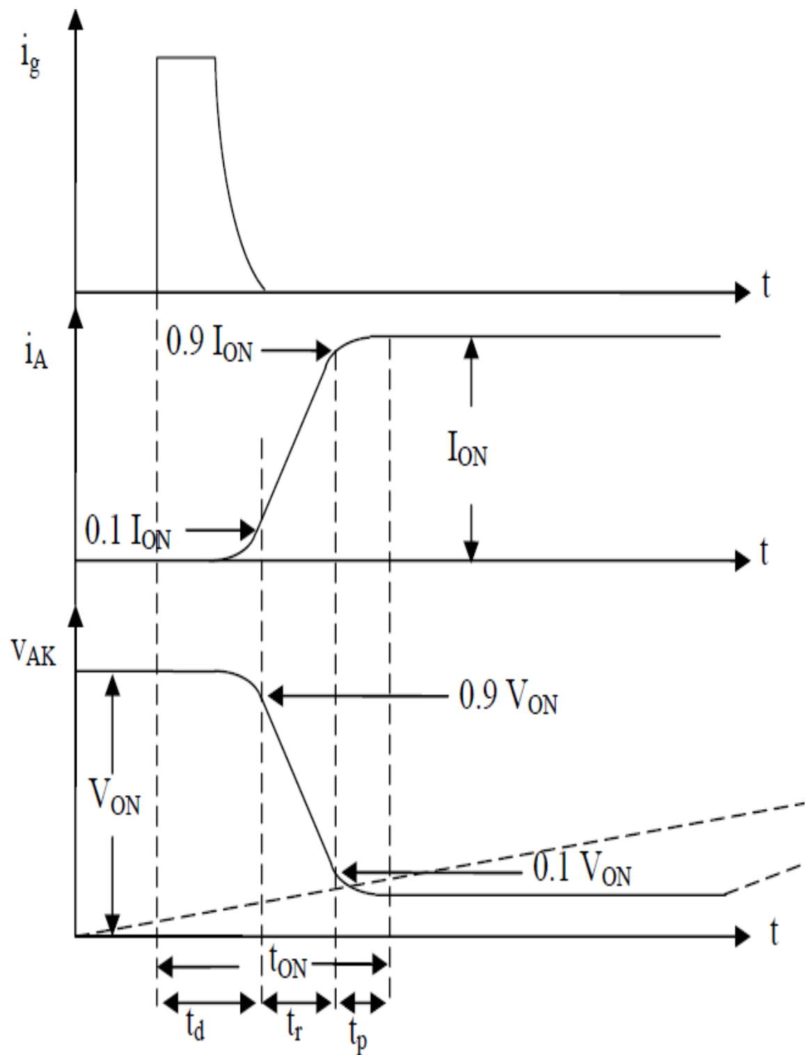
Turn on Switching Characteristics of a Thyristor
