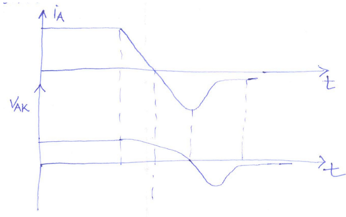
Turn off Switching Characteristics of a Thyristor
