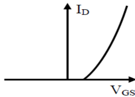
n-channel enhancement type MOSFET
