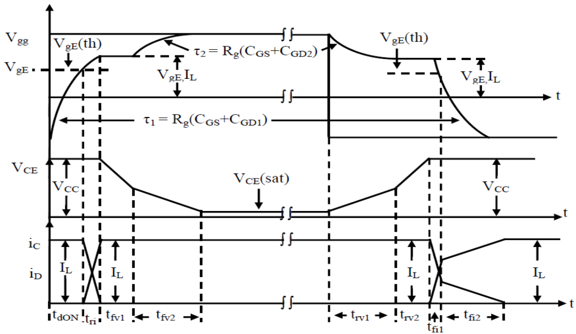
Fig. 7.6: Switching waveforms of an IGBT.
