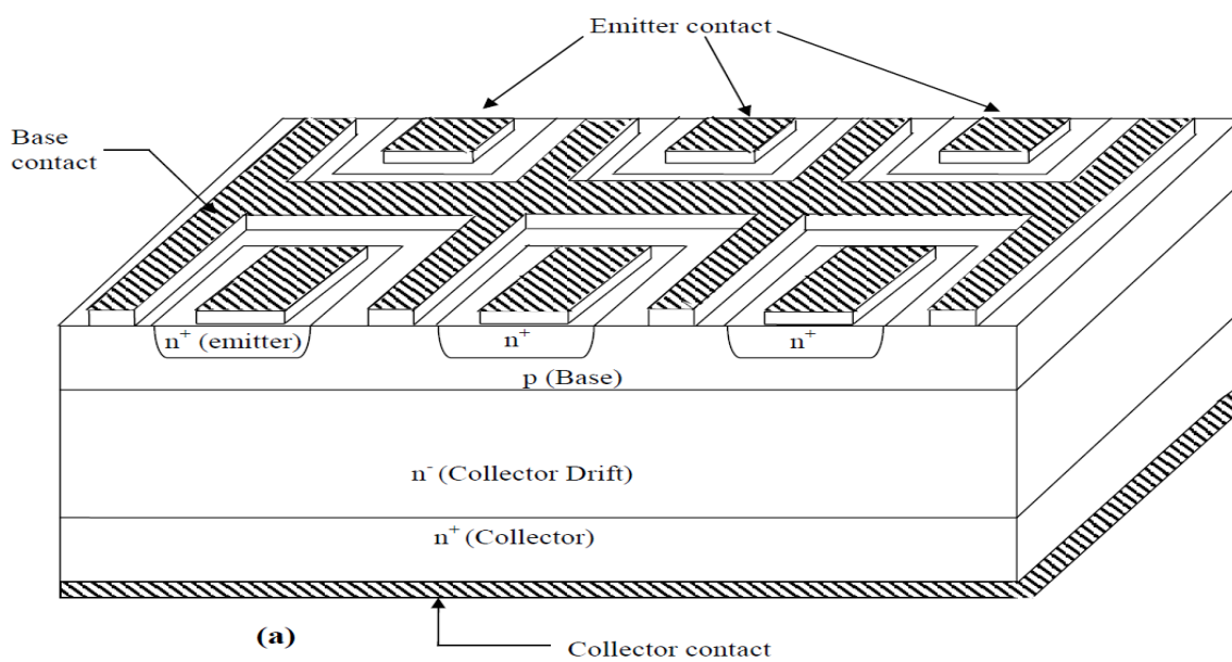
Power Bipolar Junction Transistor (BJT)
