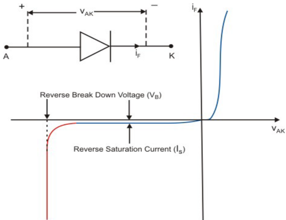
Volt-Ampere ( i-v ) characteristics of a p-n junction diode
