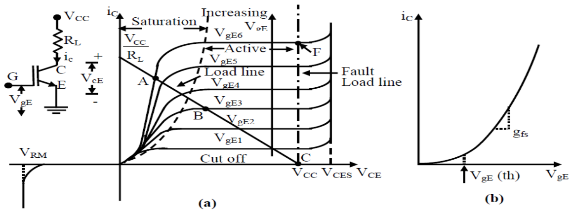
Fig. 7.4: Static characteristics of an IGBT
