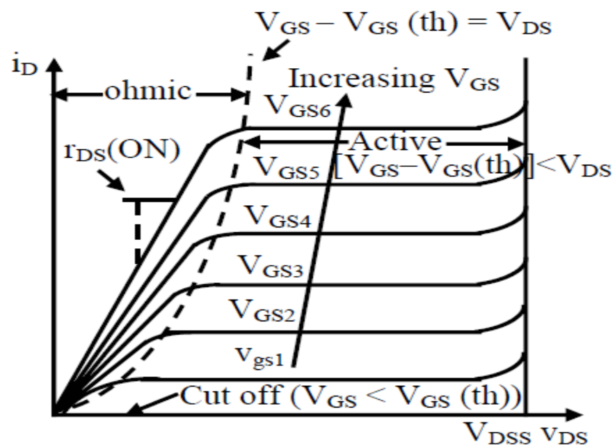
Output i-v characteristics of a Power MOSFET
