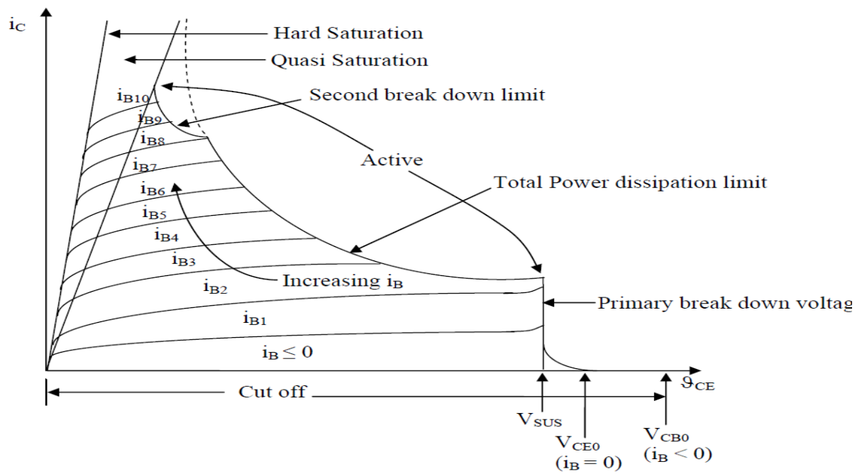
Fig. 3.4 Output ( i_c - v_{CE} ) characteristics of an n – p – n type Power Transistor
