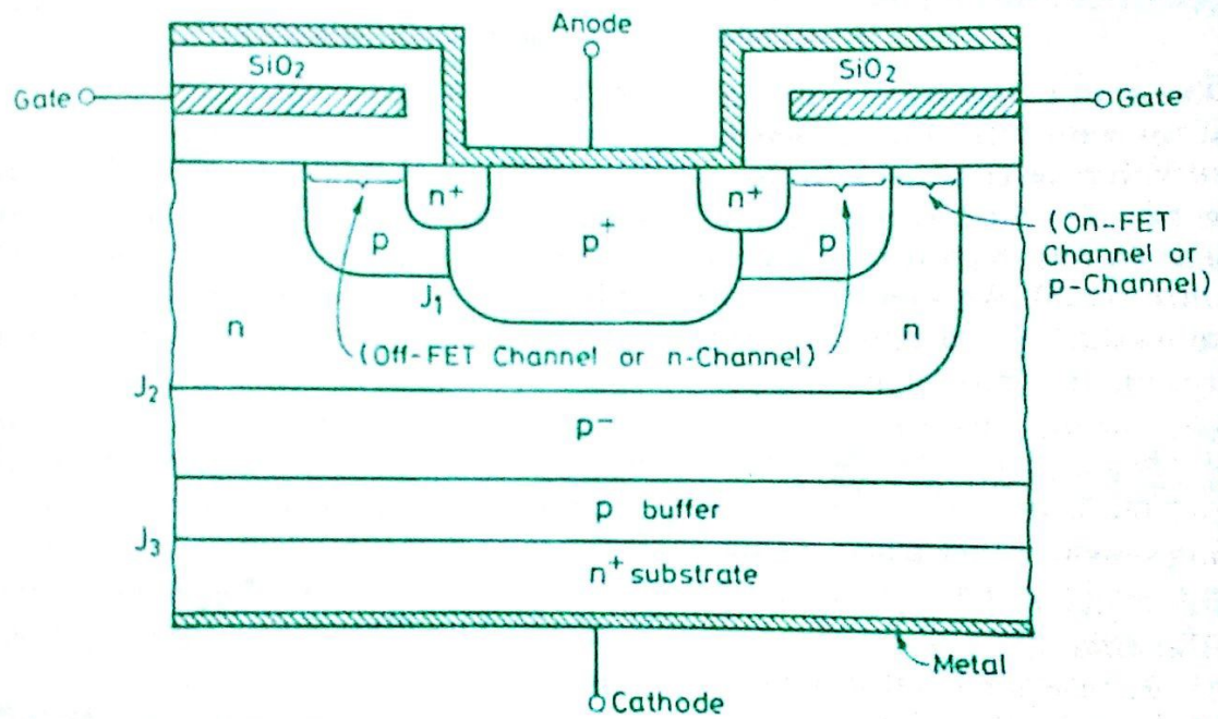
Fig. 2.27. Basic structure of an MCT.
