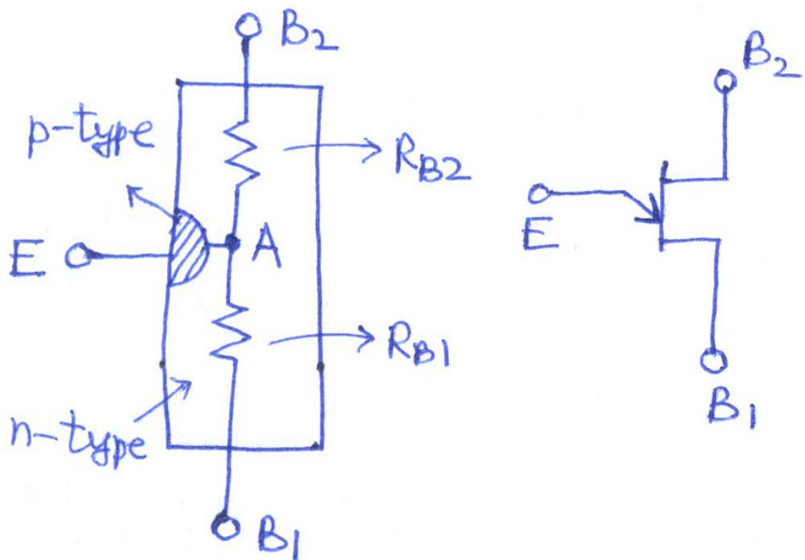
UJT Construction and Symbol
