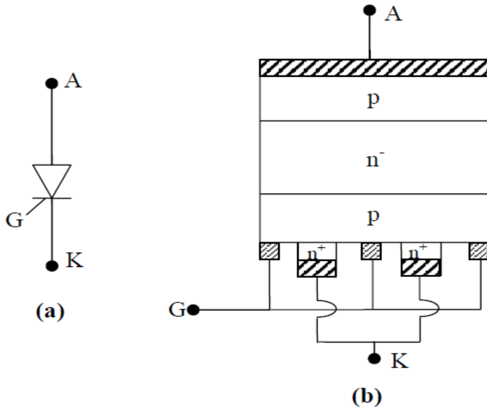
Constructional features of a thyristor (a) Circuit Symbol, (b) Schematic Construction
