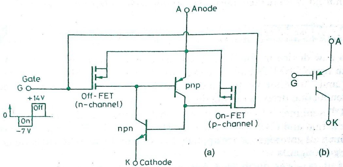
Fig. 2.28. MCT (a) equivalent circuit and (b) circuit symbol.
