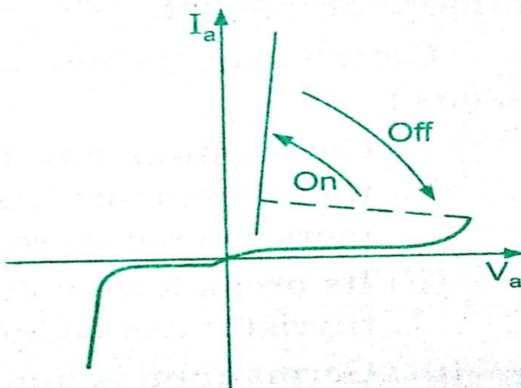
Fig. 2.29. Static I-V characteristics of an MCT.
