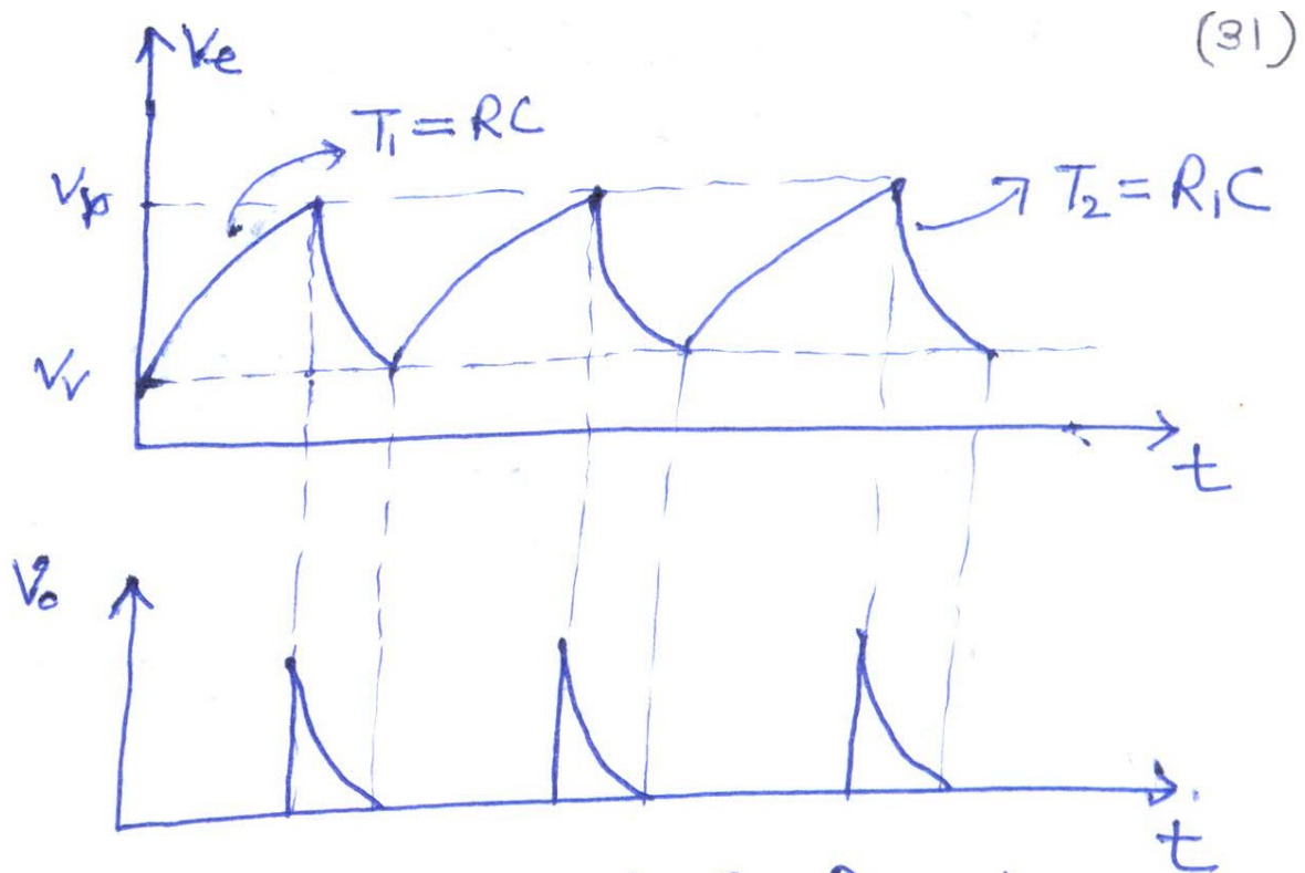
UJT Oscillator Voltage Waveforms
