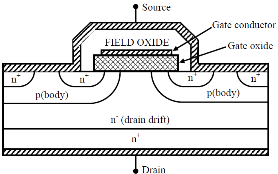
Schematic construction of a power MOSFET
