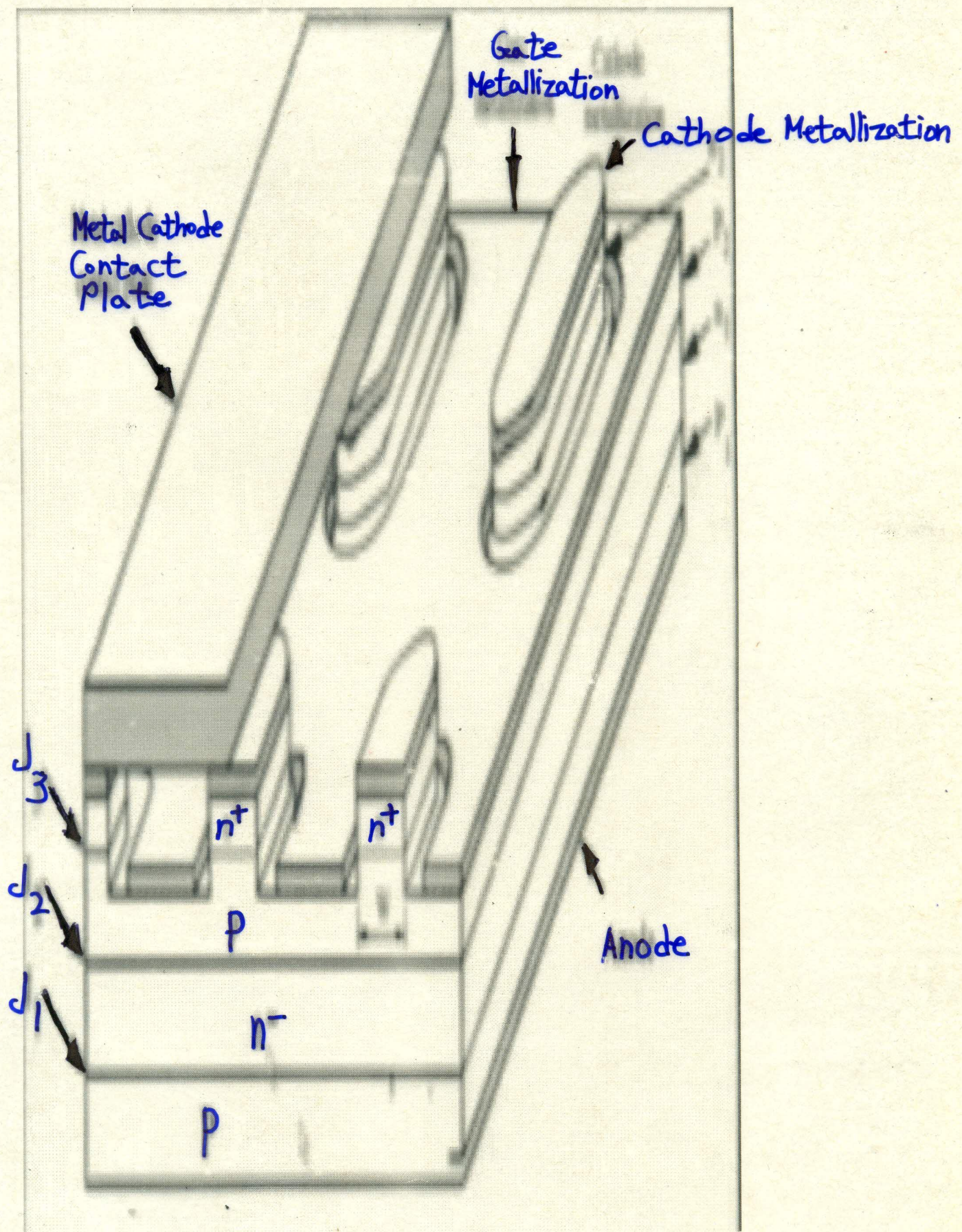
Vertical Cross Section & Perspective View of a GTO
