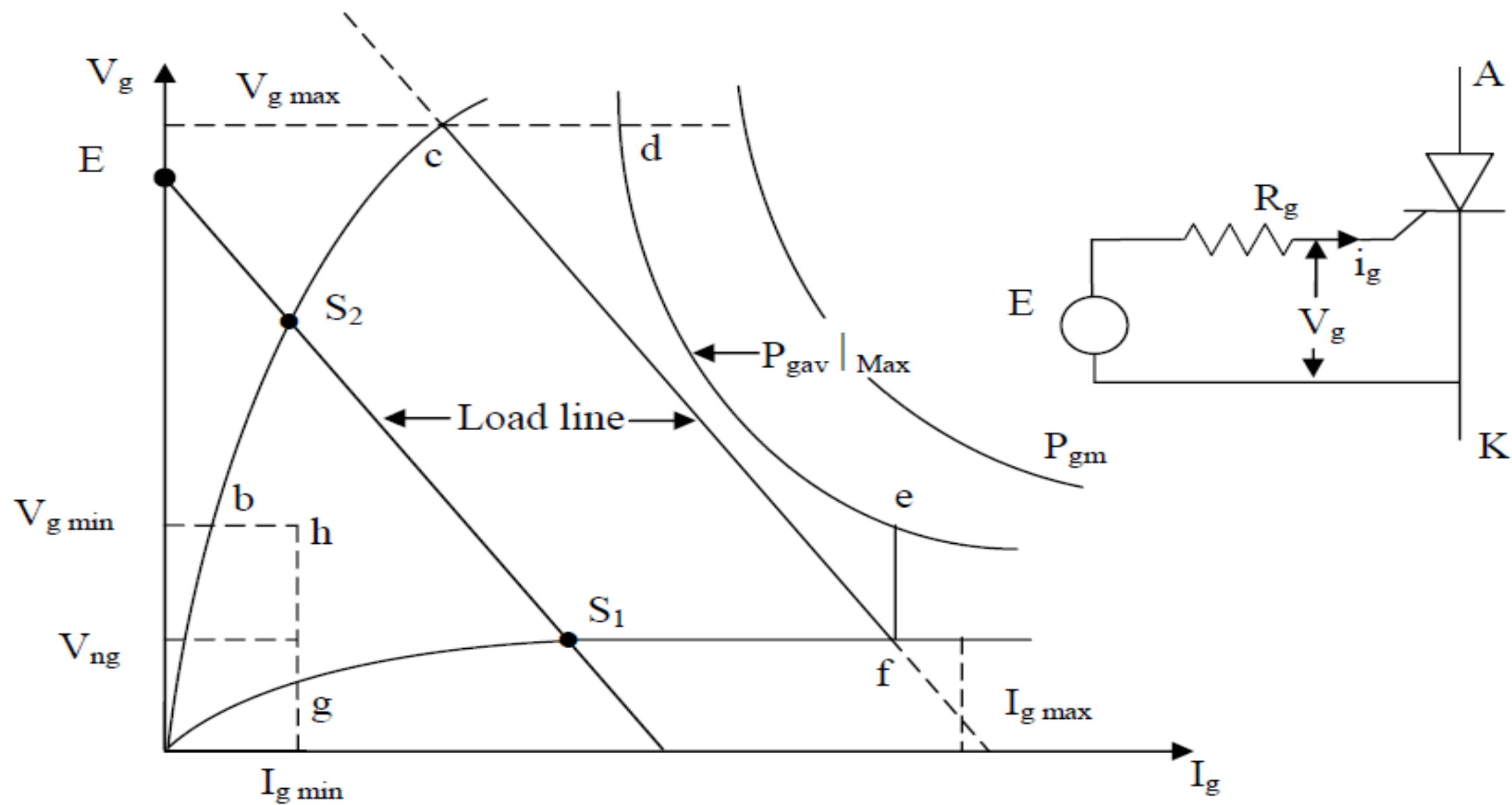
Fig. 4.5: Gate characteristics of a thyristor.
