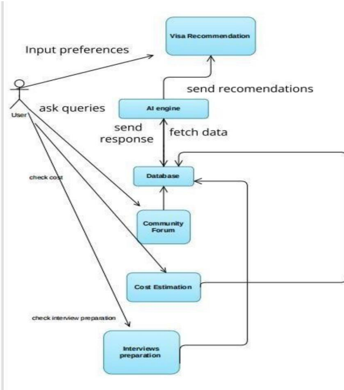
Figure 2.2.3: Collaboration diagram
