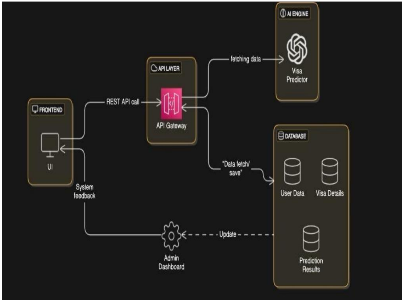
Figure 2.2.11: Component diagram
