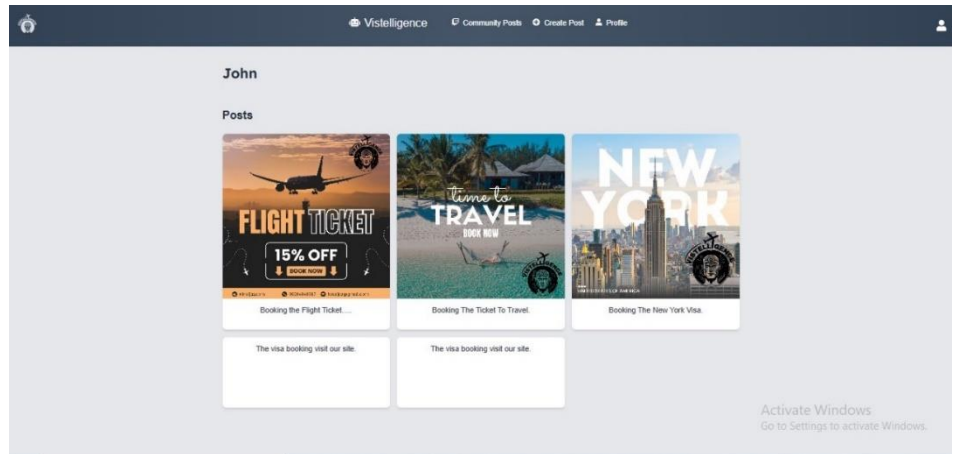
Figure 2: Profile
