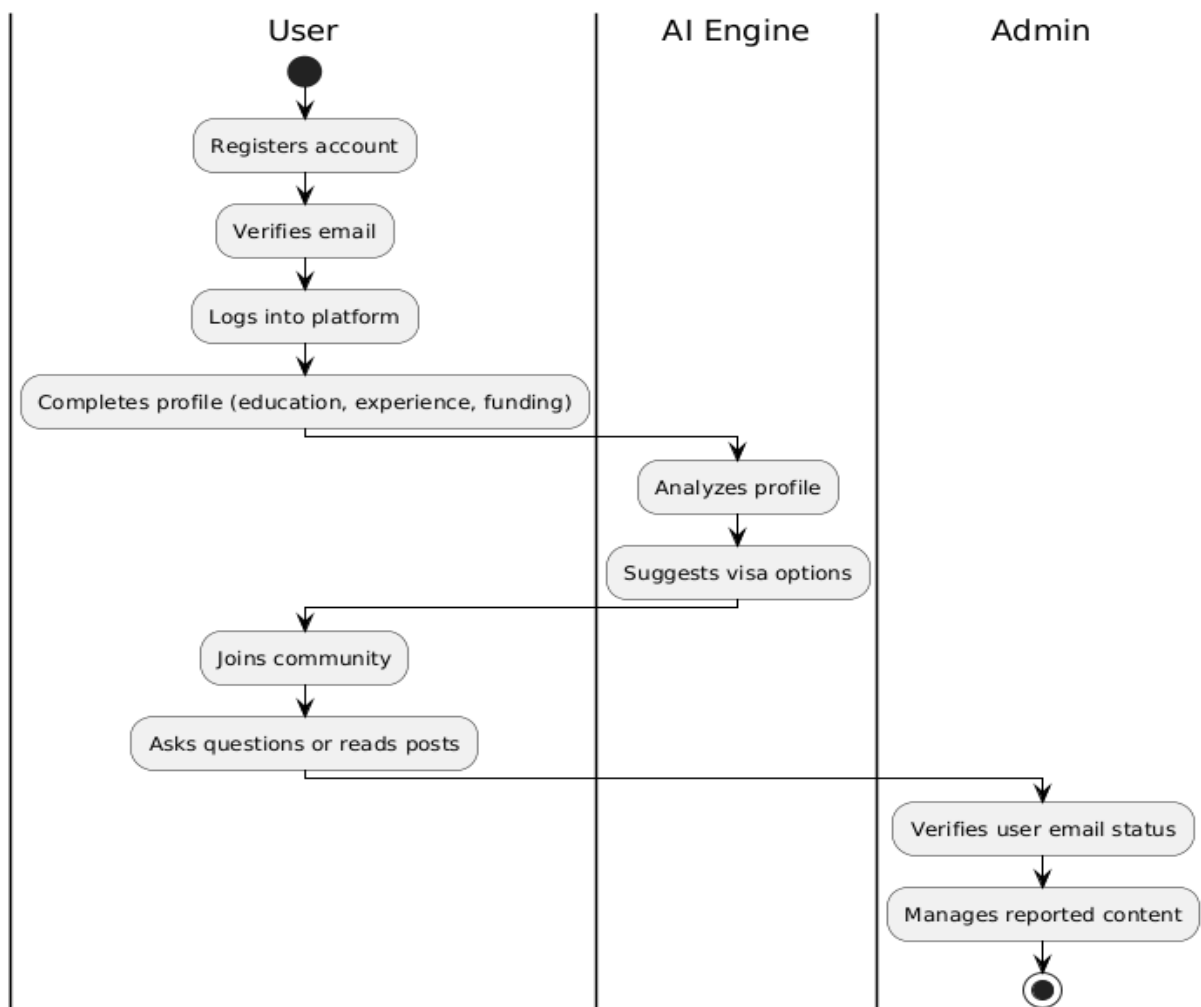
Figure 4.1: Swimlane daigram
