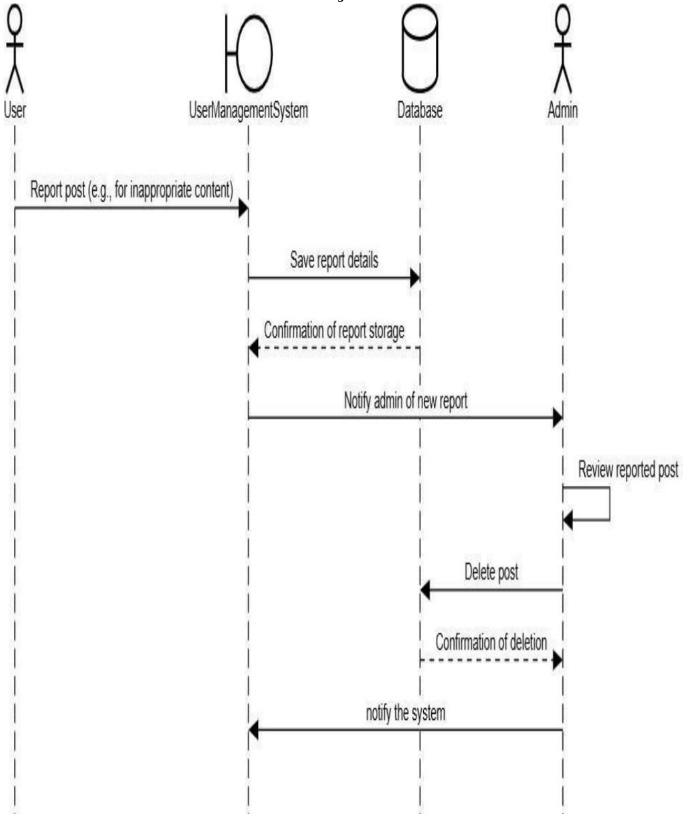
Figure 2.2.8: Report post
