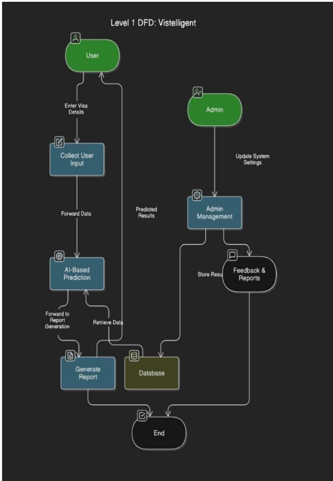
Figure 2.2.10: DFD
