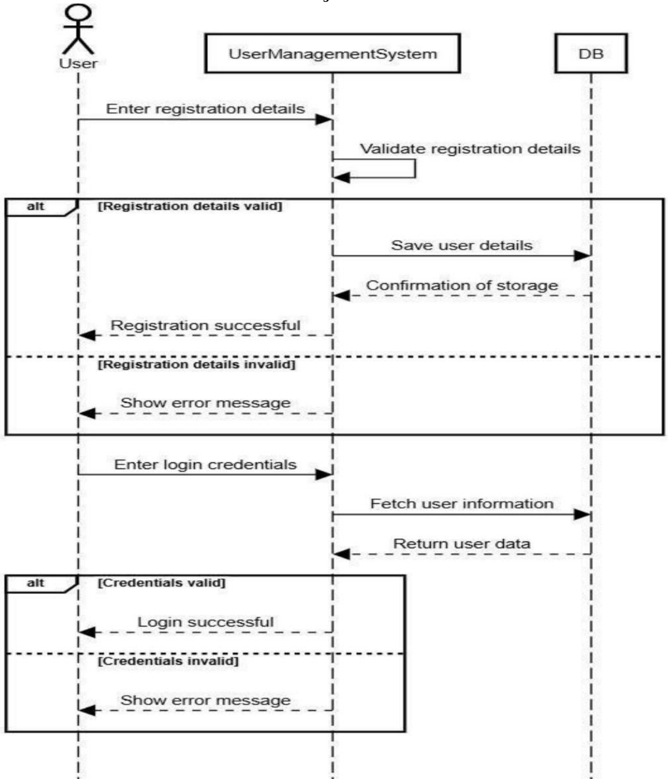
Figure 2.2.6: User Management
