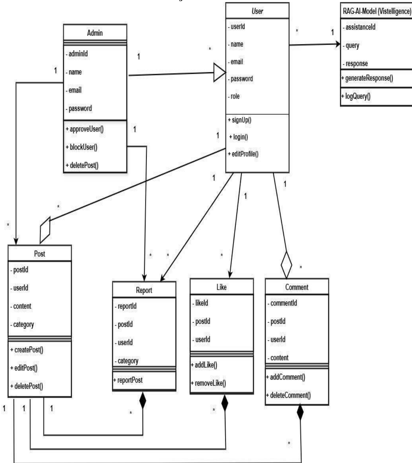
Figure 2.1.2: Class diagram
