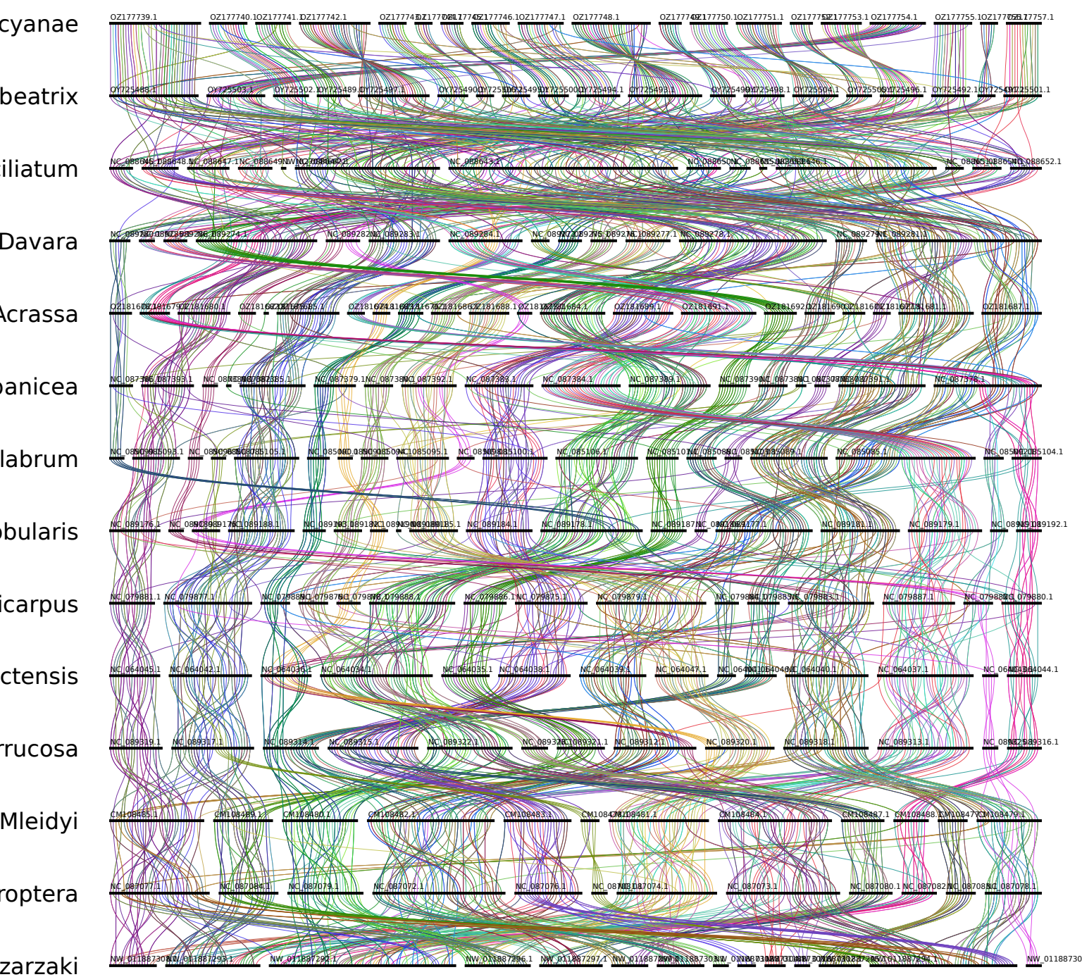
p<=0.05 RBH results (RBH-gene-coords)
