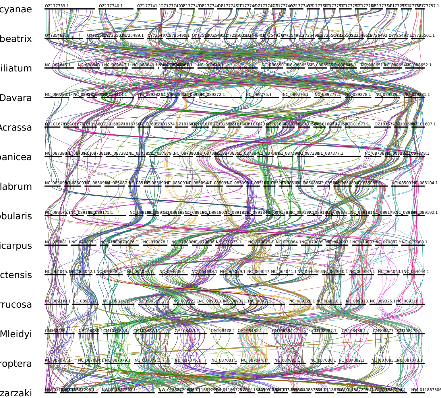
p<=0.05 RBH results (Chr-coords)
