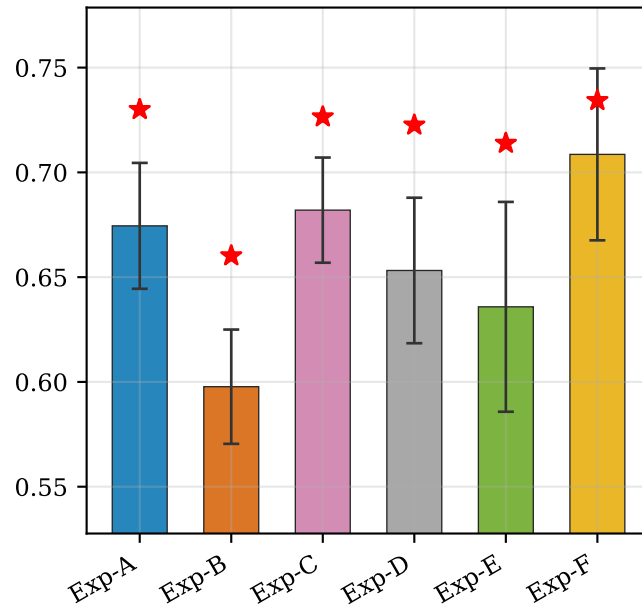
Recall
