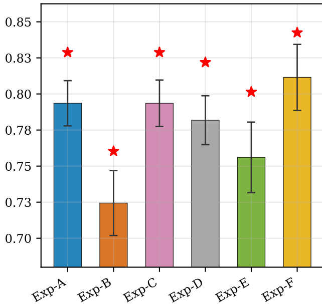
Accuracy
