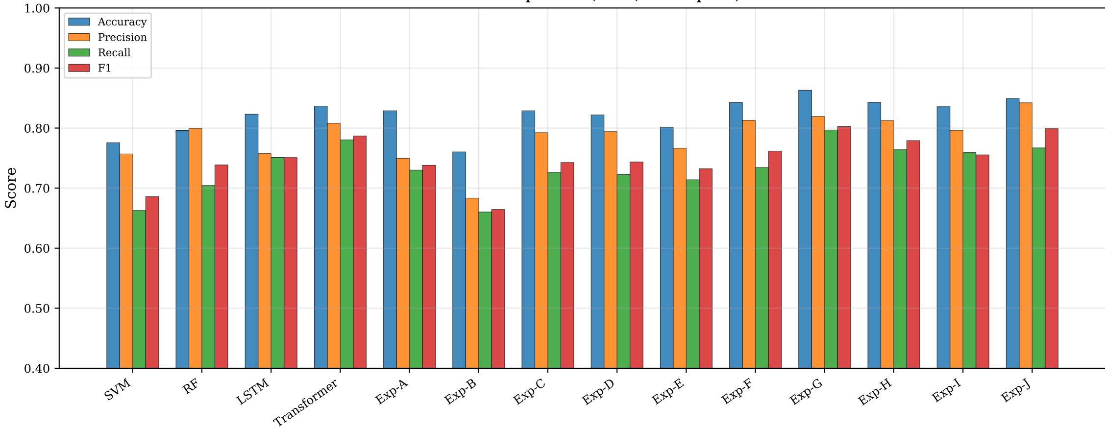
Method Comparison ( T = 3 , Best Epoch)
