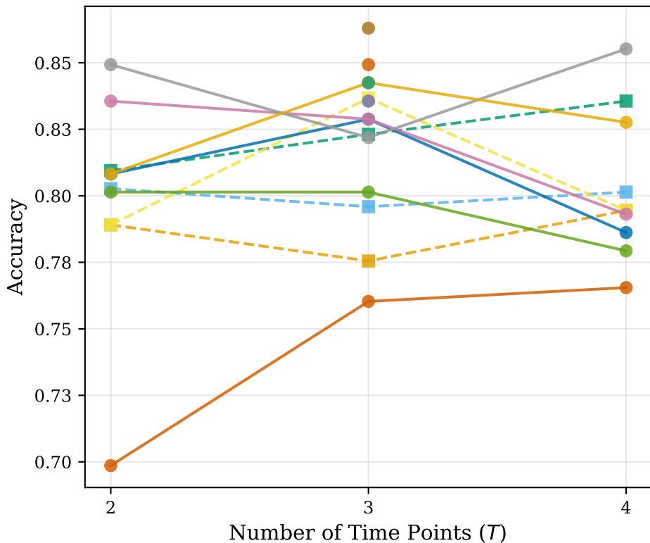
Best Accuracy vs. Temporal Resolution
