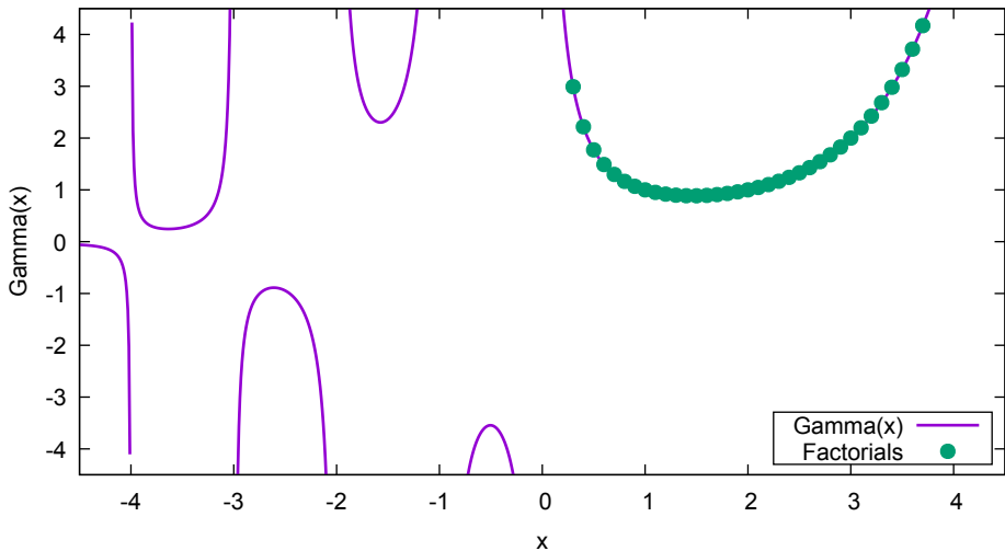
Gamma function
