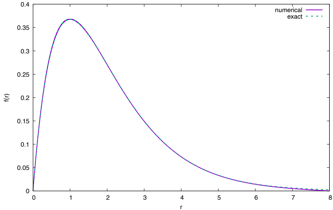
Hydrogen ground state
