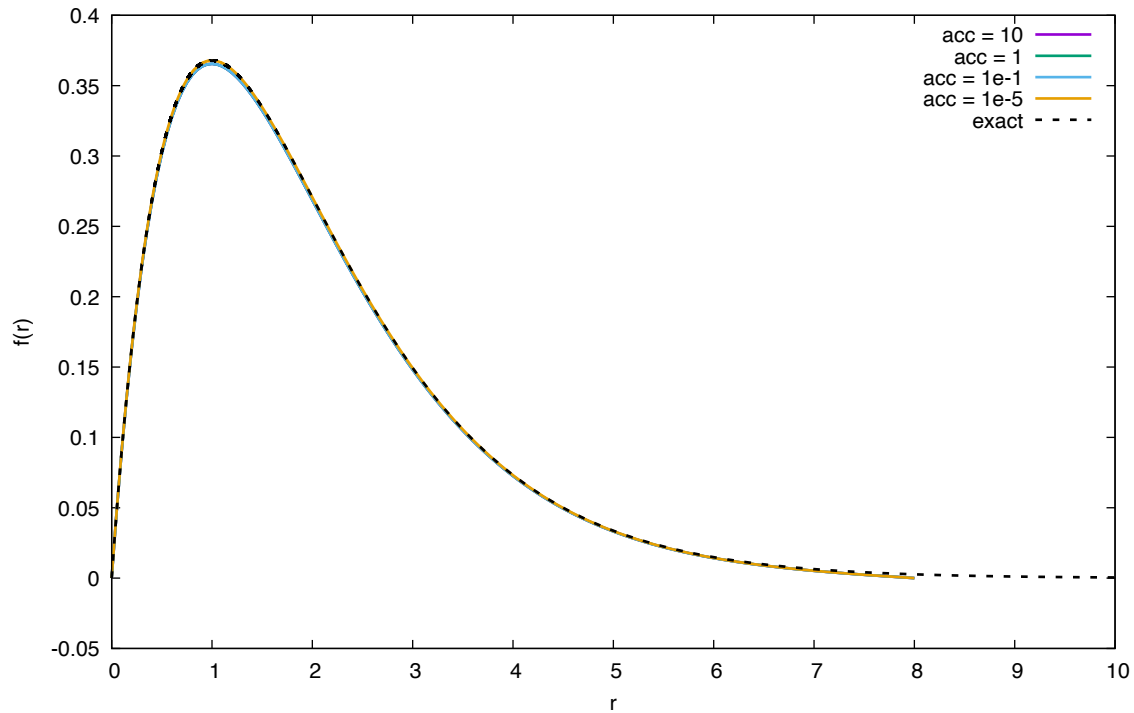
Hydrogen wavefunction - varying acc
