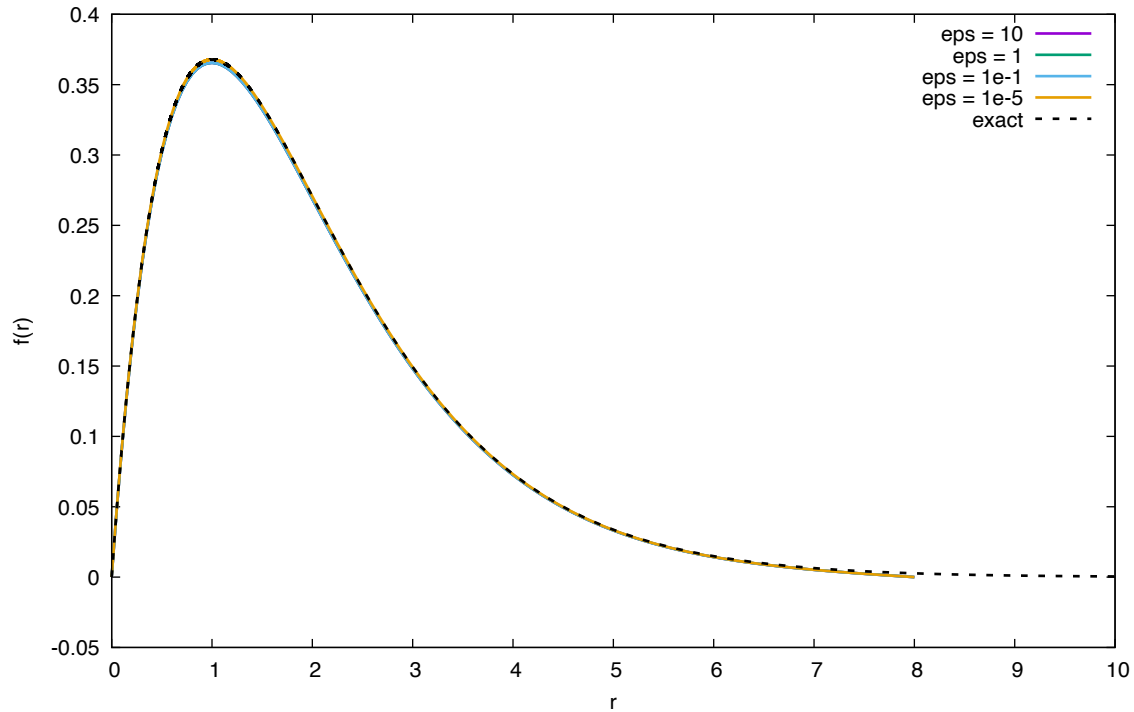
Hydrogen wavefunction - varying eps
