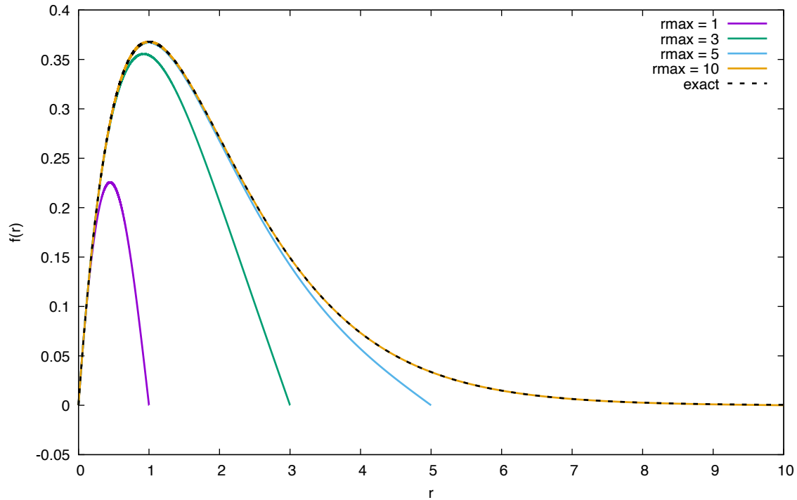
Hydrogen wavefunction - varying rmax
