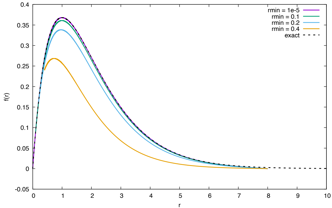
Hydrogen wavefunction - varying rmin
