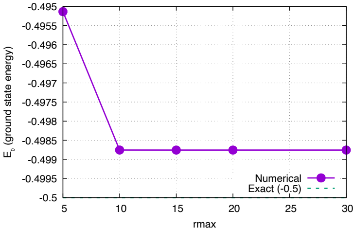
Convergence vs rmax ( \Delta r fixed)
