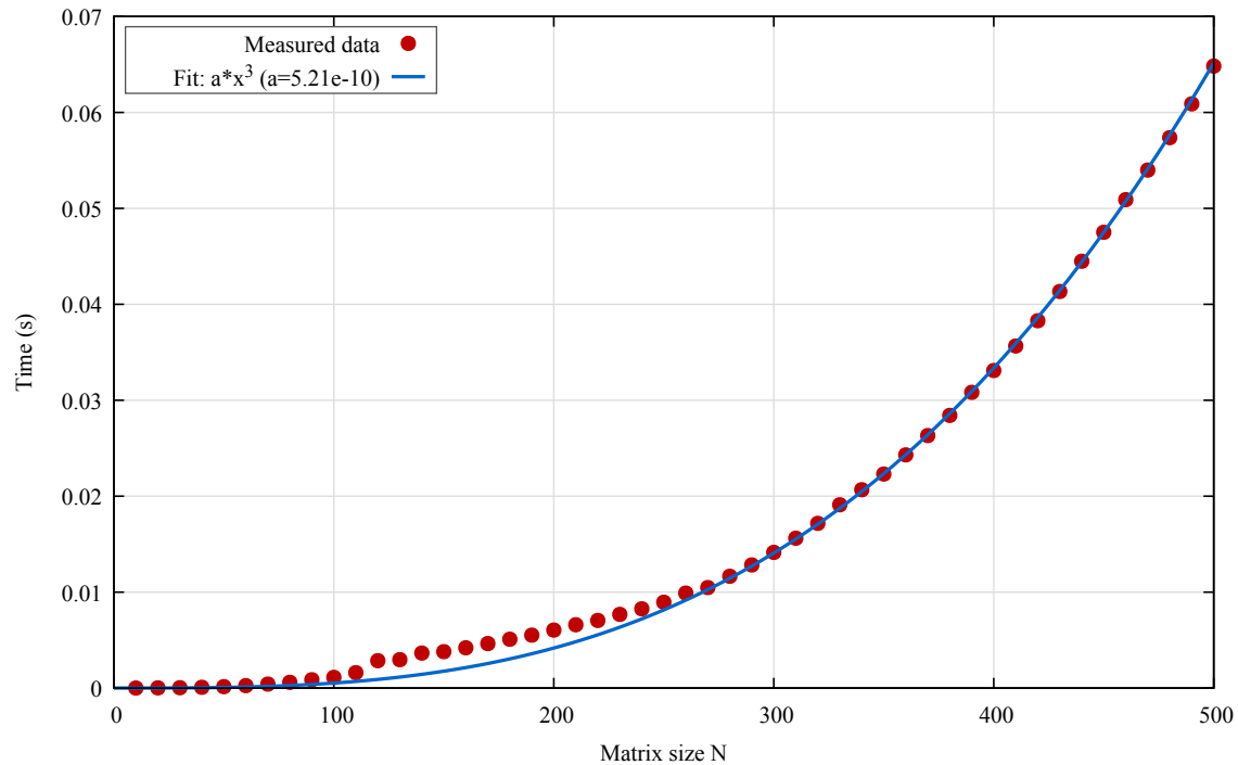
QR Decomposition Complexity
