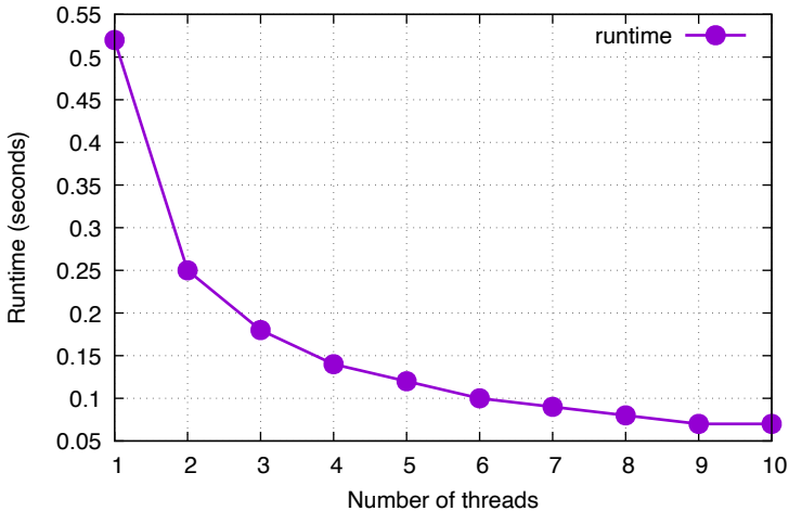
Runtime vs Threads for Harmonic Sum
