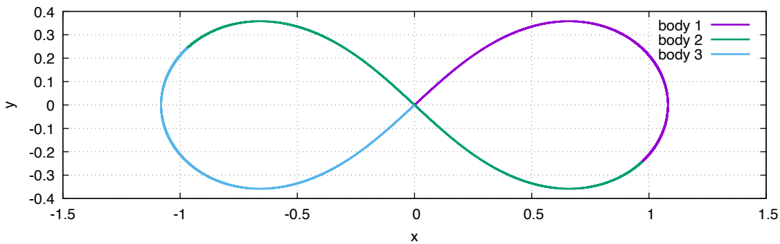
Three-Body Figure-8 Orbit
