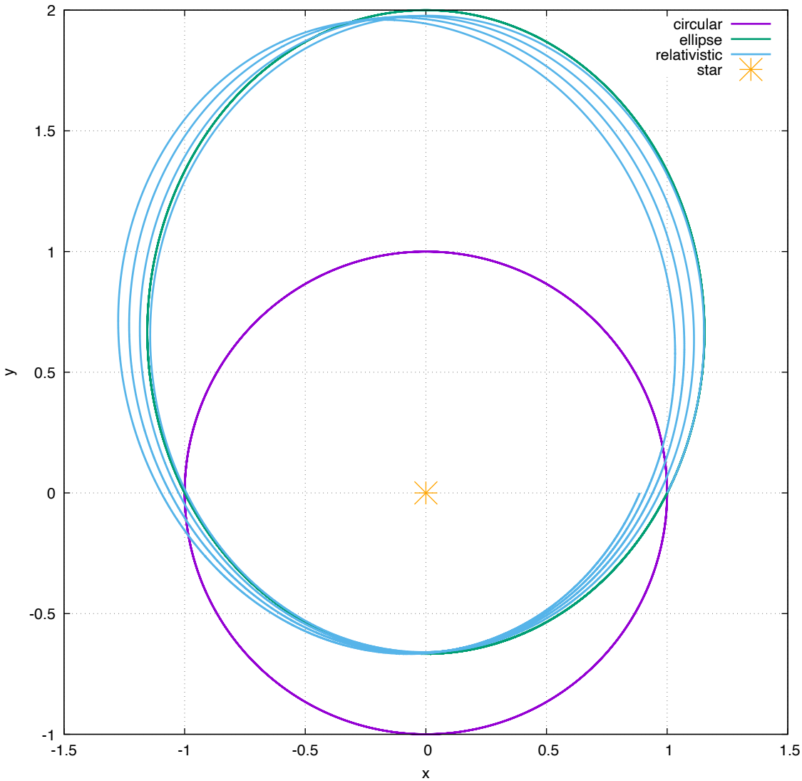
Relativistic Orbit (different \epsilon )
