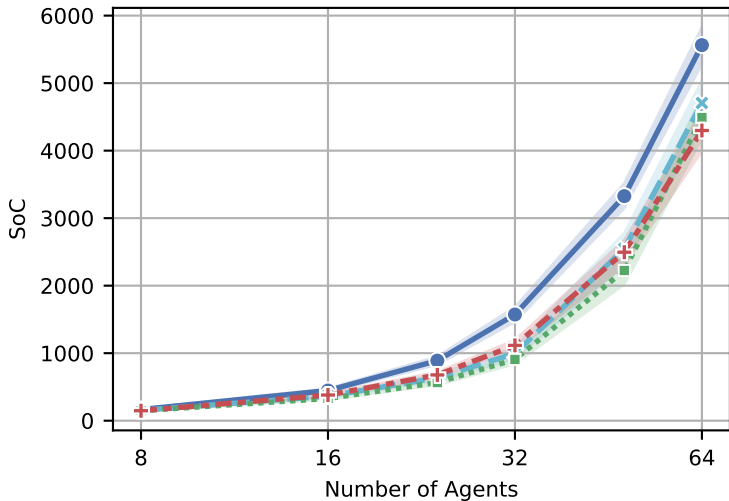
Mazes 20 × 20
