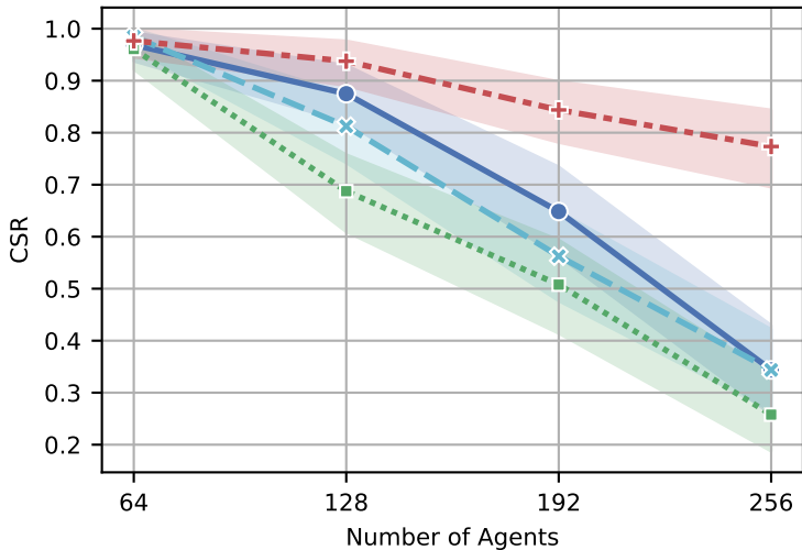
Out-of-Distribution
