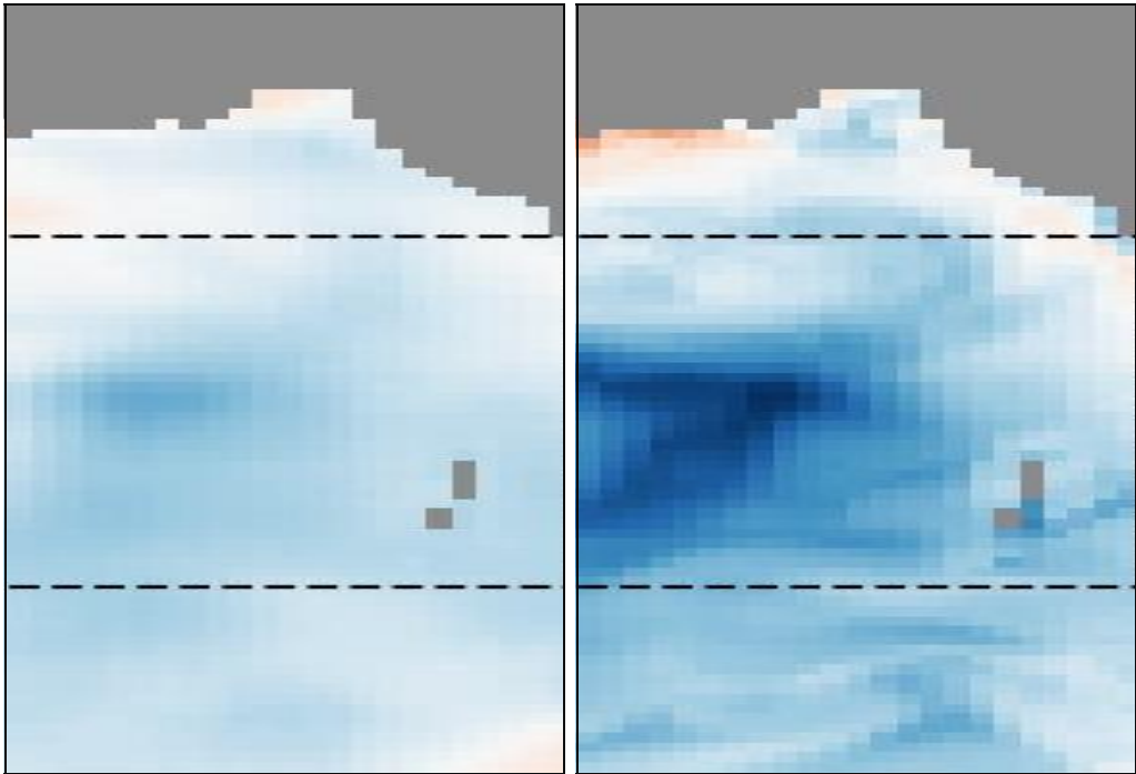
Satelight Cyclone Mocha, 2023-05-06 to 17: box-mean heat potential 93.6 → 80.0 kJ/cm 2 , satellites only.
