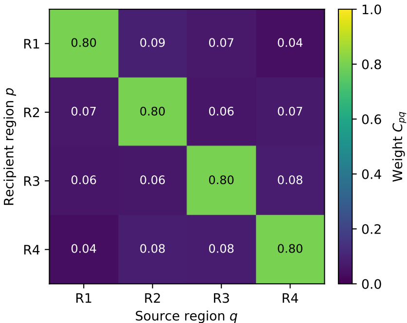
Compatible distance prior C_0 Regularization target, \lambda_C = 0.20
