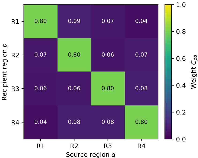
No regularization Distance initialization only, \lambda_C = 0
