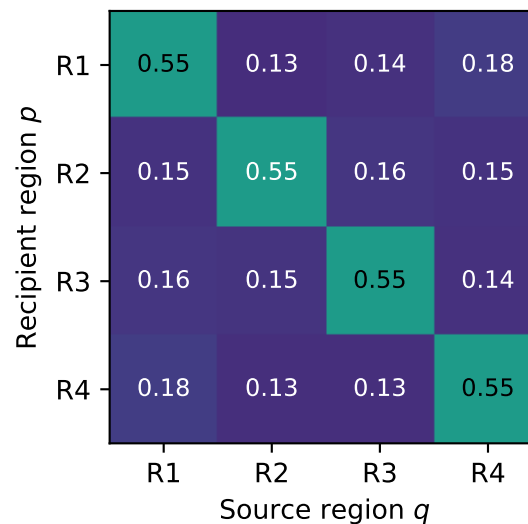
Strongly-wrong-prior estimate \hat{C} Matrix error 0.577 | Data loss 0.00396
