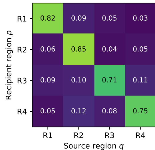
No-regularization estimate \hat{C} Matrix error 0.159 | Data loss 0.00331
