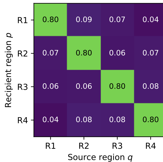
Compatible-prior estimate \hat{C} Matrix error 0.099 | Data loss 0.00323
