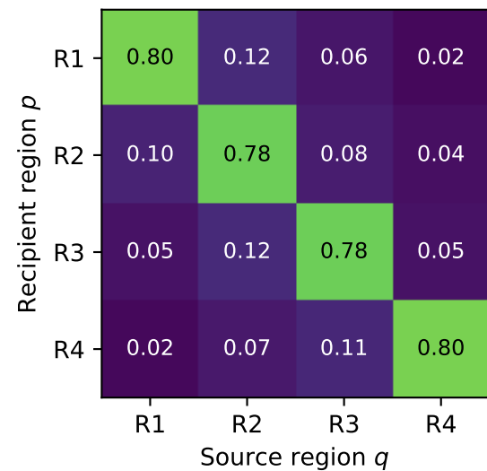
True C^* Ground truth
