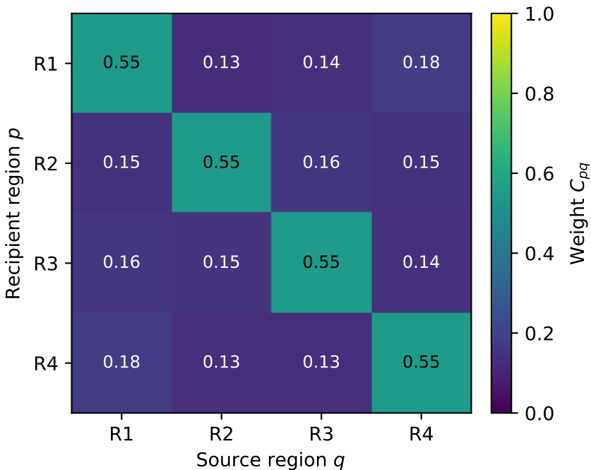
Strongly wrong prior C_0 Anti-distance target, \lambda_C = 1.00
