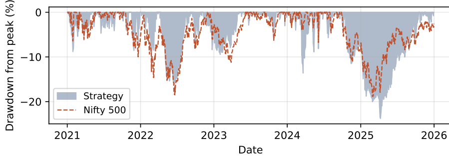
Figure 2: Drawdown from running peak, strategy vs. Nifty 500, 2021–2025. The strategy’s deeper trough in early 2025 is the -23.78\% Maximum Drawdown reported in Table 1; it recovers to a new high within the same year.
