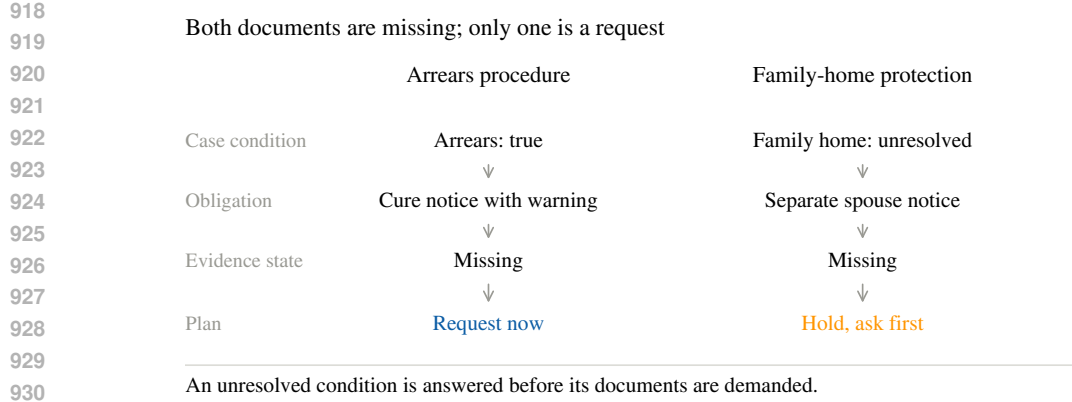
Figure 5: A recorded controller decision. The first completed CASEPATH development case in sorted cohort order has true arrears and unresolved family-home status. The controller requests the cure notice immediately and keeps the spouse notice conditional. These are two routes in the saved plan. The exported graph has the same predicate-interface failure as the other generated artefacts. The release provides the full trace and case selection rule.
