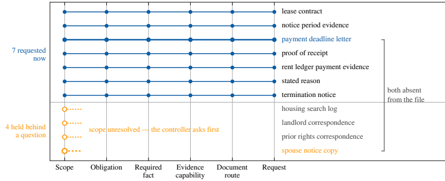
Figure 7: Where a chain stops. The first completed CASEPATH development case in sorted cohort order. Each row is one document the controller considered; the horizontal axis is the chain of Equation 1. A chain that reaches a request has an obligation whose scope resolved true, and records its own fact, capability and route. The remaining chains stop at an unresolved scope, and the controller asks rather than demands. The cure notice and the spouse notice are both absent from the file, and only one of them is a request: absence is not a reason, and the chain is where the difference is decided. The exported graph has the same predicate-interface failure as the other generated artefacts. The release provides the full trace and case selection rule.
