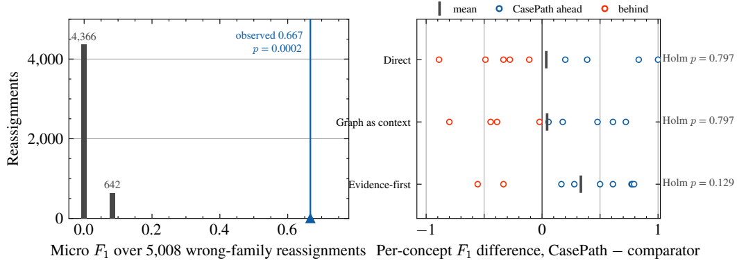
Figure 6: What the result survives, and what it does not. Left: CASEPATH’s held-out outputs are held fixed and reassigned to the wrong branch family. The entire null mass lies at or below one twelfth, while the correct assignment scores 0.667; the outputs therefore carry branch-specific content rather than a single checklist that fits any branch. Right: the preregistered family-swap contrast. Concepts fall on both sides of zero for every comparator and no Holm-adjusted test reaches significance, which is why this paper claims selectivity and traceability rather than statistical dominance.
