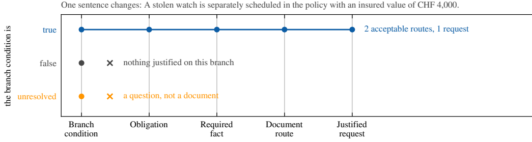
Figure 1: The three states a branch condition can take, on one benchmark intervention. The pair differs by the sentence quoted above. When the condition holds, the reference contract activates one obligation whose fact either of two document routes can establish, so one request is justified. When it is false, nothing on this branch is. When the sources leave it unresolved, the chain stops and CASEPATH asks. Section 2 defines each version’s route-selection and sufficiency rules.
