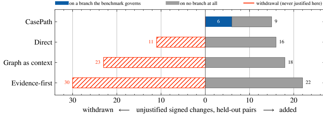
Figure 4: The unjustified changes differ in kind, not only in count. Every unjustified signed change made by the three comparators moves a document that no branch in this benchmark governs. CASEPATH makes 9 such changes rather than 27, 41 or 52, and six of its fifteen fall on a governed branch. Governed means the document appears in some unit’s reference branch set or in an acceptable signed change; it does not mean the remainder are documents every claim needs, which this benchmark cannot test.
