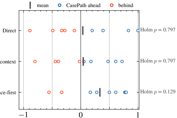
Per-concept F_1 difference, CasePath - comparator
