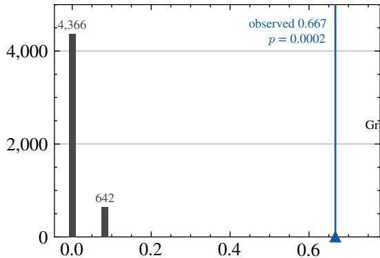
Micro F_1 over 5,008 wrong-family reassignments
