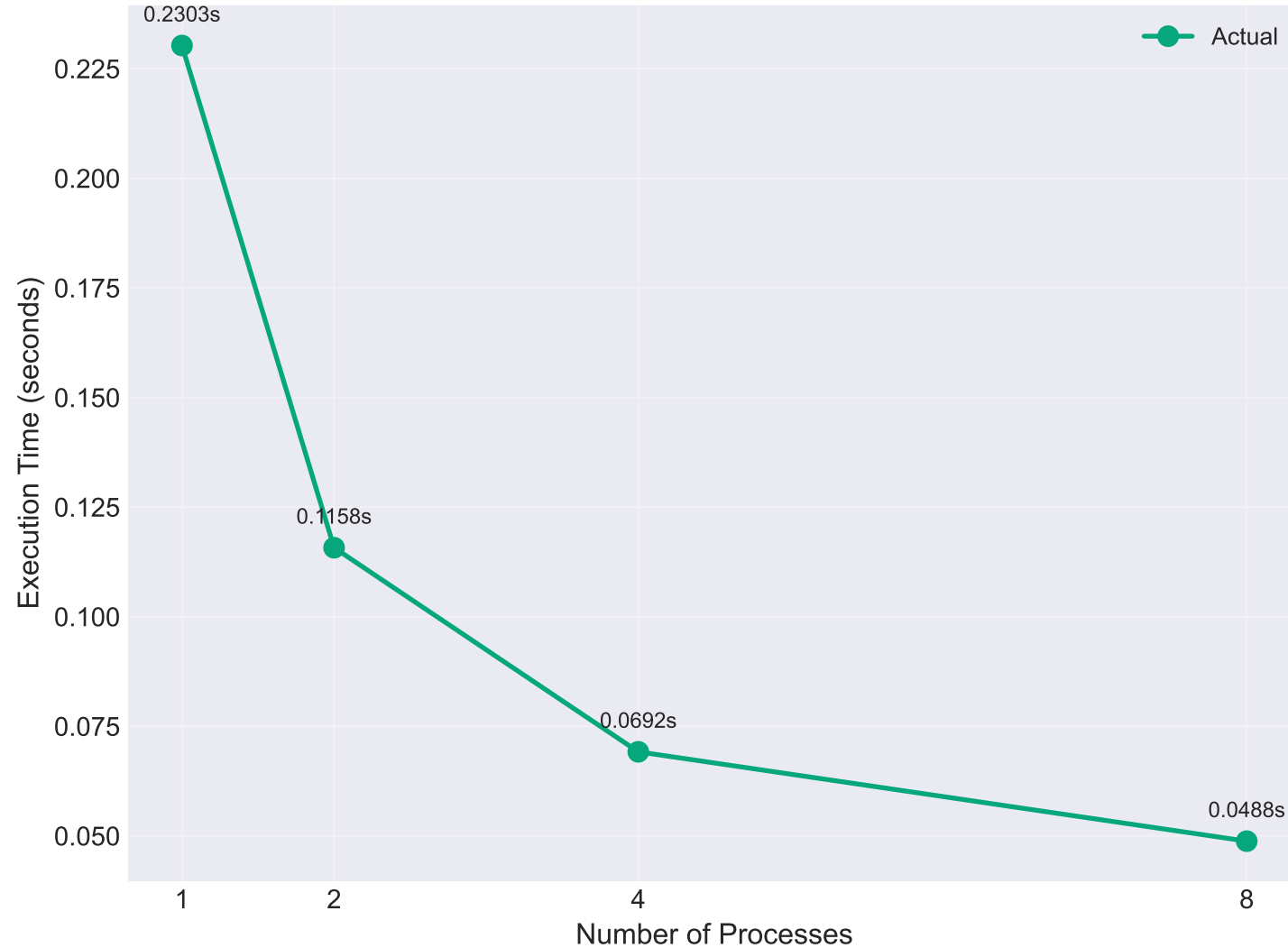
MPI: Processes vs Execution Time (N=1024)
