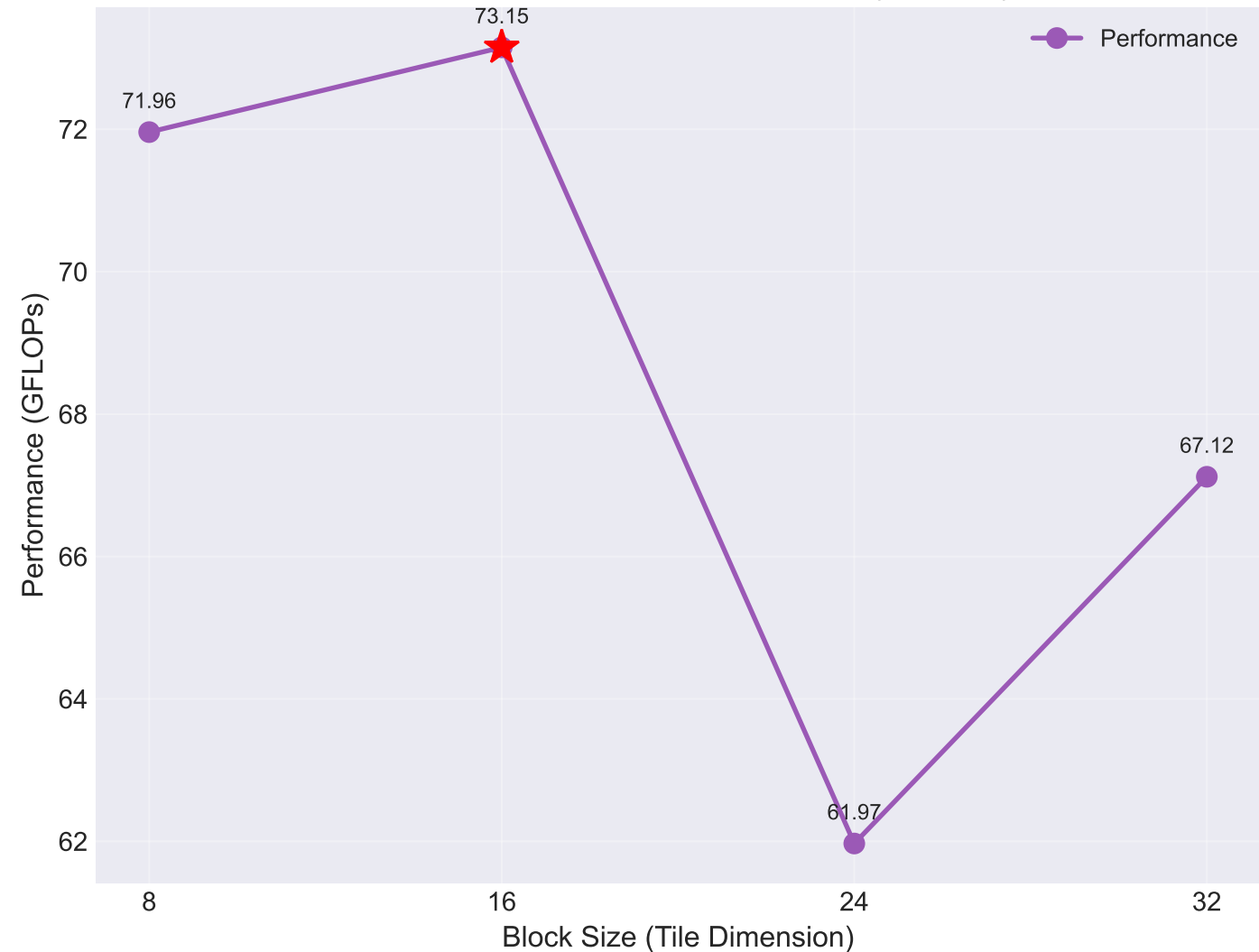
CUDA: Block Size vs Performance (N=1024)
