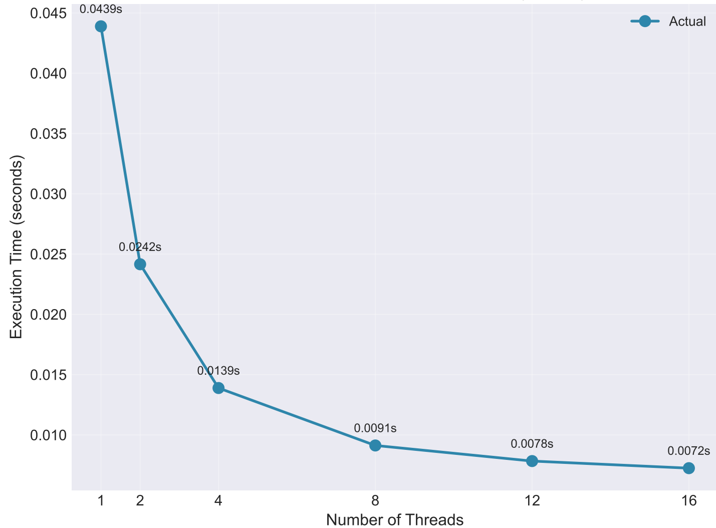
OpenMP: Threads vs Execution Time (N=512)
