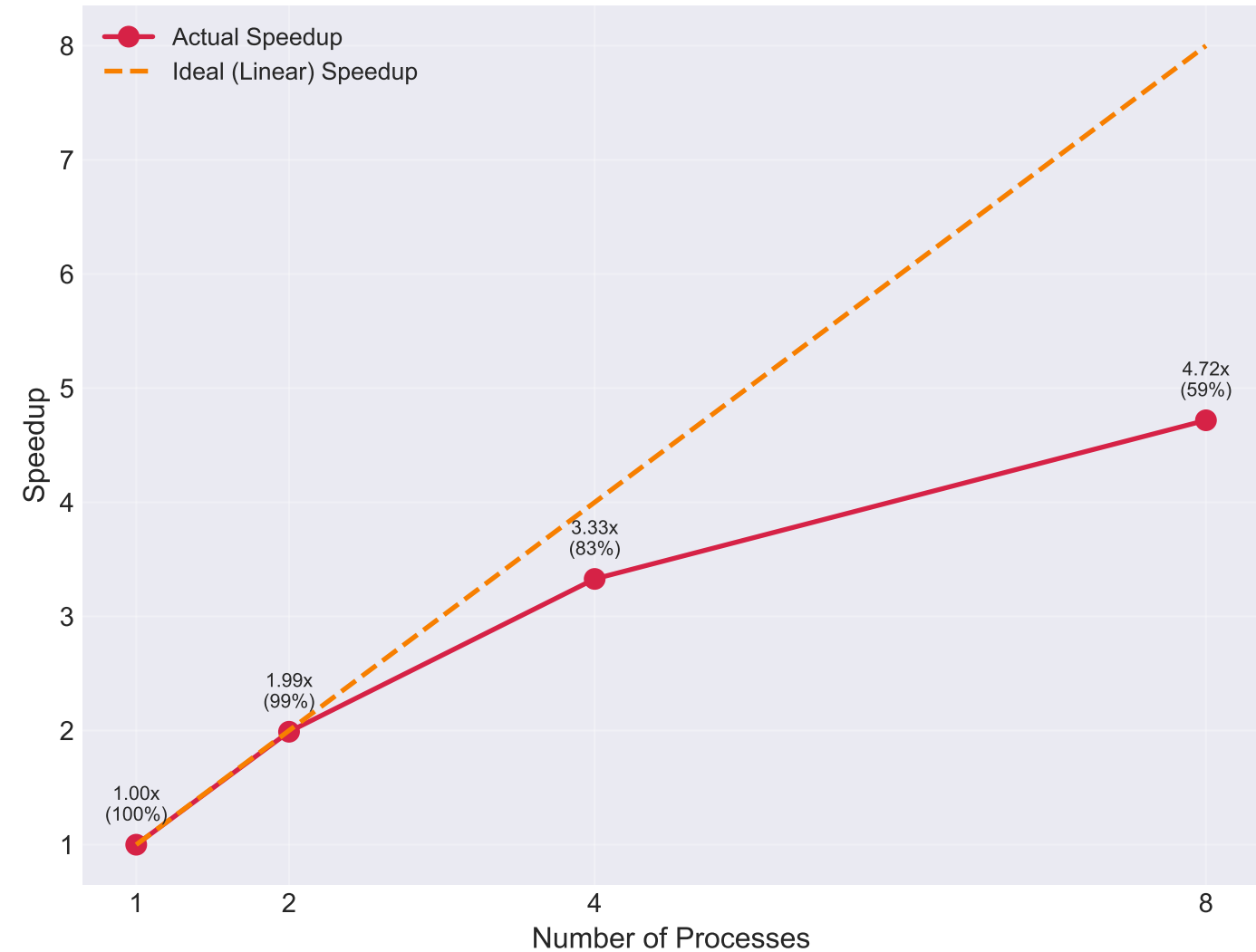
MPI: Processes vs Speedup (N=1024)
