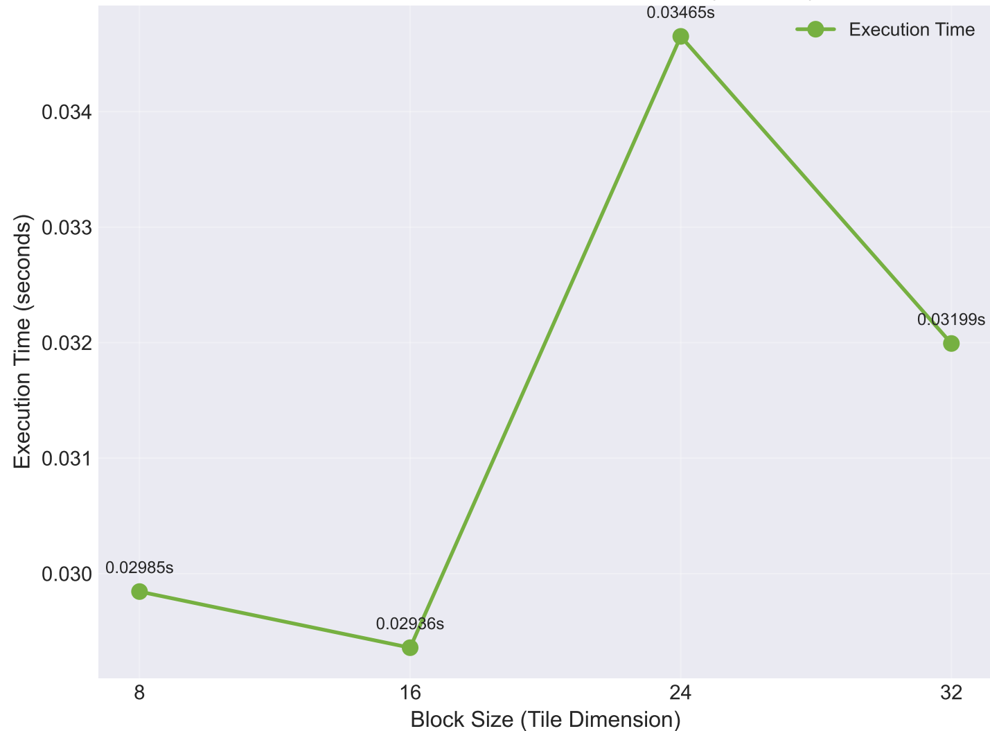
CUDA: Block Size vs Execution Time (N=1024)
