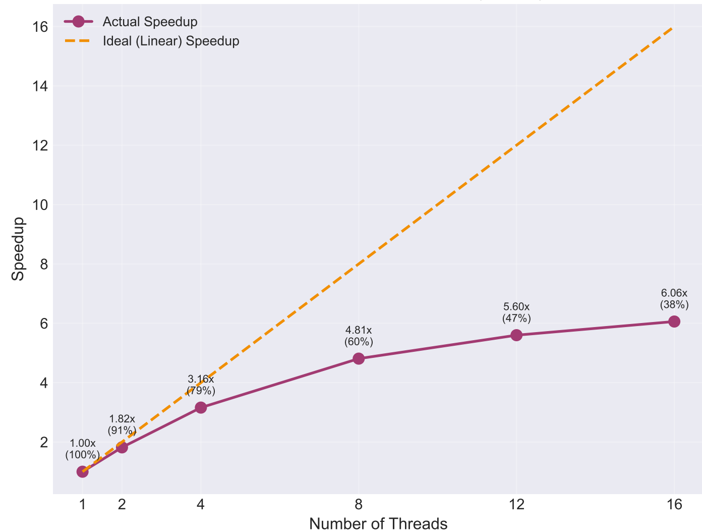
OpenMP: Threads vs Speedup (N=512)
