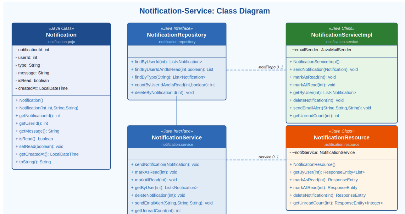
Figure 7: Notification-Service — Class Diagram
