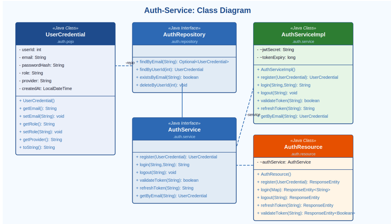
Figure 2: Auth-Service — Class Diagram
