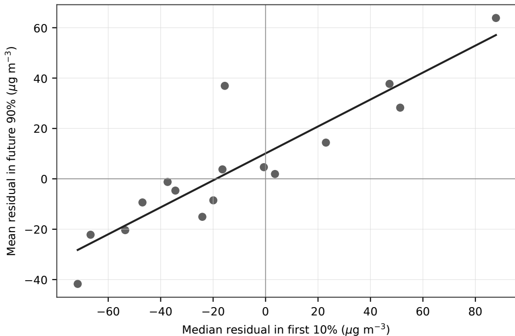
Early bias predicts later bias ( r=0.90 )
