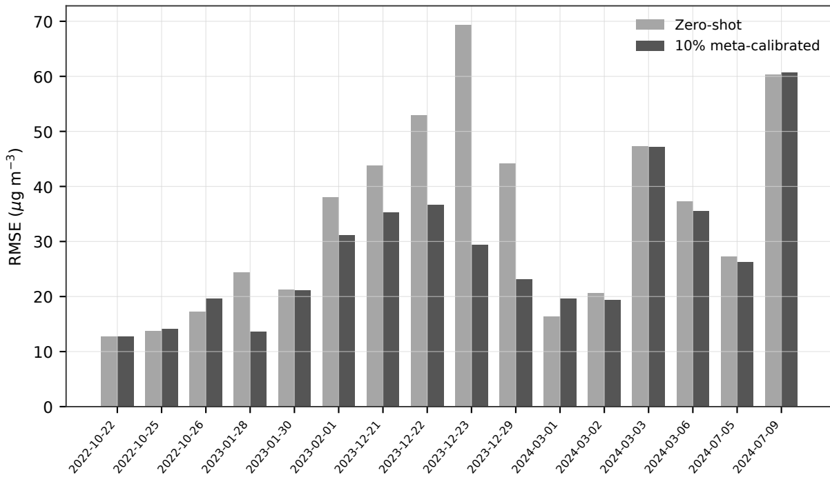
Matched future-90% error by held-out date
