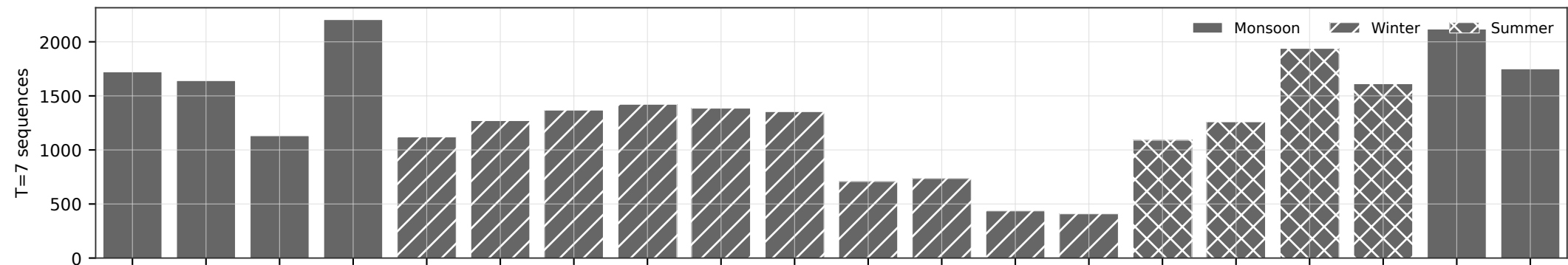
TRAQID coverage across 20 complete collection dates
