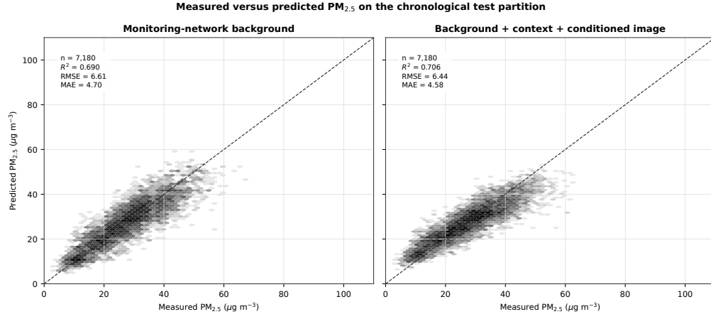
Figure 5: Measured versus predicted Taiwan PM_{2.5} on the chronological 54-date test period. Both panels use identical 7,180 sequences and axes. The conditioned model reduces aggregate error but still underestimates sparse high-concentration observations.
