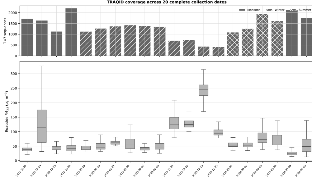
Figure 1: TRAQID date coverage and roadside PM 2.5 distributions. Shading denotes the season labels used in the campaign-level analysis. Box plots omit fliers for legibility but all values are retained in modelling.
