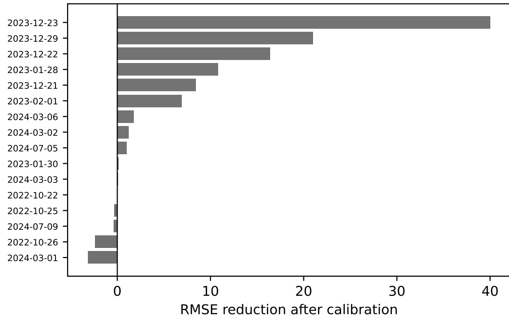
Date-level calibration effect
