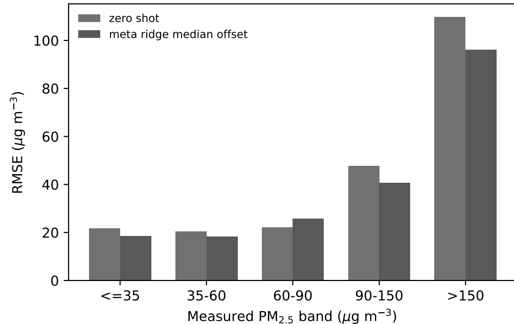
Error by concentration
