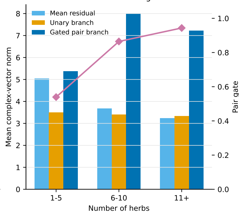
b Learned branch magnitudes
