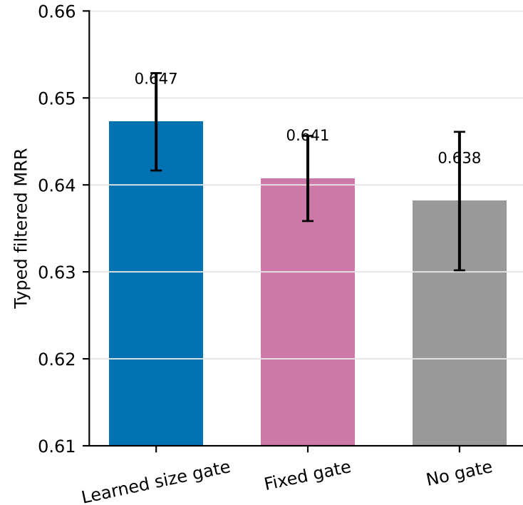
a Gate ablation
