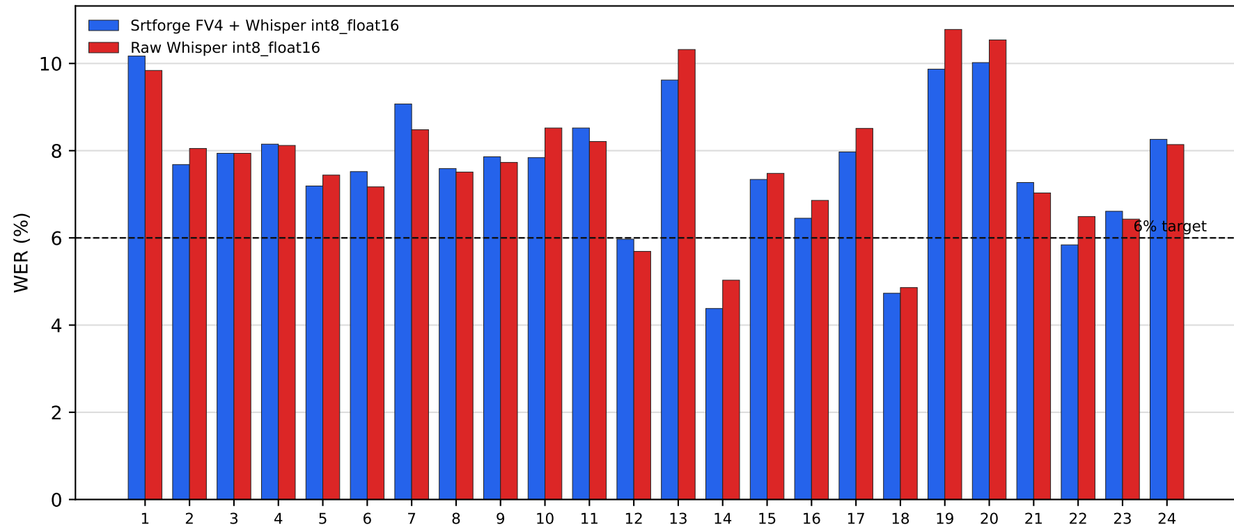
Season-scale WER by episode
