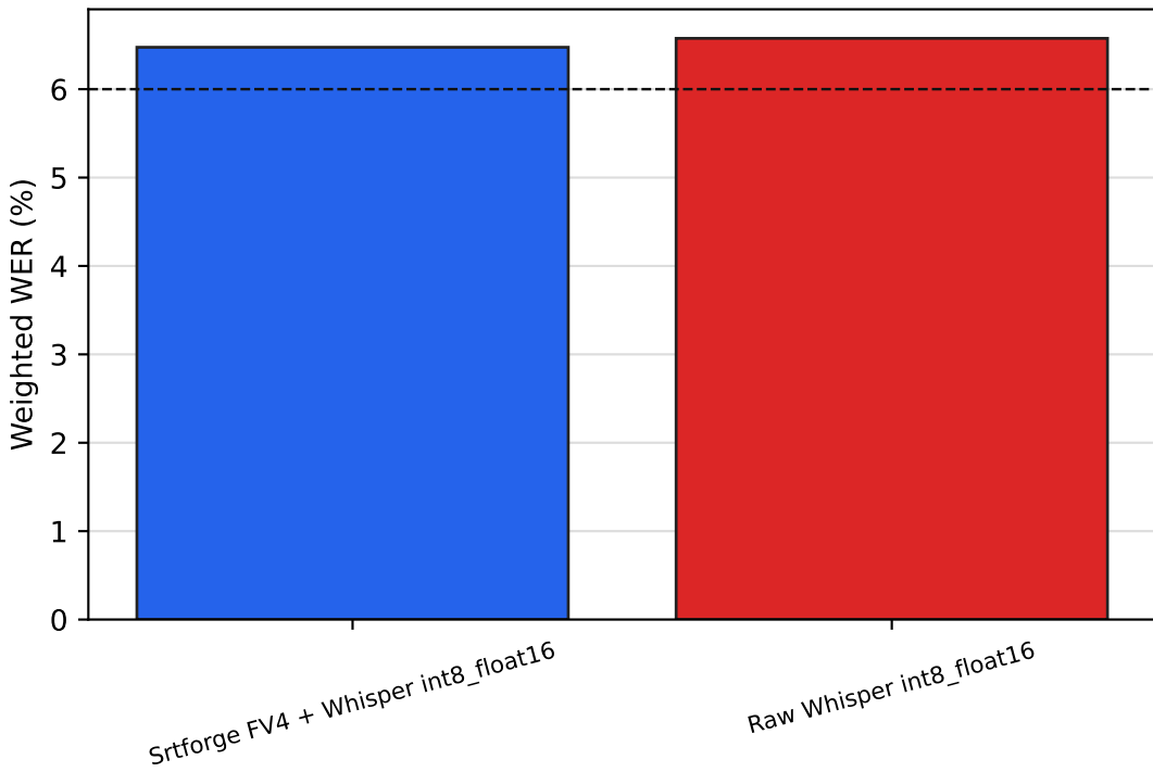
Steins;Gate S01 conservative assisted-truth summary
