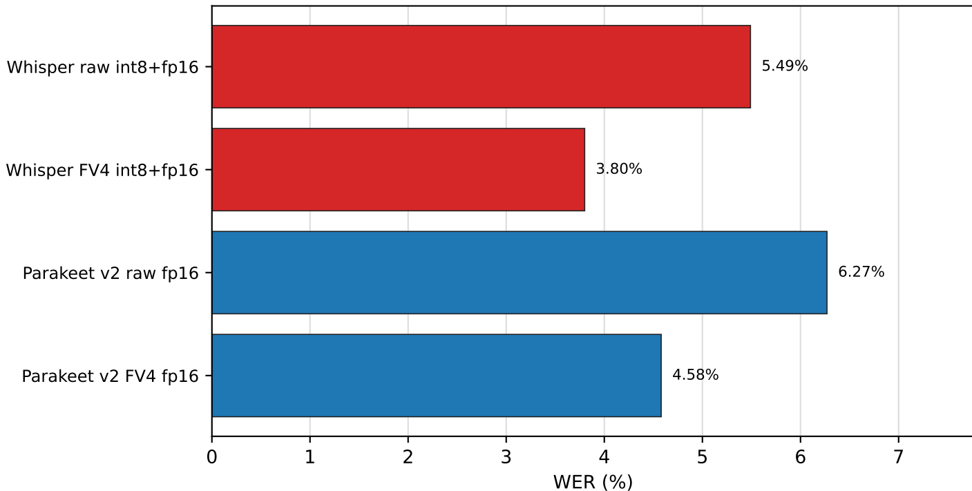
Reference media asset (M-1) WER by pipeline variant
