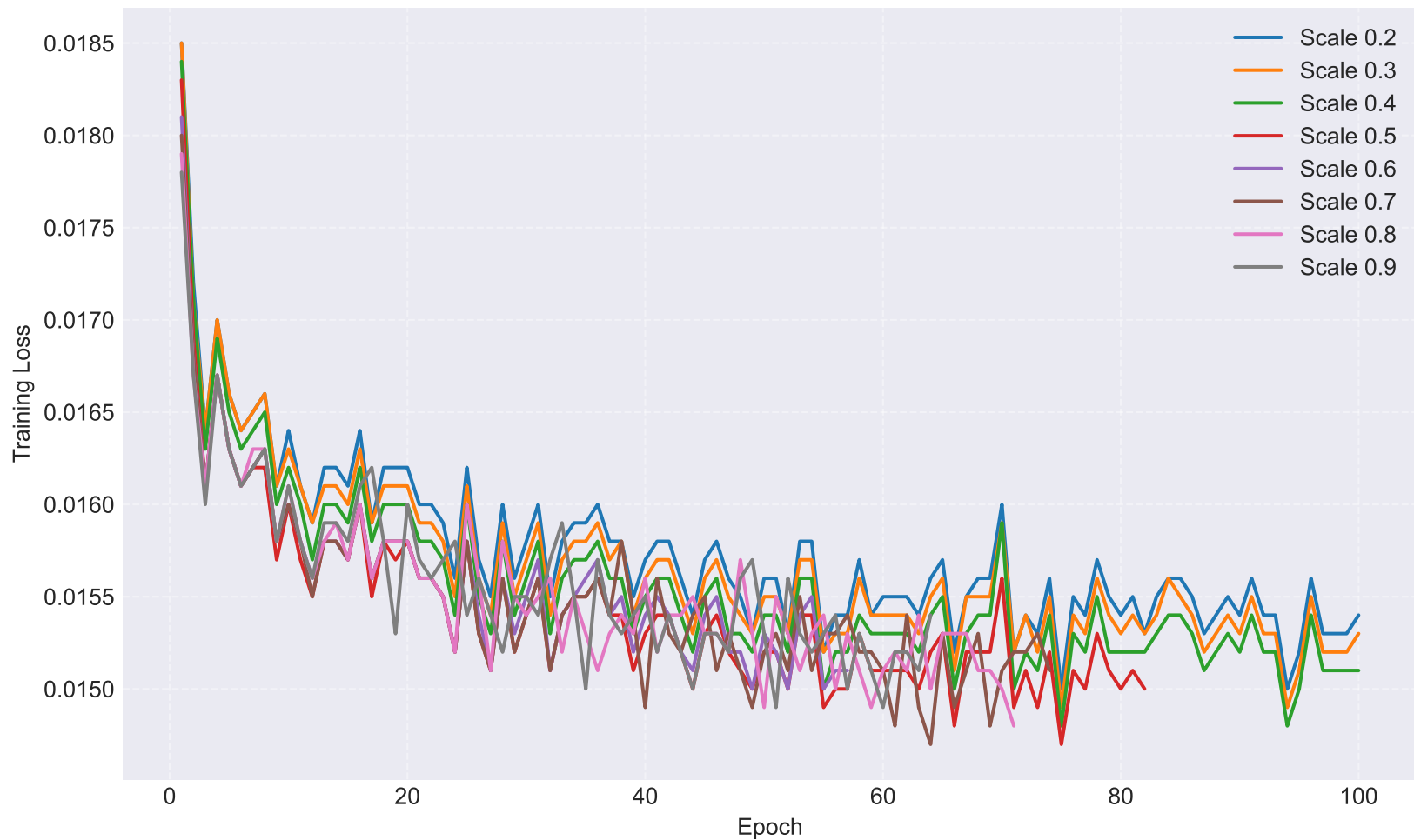
Training Loss vs Epoch (Experiment 1)
