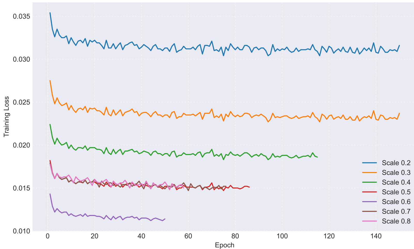
Training Loss vs Epoch (Experiment 2)
