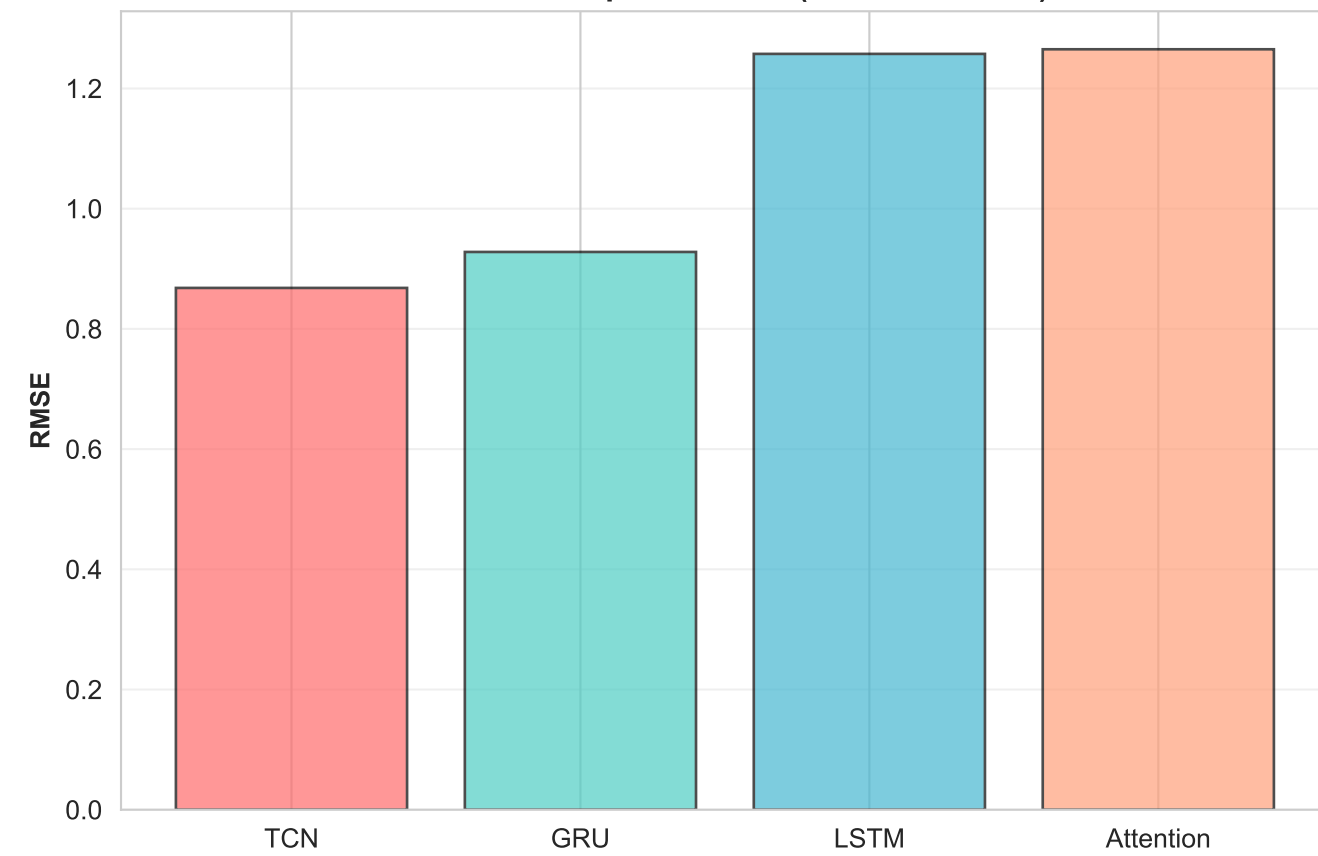
Root Mean Squared Error (Lower is Better)
