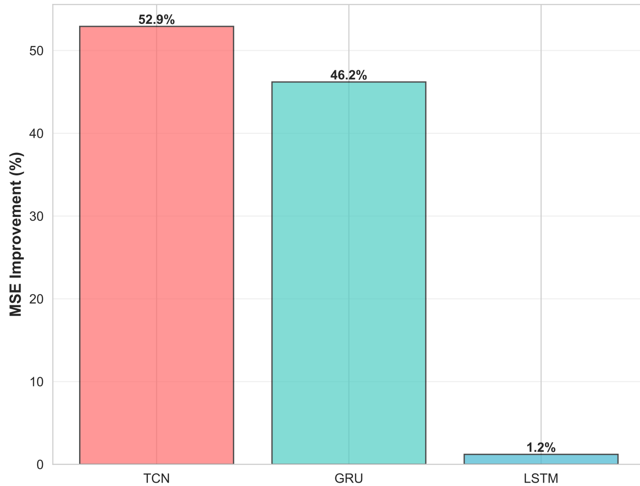
MSE Improvement vs Attention Baseline
