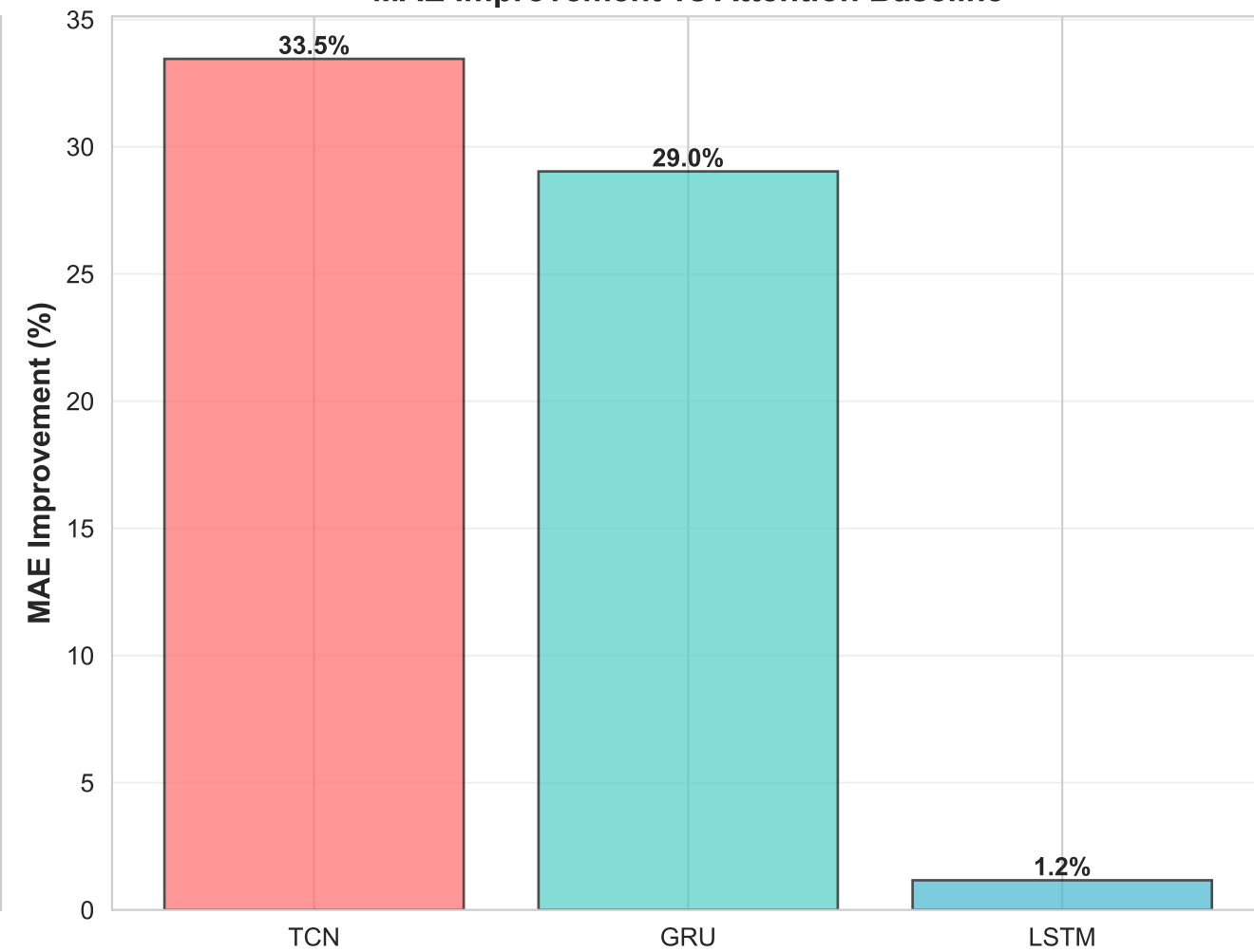
MAE Improvement vs Attention Baseline
