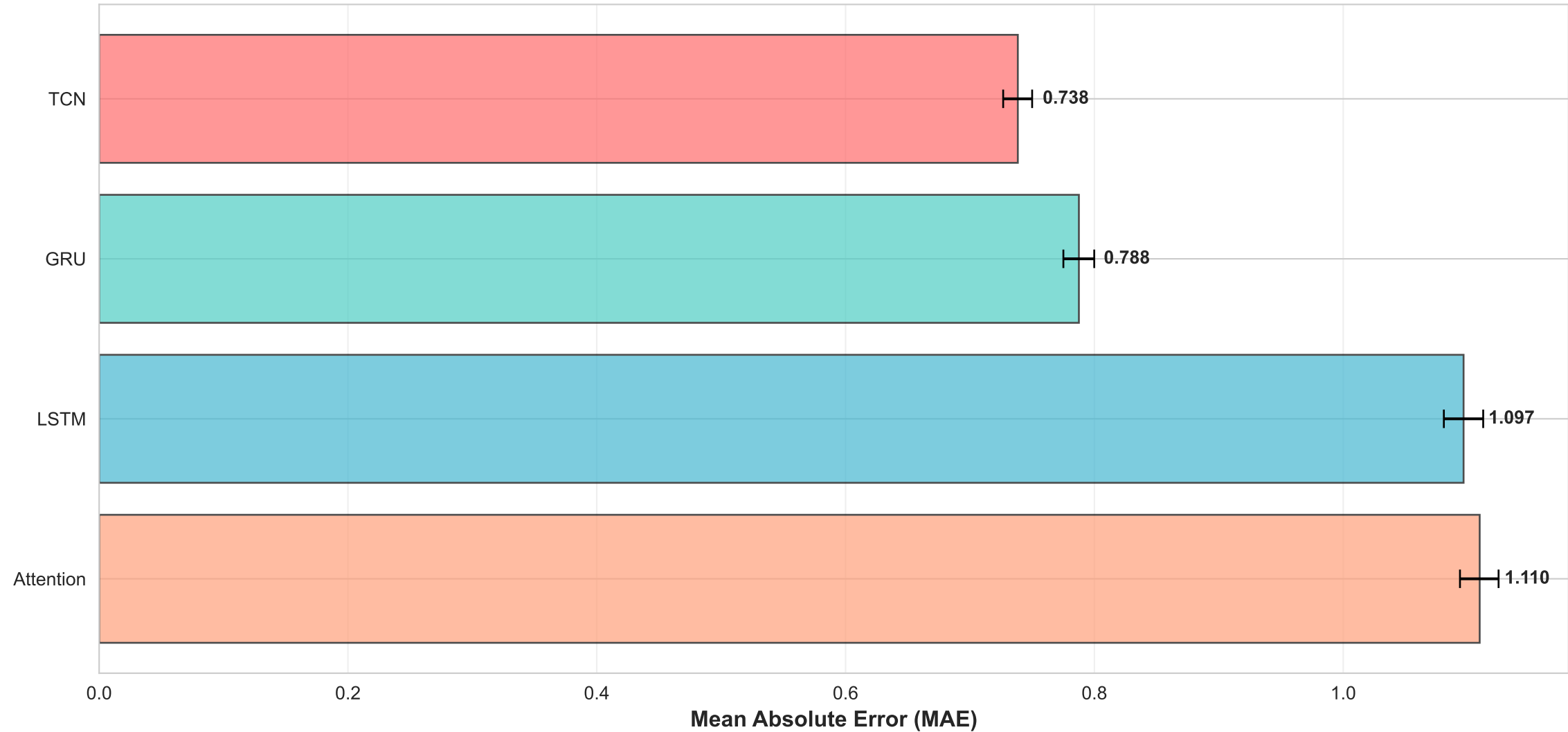
Model Ranking by MAE with 95% Confidence Intervals
