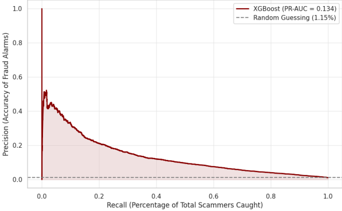
Precision-Recall Curve (Fraud Detection)
