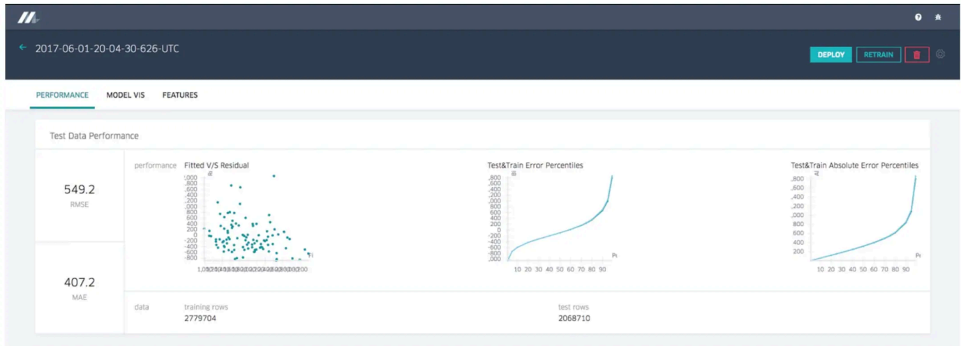
Figure 4: Regression model reports show regression-related performance metrics.
