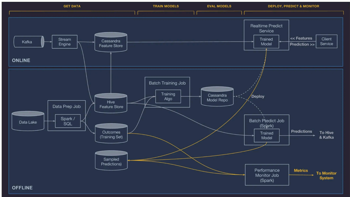
Figure 10: Predictions are sampled and compared to observed outcomes to generate model accuracy metrics.
