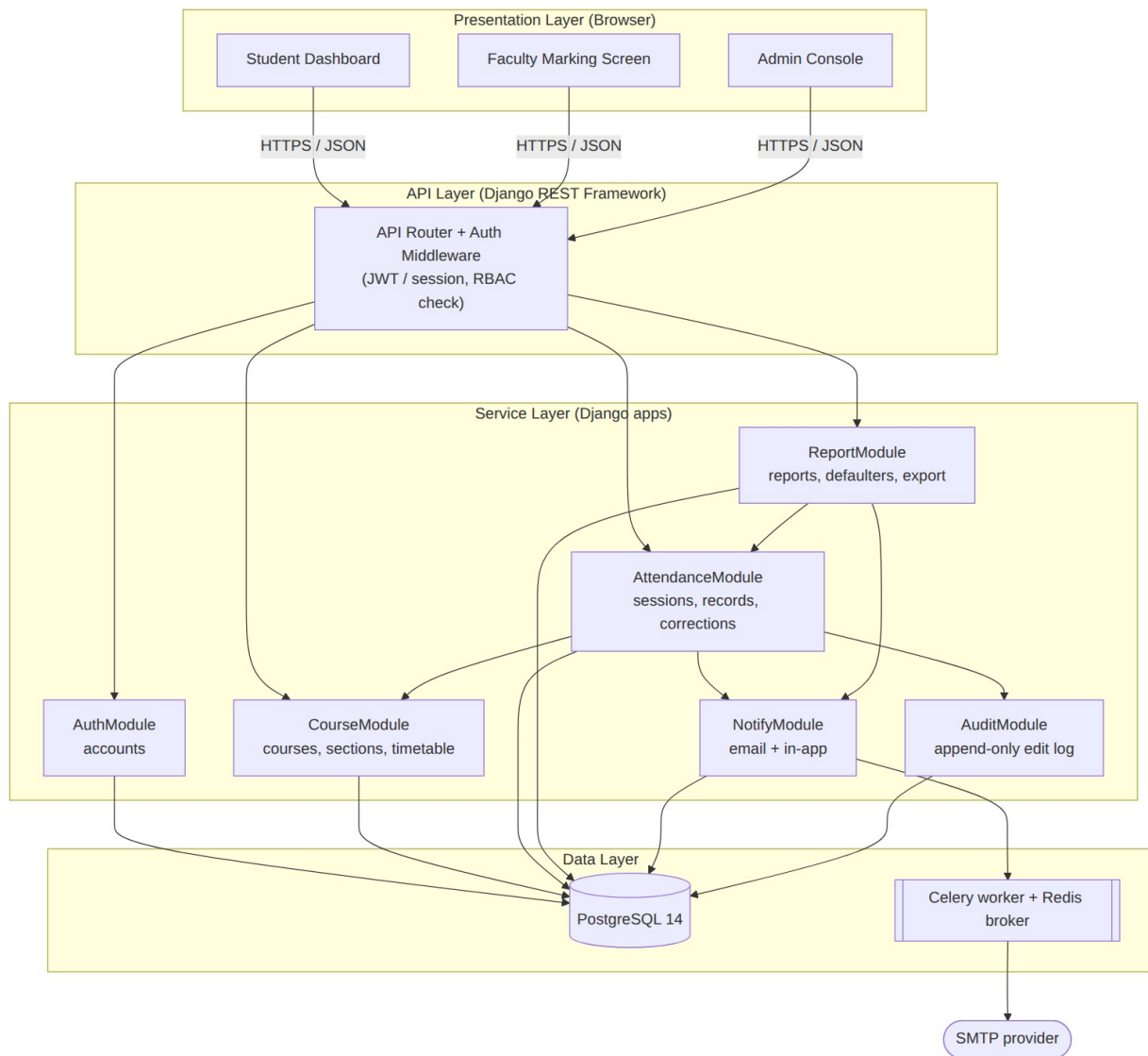
Figure 1: SAMS component diagram (layered)
