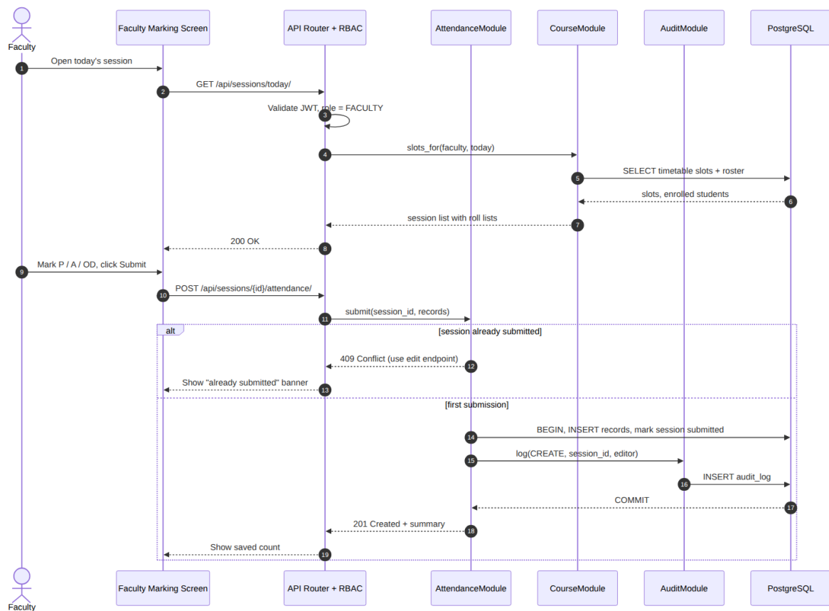
Figure 5: Mark attendance
