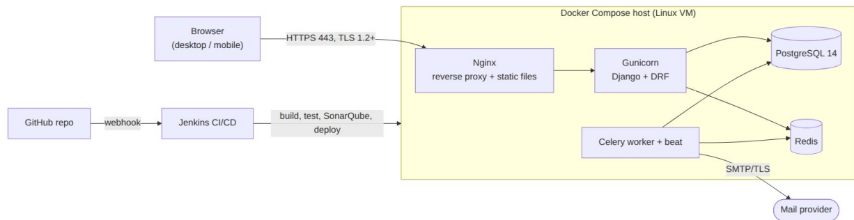
Figure 3: Deployment diagram
