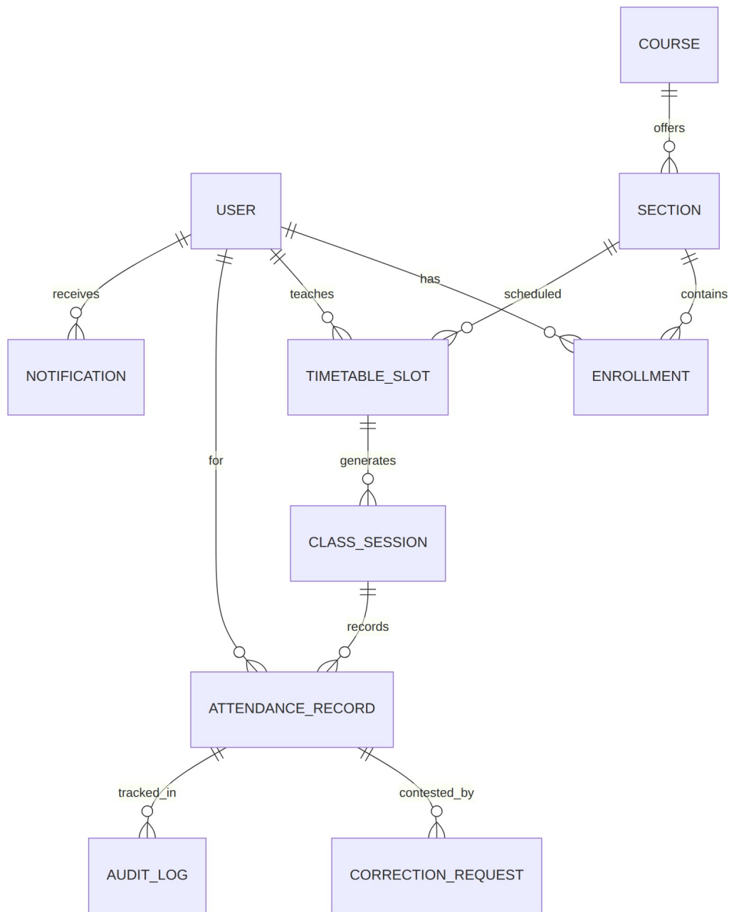
Figure 4: Entity-relationship diagram
