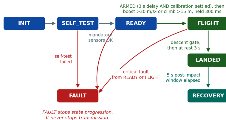
Mission state machine — every transition and the guard on it
