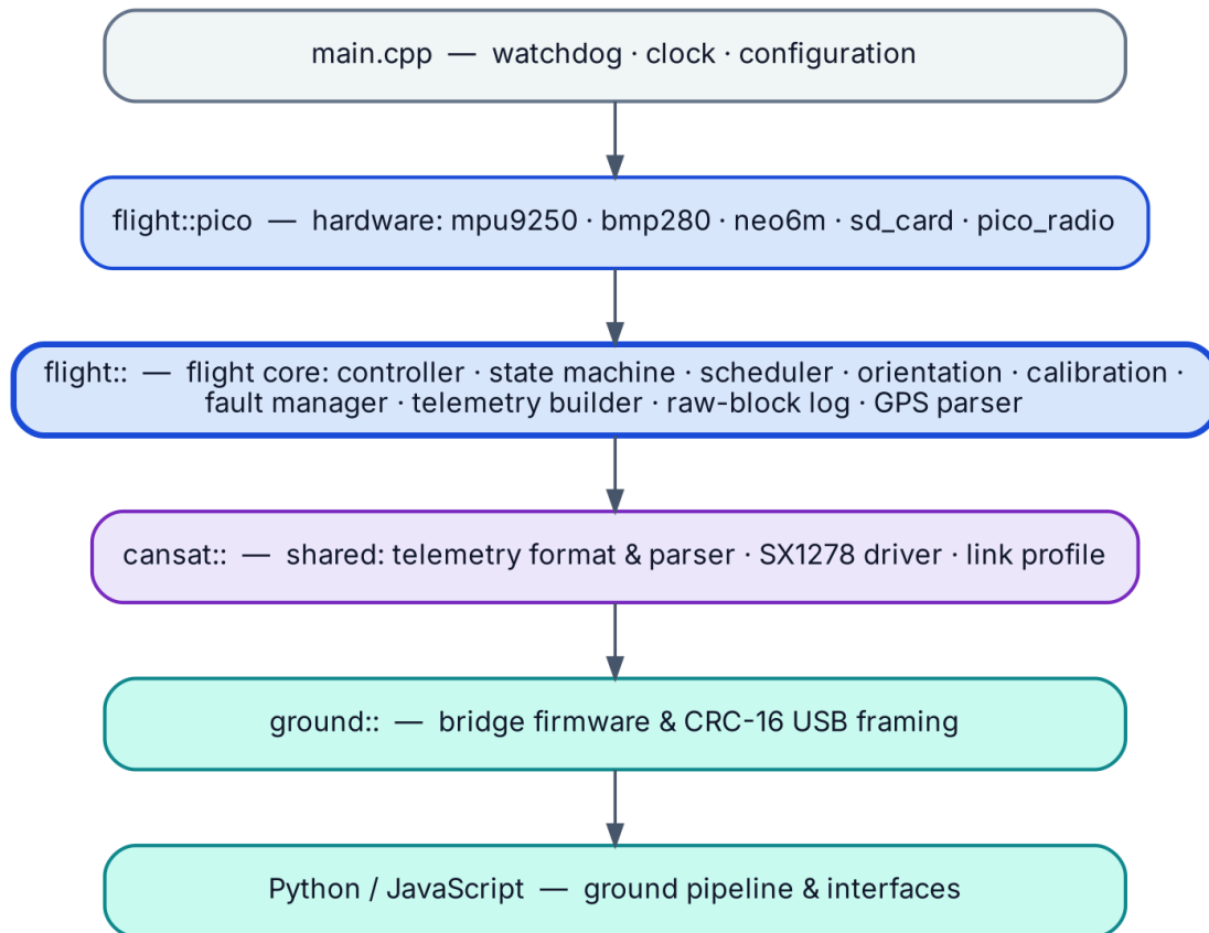
Figure 8 · Each layer depends only on the layer beneath it. The flight core (bold) is hardware-free.
