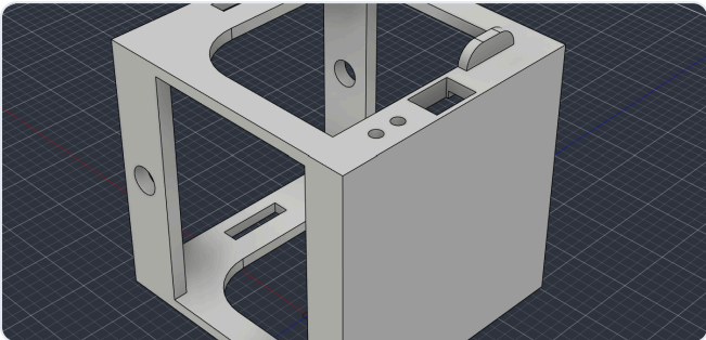
Render, three-quarter view from above: switch cut-out and two LED holes on the upper face.
