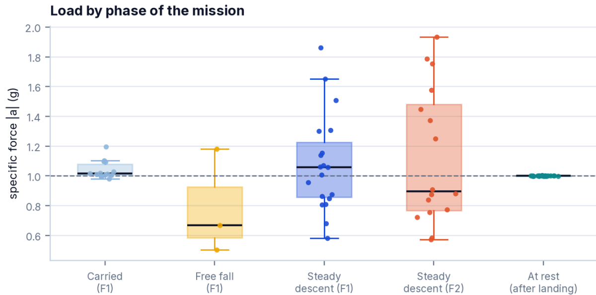
Figure 37 · The load on the vehicle by phase of the mission, in units of g: carried, free fall, steady descent (both flights) and at rest after landing. The resting value (1.000 g, \sigma 0.0015 g) is the accelerometer's calibration made visible.
