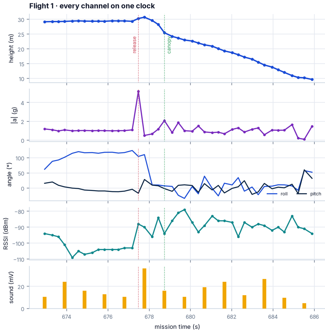
Figure 33 · Flight 1 on one clock. Height, specific force, roll and pitch, RSSI and acoustic level — release and canopy opening marked. The same instant shows up in every channel: the acceleration spike, the roll swinging from 110° (on its side) to upright, the radio signal improving by 14 dB, and the loudest microphone packet.
