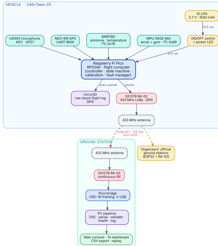
Figure 1 · The whole system: the vehicle, the radio link, and the team's ground station beside the organizers' official stations.
