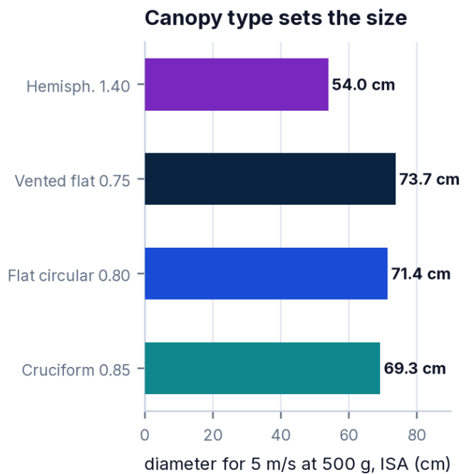
Figure 16 · Left: terminal descent rate against flat canopy diameter for the three masses of the band, on a standard day (solid) and a 35 °C day (dashed); the design floor is 80 cm. Right: the diameter needed for 5 m/s at 500 g for each canopy type.
