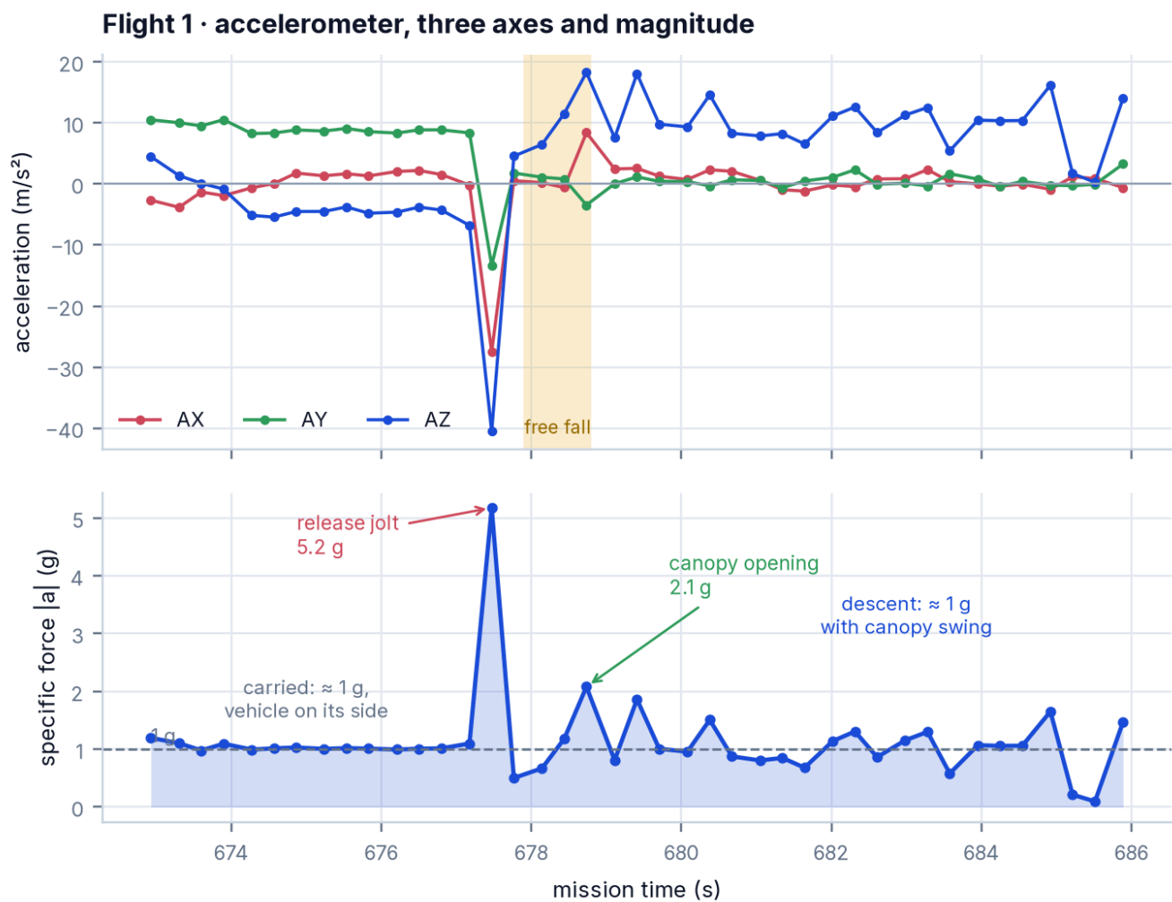
Figure 32 · Flight 1 — acceleration. The release jolt (5.2 g), the free-fall dip below 1 g, the canopy-opening load (2.1 g) and the descent at about 1 g with canopy swing.
