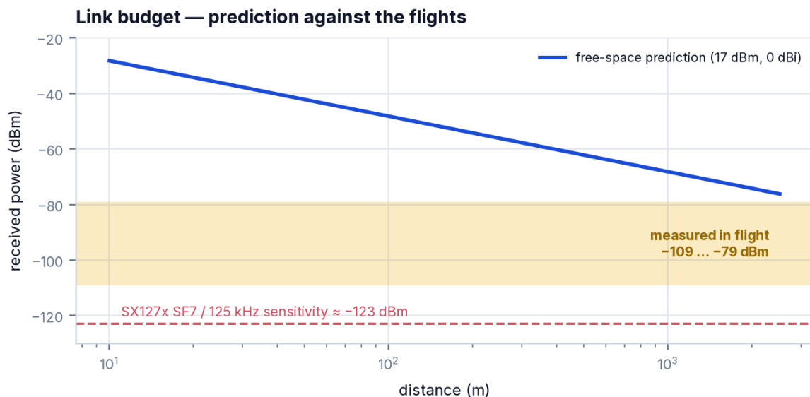
Figure 24 · Free-space prediction (17 dBm, 0 dBi antennas) with the receiver floor, and the band of RSSI the organizers' station actually recorded in flight.
