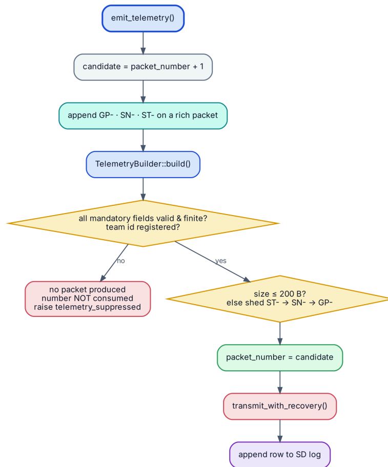
Figure 5 · The path from a snapshot to a packet. Nothing is built if any mandatory field is invalid, and the packet number is consumed only when a packet is actually produced.
