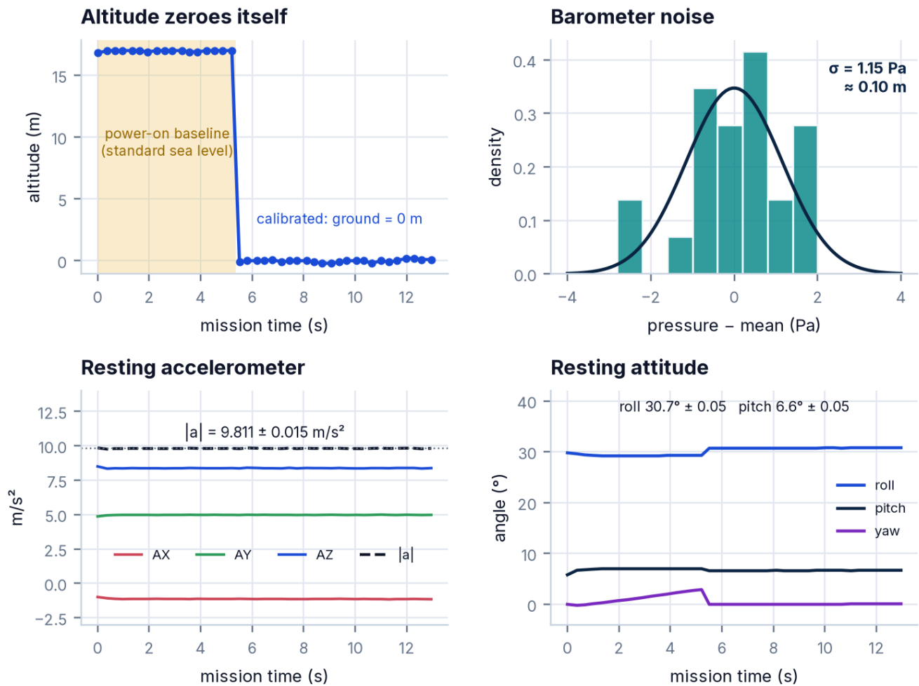
Figure 47 · The after-landing session. Top left: altitude zeroes itself at 5.5 s. Top right: barometer noise at rest. Bottom left: resting accelerometer. Bottom right: resting attitude.
