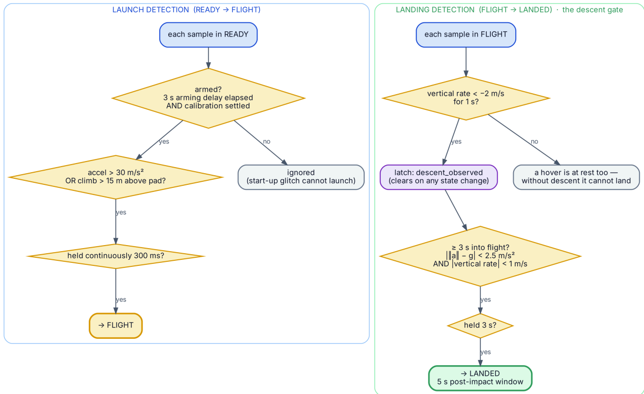
Figure 7 · Launch detection (left) and landing detection with the descent gate (right).
