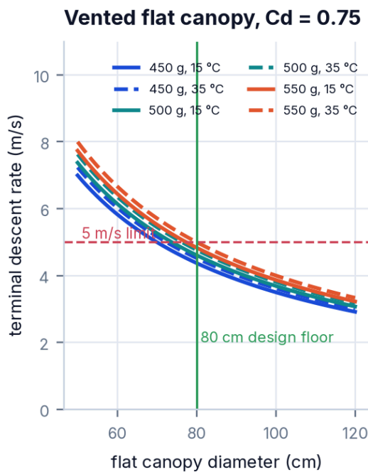
Figure 16 · Left: terminal descent rate against flat canopy diameter for the three masses of the band, on a standard day (solid) and a 35 °C day (dashed); the design floor is 80 cm. Right: the diameter needed for 5 m/s at 500 g for each canopy type.
