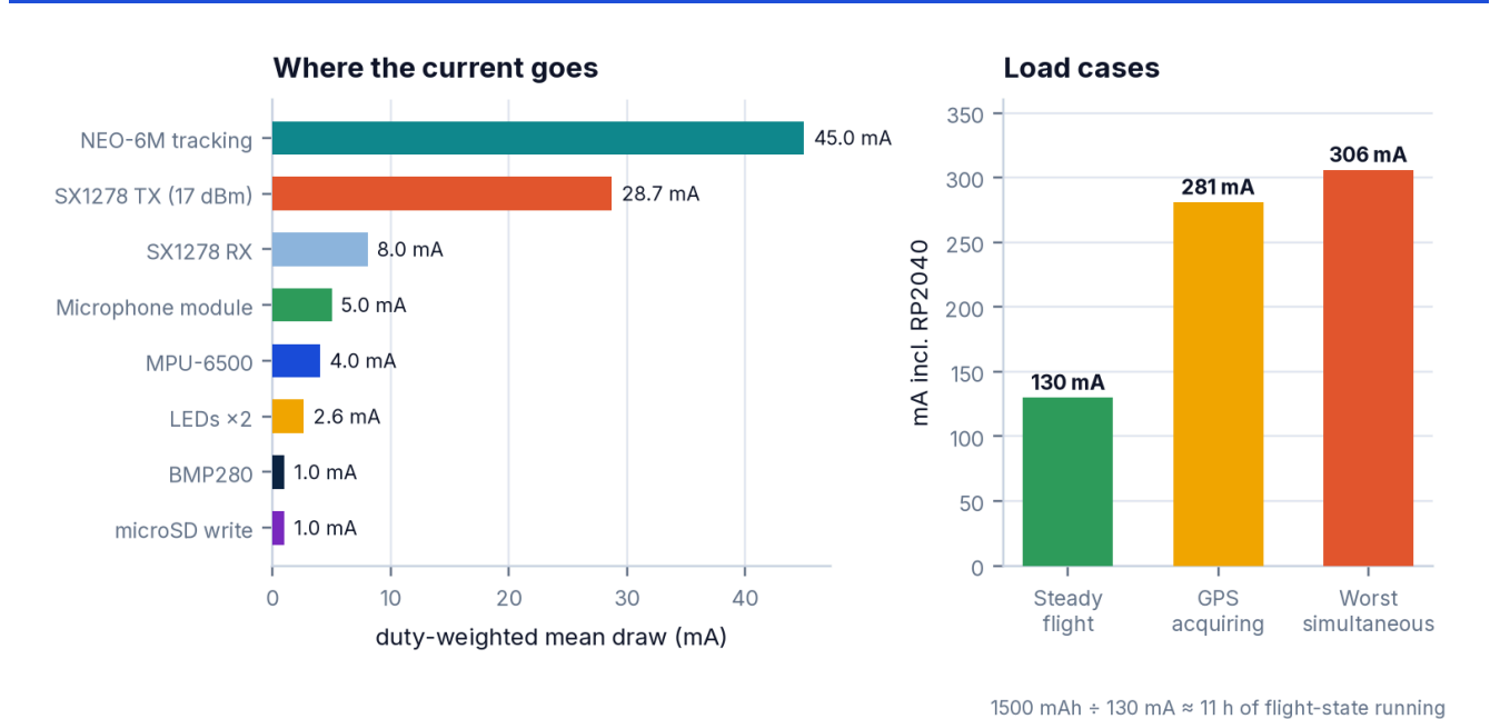
Figure 11 · Duty-weighted current by device (left) and the three load cases (right).
