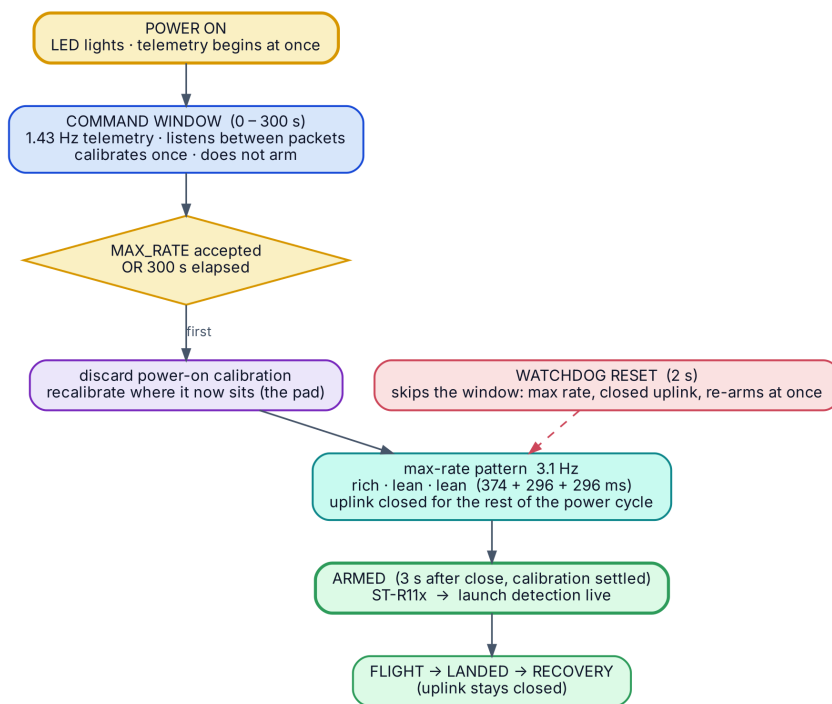
Figure 6 · The power-on sequence. The watchdog path skips the window: a reset may come mid-flight, and five minutes unarmed and listening would be five minutes without launch or landing detection.
