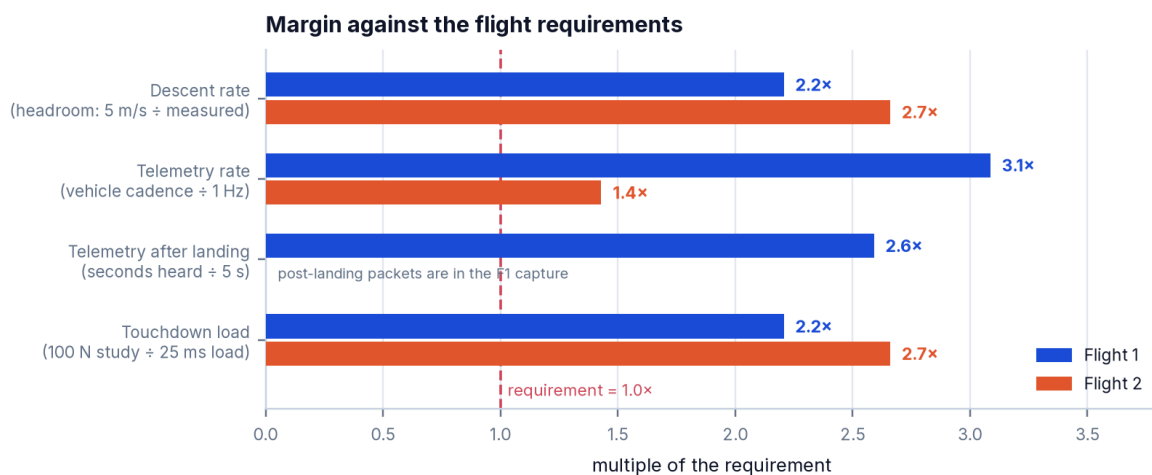
Figure 3 · Each measured quantity as a multiple of the requirement it answers. 1.0 is the requirement.
