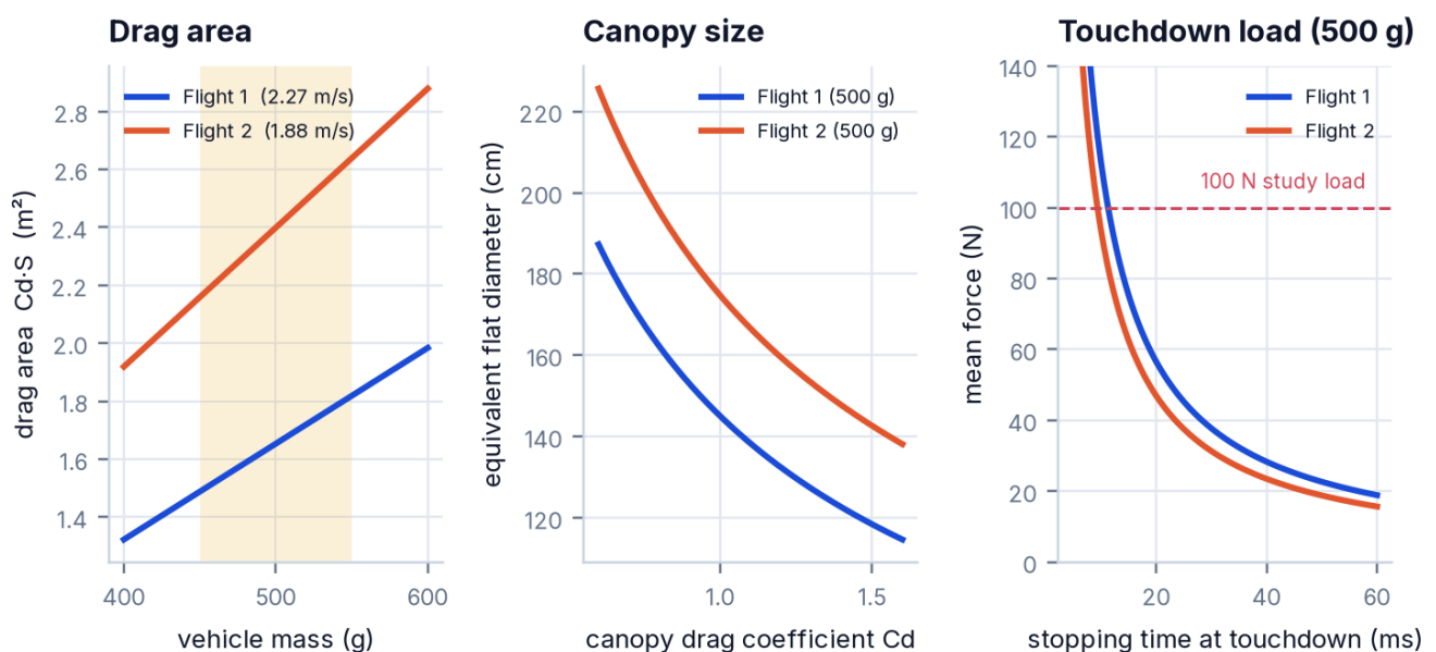
Figure 15 · Left: drag area ( Cd \cdot S ) implied by each flight's steady rate against vehicle mass. Centre: the equivalent flat canopy diameter against its drag coefficient. Right: mean touchdown force against stopping time, with the 100 N study load.
