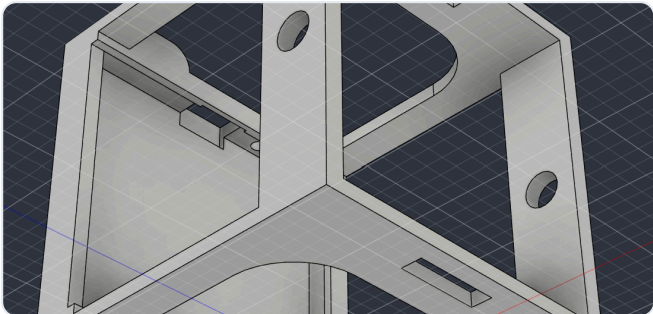
Render from below: arched openings, central spine and harness slots.
