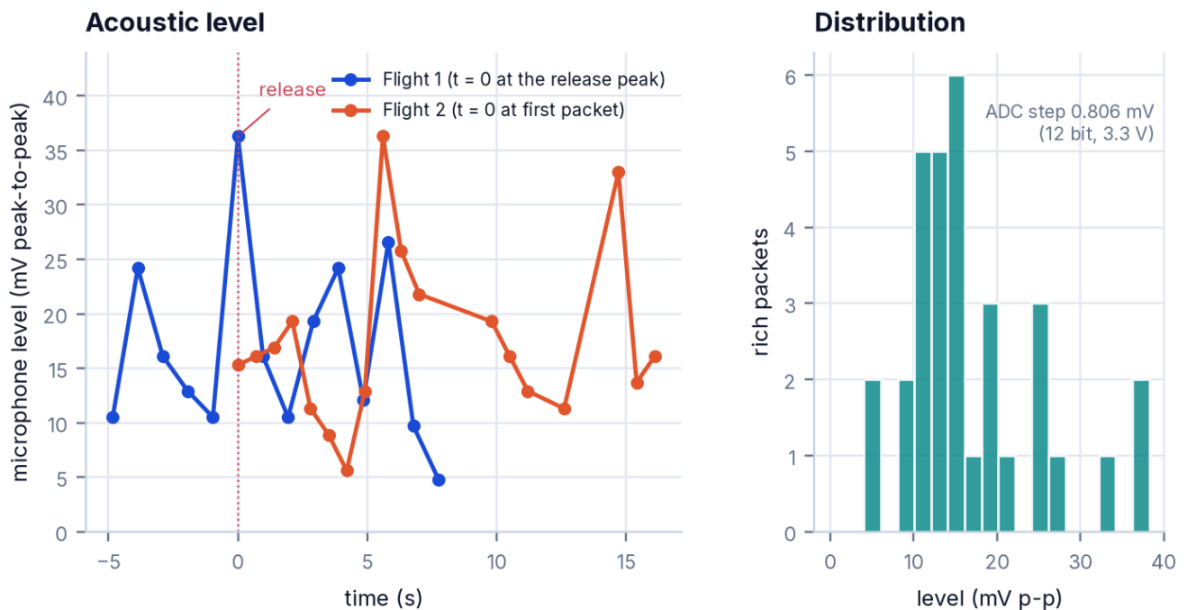
Figure 45 · Acoustic level against time (left) and its distribution (right). The loudest packet of Flight 1 is the release.
