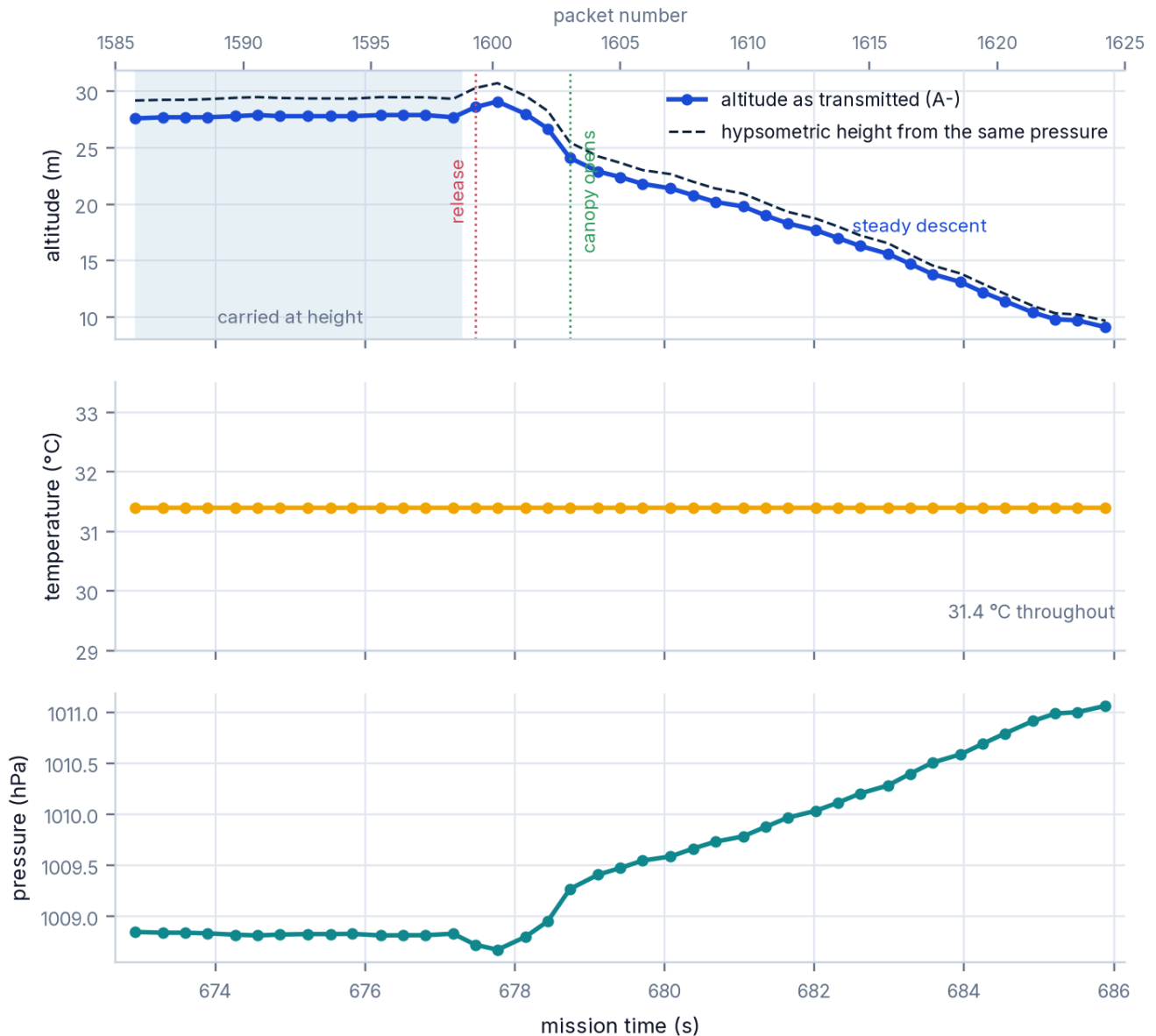
Figure 30 · Flight 1 — the three mandatory graphs. Altitude (as transmitted, and re-derived from the same pressure with the hypsonometric equation), temperature and pressure against mission time, with packet number along the top.
