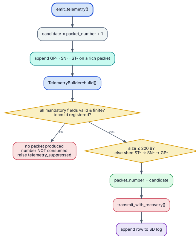
Figure 21 · Building a packet: validity, size shedding and the packet number.
