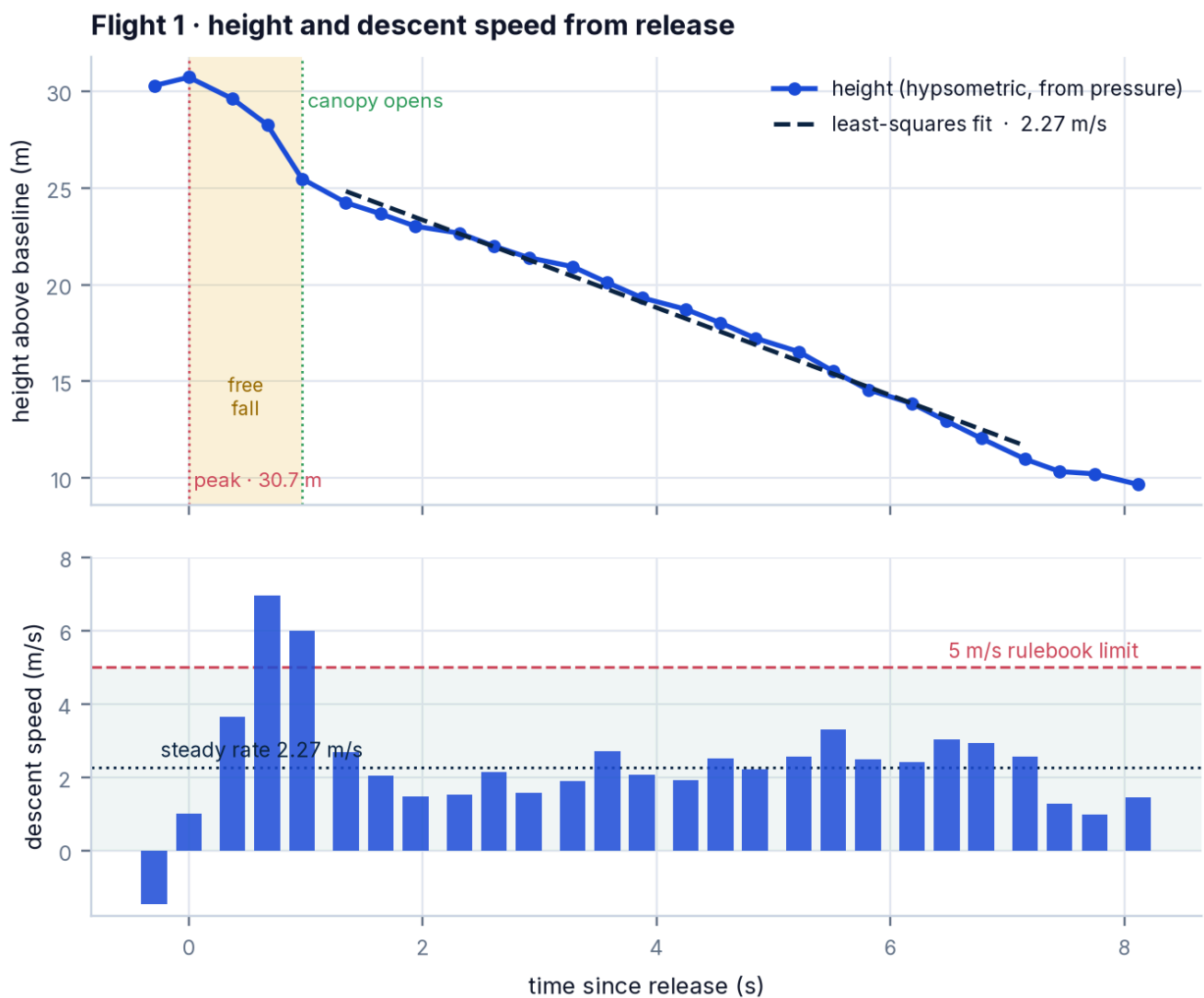
Figure 31 · Flight 1 — the descent. Top: height from the release peak, the free-fall segment shaded, and the least-squares line through the steady descent. Bottom: descent speed from successive packets against the 5 m/s limit.
