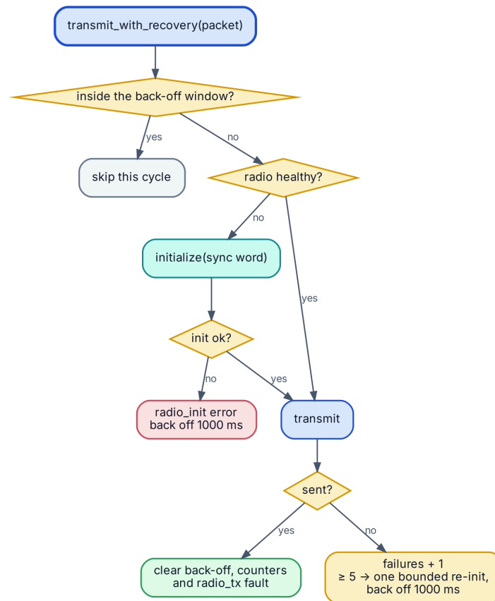
Figure 22 · Transmit with bounded recovery. A dead radio costs one initialisation per back-off window, never a blocking retry loop.
