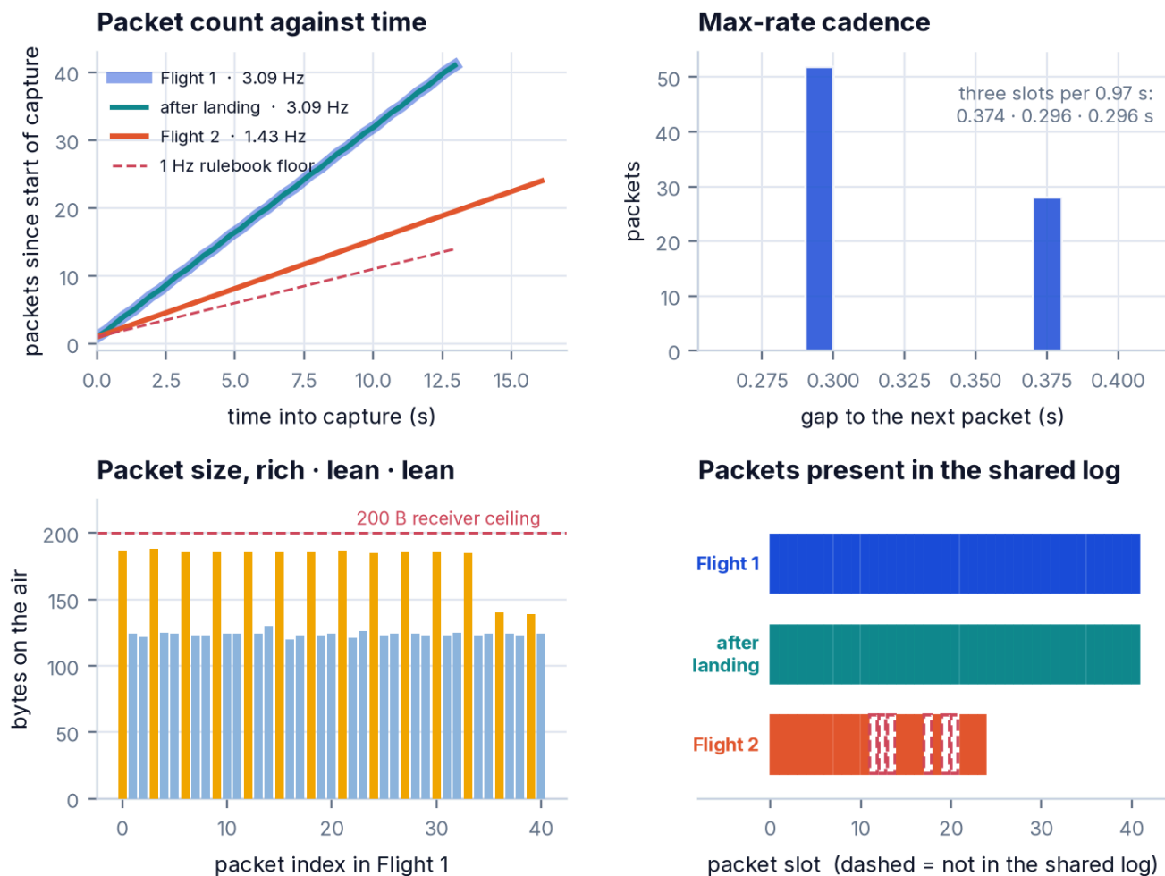
Figure 29 · Top left: packet count against time (the 1 Hz rulebook floor dashed). Top right: gaps between packets in the max-rate pattern. Bottom left: packet size by shape. Bottom right: which packet slots are present in the shared log.
