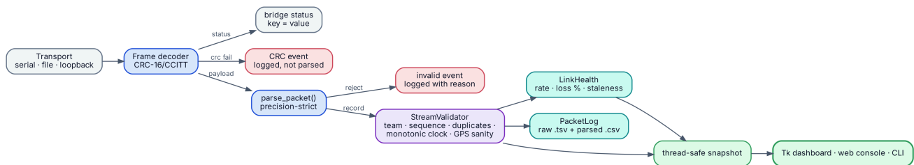
Figure 26 · The receive pipeline. Each stage counts its rejections separately, so a transport fault is never mistaken for a sensor fault.
