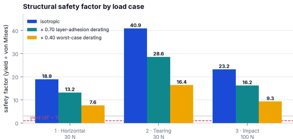
Figure 14 · Safety factor by load case: isotropic, and derated for the layered structure of a printed part.
