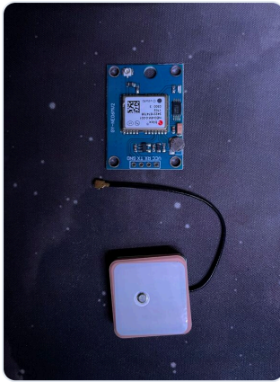
NEO-6M GPS with EEPROM and active patch antenna.
