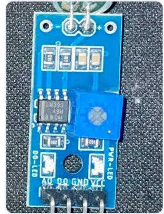
LM393 sound module: electret capsule, comparator and gain trimmer.
