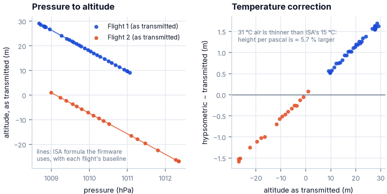
Figure 41 · Left: transmitted altitude against measured pressure for both flights, with the ISA formula (lines) using each flight's recovered baseline. Right: the difference between the temperature-corrected height and the transmitted altitude.
