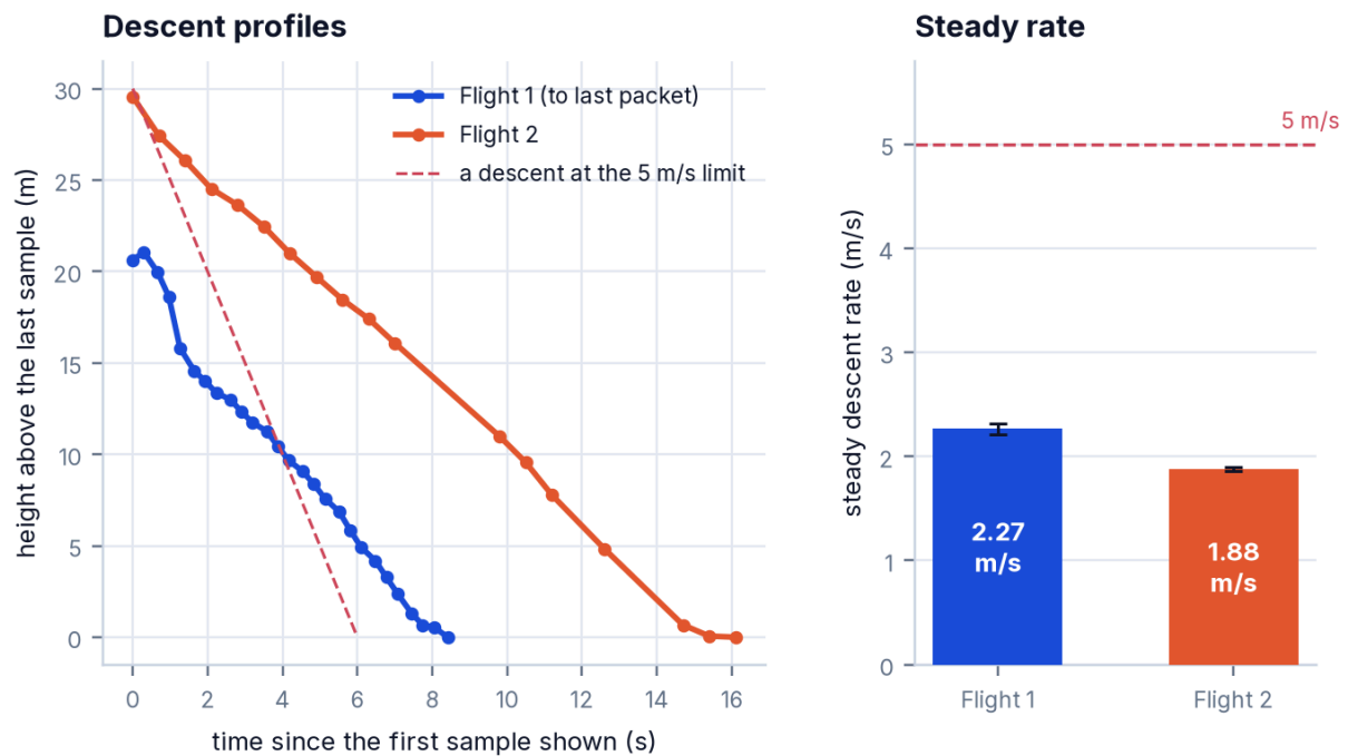
Figure 2 · The two descents on one axis, with the 5 m/s limit drawn as a reference line, and the steady rates.
