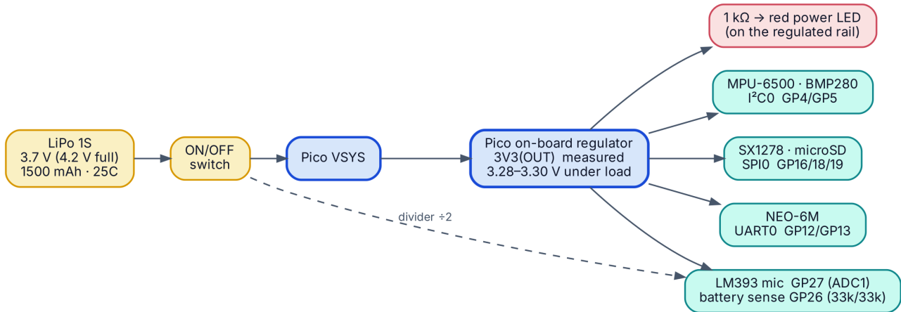
Figure 10 · From battery to every load. The switch sits in the battery lead ahead of everything; every peripheral runs from the Pico's own 3.3 V output.
