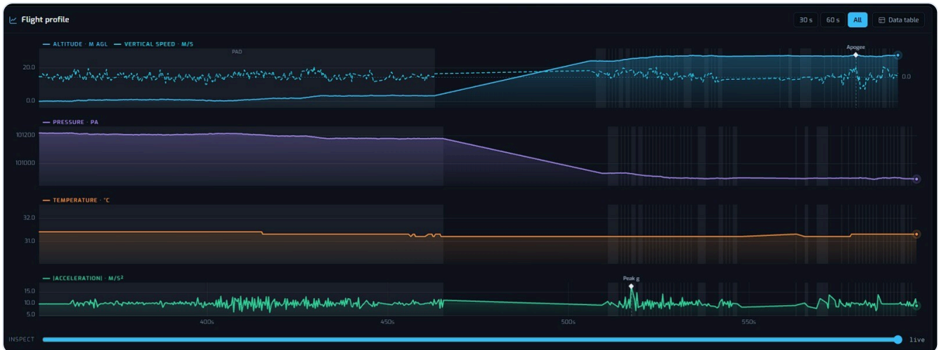
Figure 32 · Flight profile panel, live. Altitude above ground (and vertical speed), pressure, temperature and specific force against time, with the pad period shaded, the apogee and peak-g markers, a 30 s / 60 s / all window, a data-table view and an inspect slider that scrubs back through the record. Here the vehicle sits on the pad at 0 m, is carried up the building to about 27 m, and is held at height before the throw.
