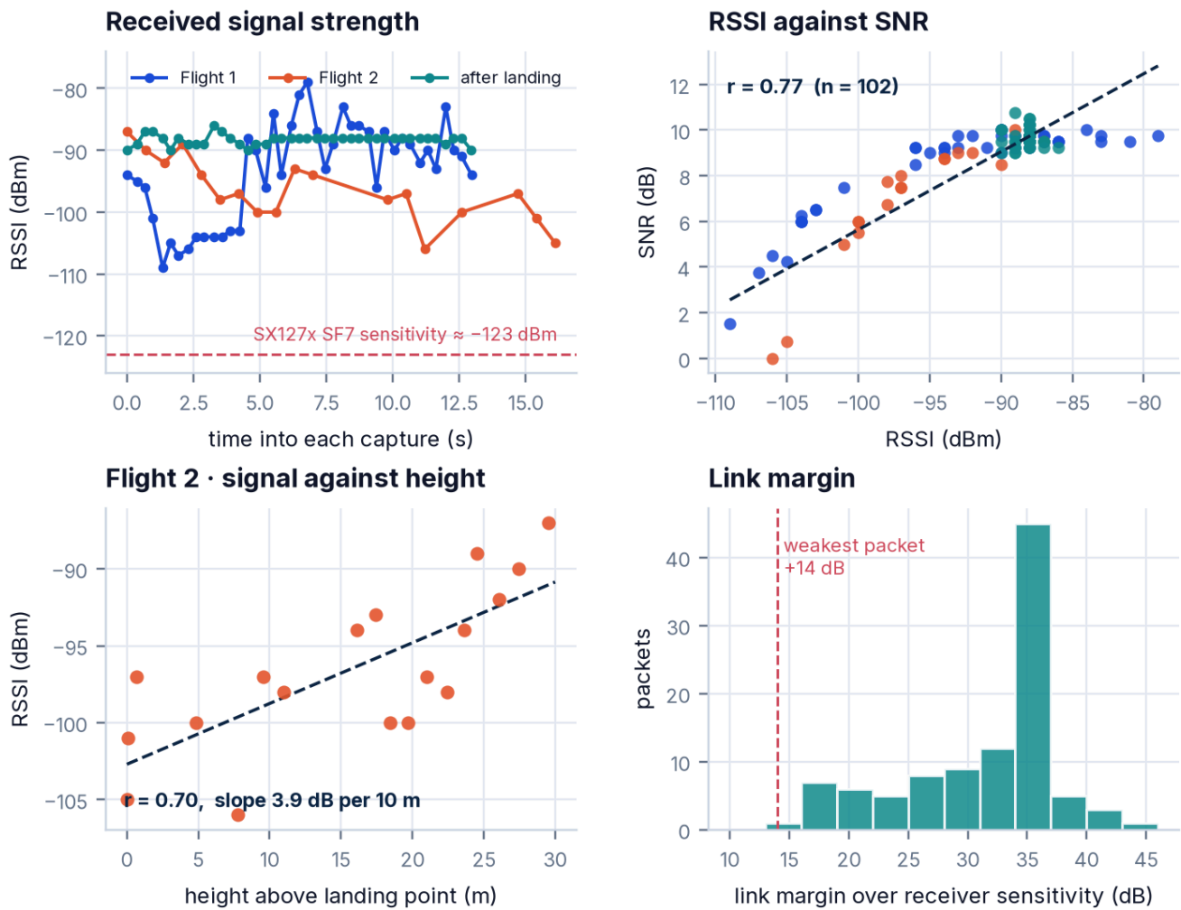
Figure 52 · Top left: RSSI against time into each capture, with the receiver's SF7 sensitivity. Top right: SNR against RSSI. Bottom left: Flight 2 RSSI against height above the landing point. Bottom right: link margin over receiver sensitivity for every packet.
