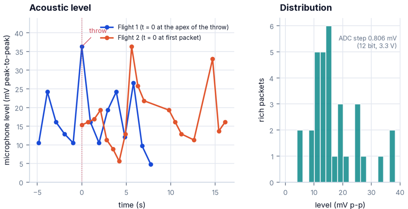
Figure 53 · Acoustic level against time (left) and its distribution (right). The loudest packet of Flight 1 is the throw.
