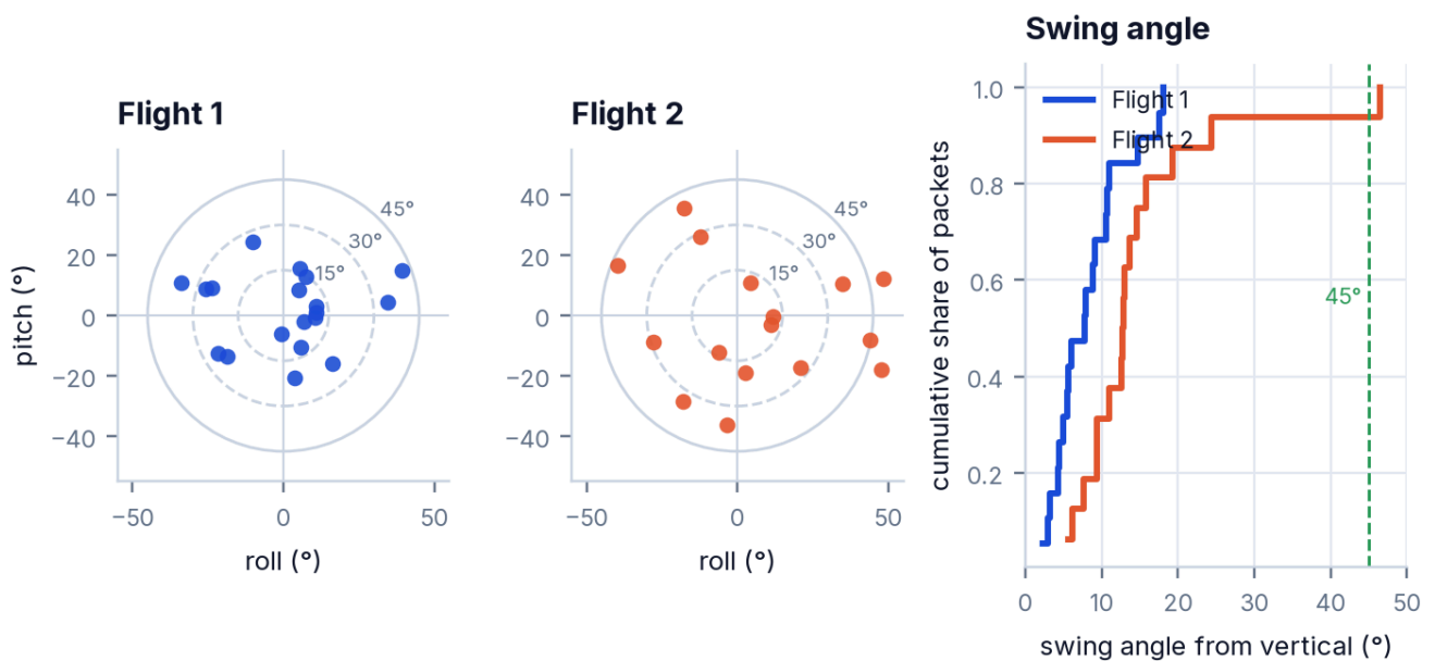
Figure 47 · The swing cone. Each dot is one packet of steady descent: roll against pitch, with 15°, 30° and 45° circles (left, centre); cumulative distribution of the swing angle (right). Flight 1 never leaves the 18° circle; Flight 2 stays inside 45° for 93 % of its packets.
