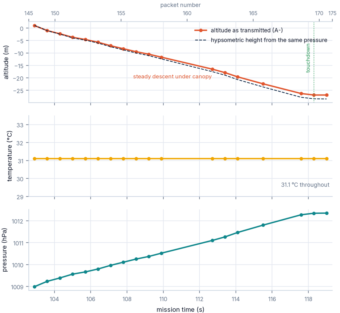
Figure 42 · Flight 2 — the three mandatory graphs. The transmitted altitude falls from +1.0 to -26.9 m relative to the vehicle's baseline; the pressure rises 335 Pa; temperature is a constant 31.1 °C.
