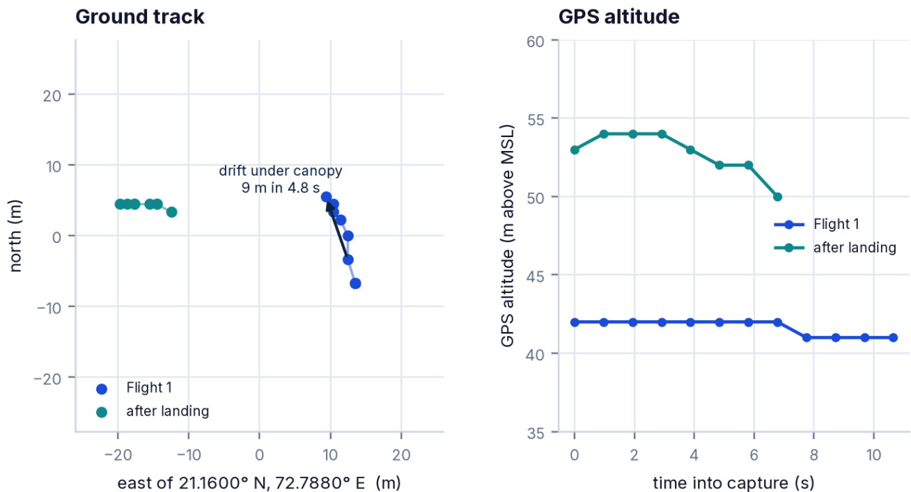
Figure 54 · Left: GPS fixes in the rich packets, in metres from a reference point, for Flight 1 and the after-landing session. Right: GPS altitude.
