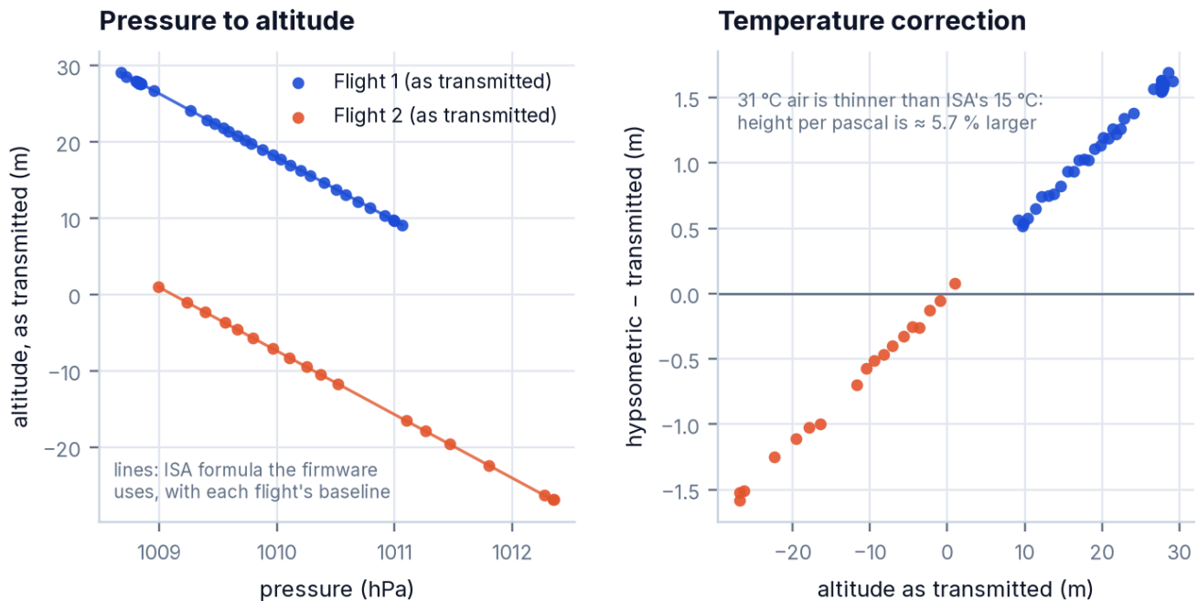
Figure 49 · Left: transmitted altitude against measured pressure for both flights, with the ISA formula (lines) using each flight's recovered baseline. Right: the difference between the temperature-corrected height and the transmitted altitude.
