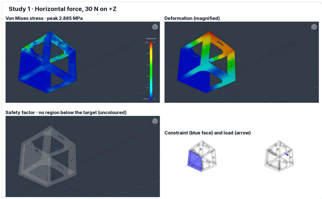
Figure 18 · Study 1 — horizontal force, 30 N on +Z. The stress concentrates around the arched cut-outs and where the central spine meets the top rail, peaking at 2.885 MPa; the safety-factor plot shows no region below the study target (the frame is left uncoloured).
