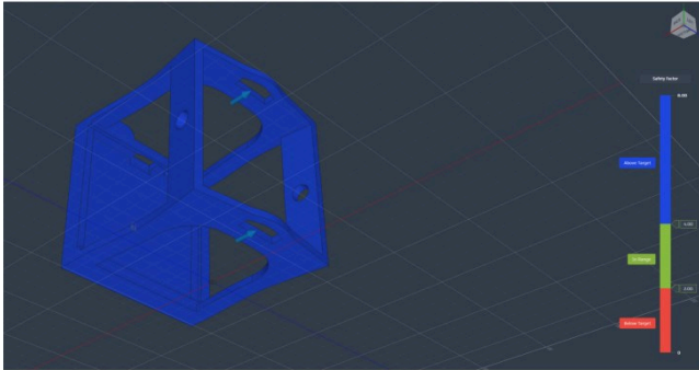
Figure 19 · Study 2 — tearing force, 30 N on -X. The lowest stresses of the three studies (peak 1.330 MPa) and a peak displacement of only 0.026 mm: the frame is very stiff against a pull on the harness points.
