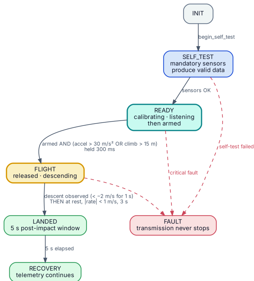
Figure 24 · Every transition and the guard on it. FAULT stops state progression, never transmission.
