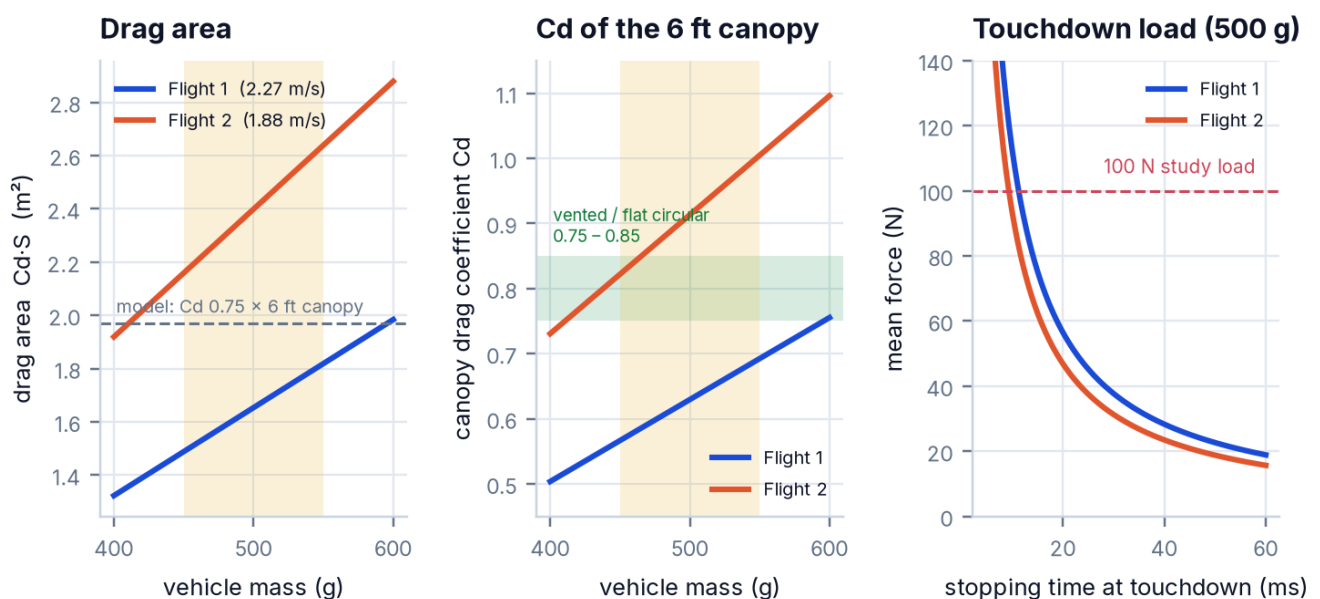
Figure 17 · Left: drag area ( Cd \cdot S ) implied by each flight's steady rate against vehicle mass, with the model's value for the 6 ft canopy. Centre: the drag coefficient of the 6 ft canopy that each flight implies. Right: mean touchdown force against stopping time, with the 100 N study load.
