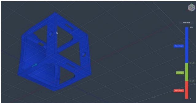
Figure 20 · Study 3 — impact force, 100 N on -X. The loaded panel bows (drawn magnified; the true peak displacement is 0.209 mm) and the stress spreads into the base and the neighbouring rails, peaking at 2.345 MPa, 4 % of the 54.4 MPa yield strength used in the study. The safety-factor plot is blue — above the study target — over the whole frame.
