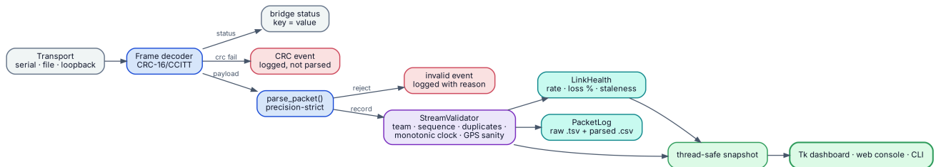
Figure 31 · The receive pipeline. Each stage counts its rejections separately, so a transport fault is never mistaken for a sensor fault.
