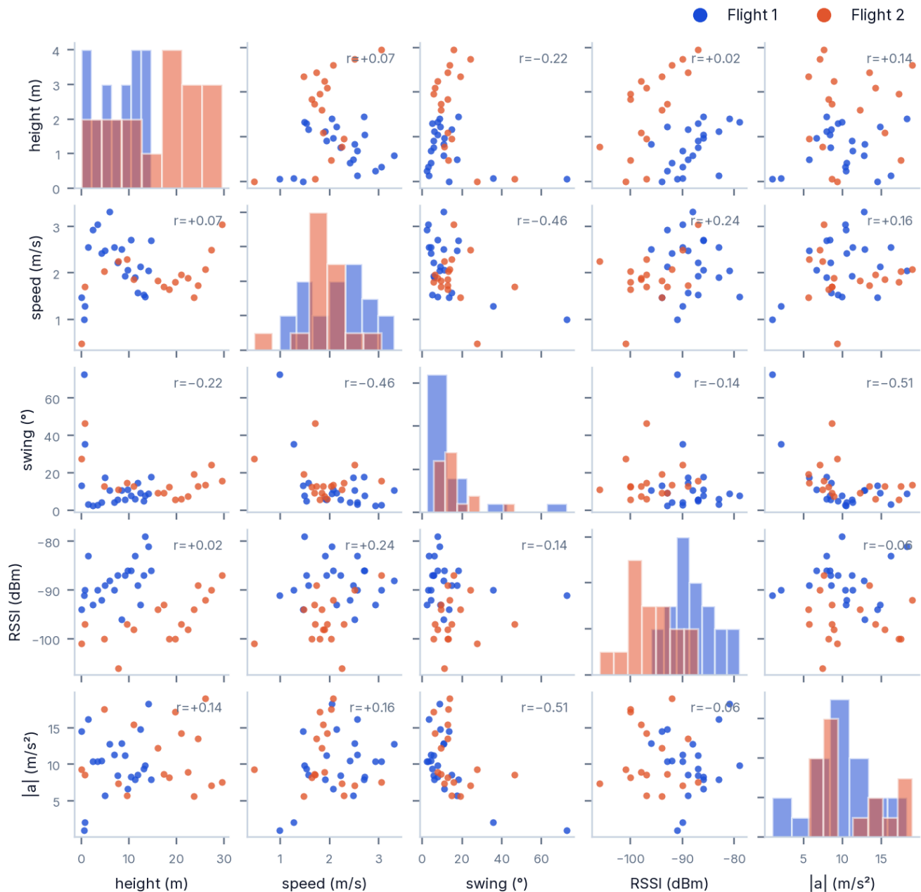
Figure 51 · Pair plot of height above the last sample, descent speed, swing angle, RSSI and specific force, both flights. The diagonal shows each variable's distribution.
