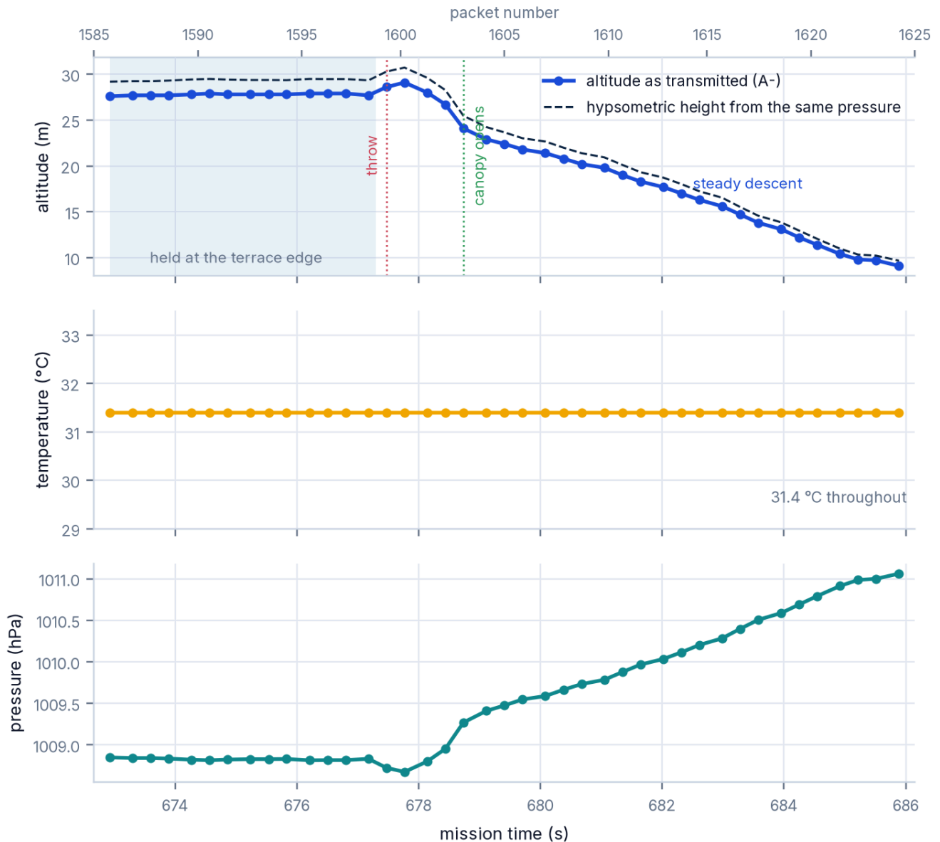
Figure 38 · Flight 1 — the three mandatory graphs. Altitude (as transmitted, and re-derived from the same pressure with the hypsonetric equation), temperature and pressure against mission time, with packet number along the top.
