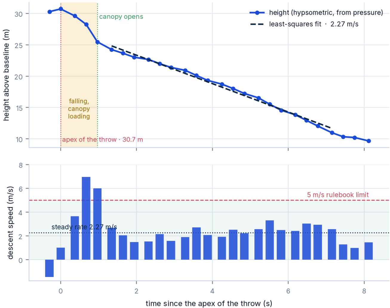
Figure 39 · Flight 1 — the descent. Top: height from the apex of the throw, the falling segment shaded, and the least-squares line through the steady descent. Bottom: descent speed from successive packets against the 5 m/s limit.
