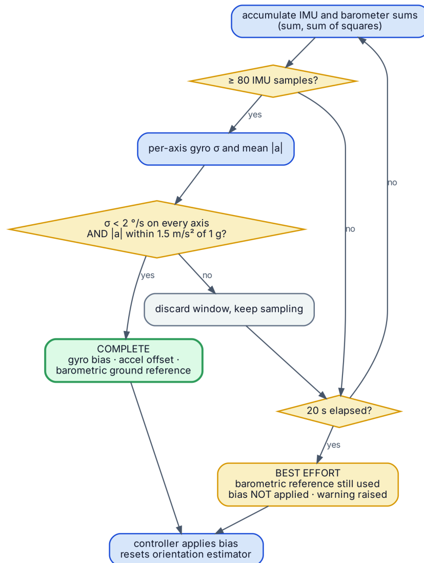
Figure 25 · Pad calibration. Best-effort still produces a usable barometric reference, because averaging pressure does not require stillness.
