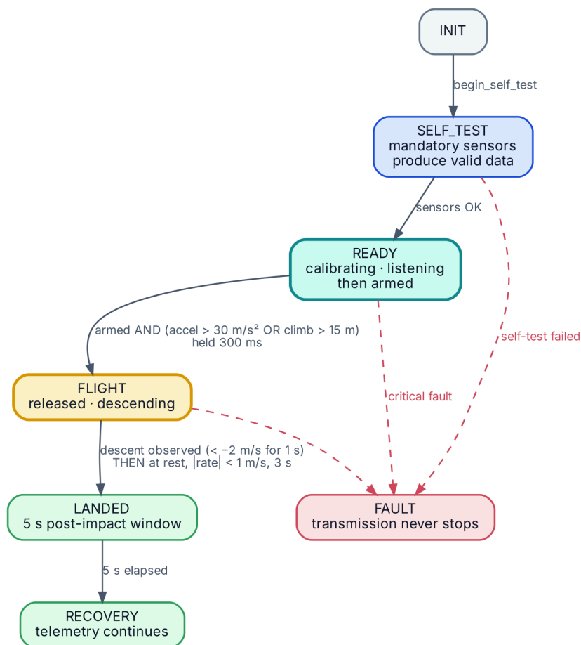
Figure 21 · Every transition and the guard on it. FAULT stops state progression, never transmission.
