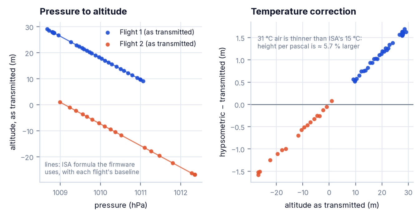
Figure 46 · Left: transmitted altitude against measured pressure for both flights, with the ISA formula (lines) using each flight's recovered baseline. Right: the difference between the temperature-corrected height and the transmitted altitude.
