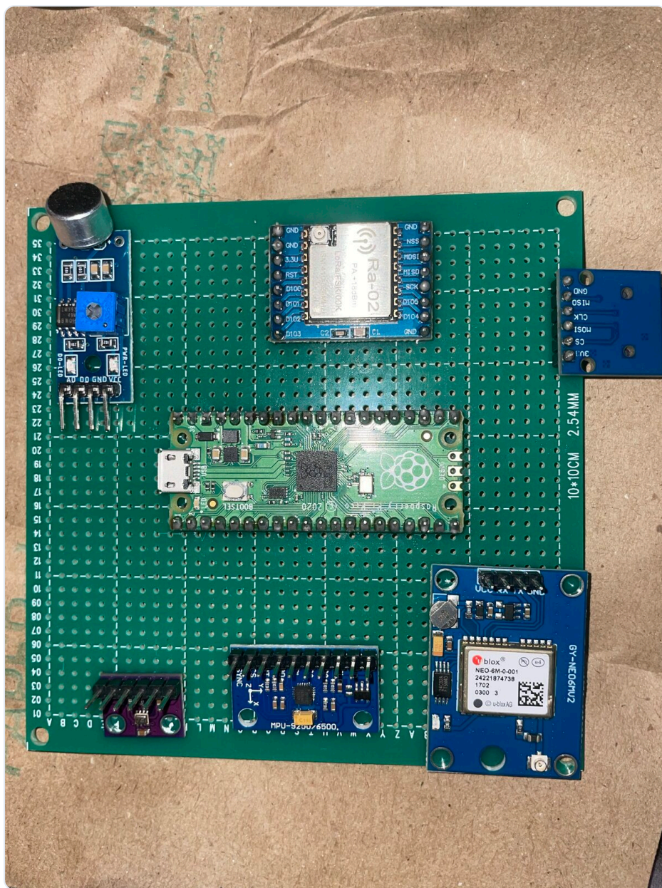
Figure 12 · The vehicle board, component side. 10 × 10 cm universal board with the microphone module (top left), RA-02 radio (top), microSD reader (right edge), Raspberry Pi Pico (centre), GPS module (lower right), IMU (lower centre) and BMP280 (lower left), laid out to keep the radio and card close to the Pico and the sensors on short I 2 C runs.
