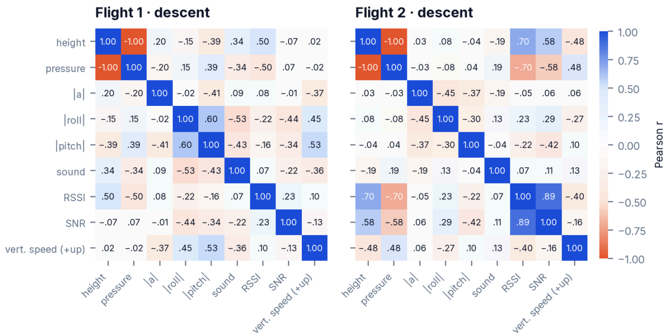
Figure 47 · Pearson correlation matrices for the descent of each flight. Height and pressure are one measurement seen twice ( r = -1.00 ).
