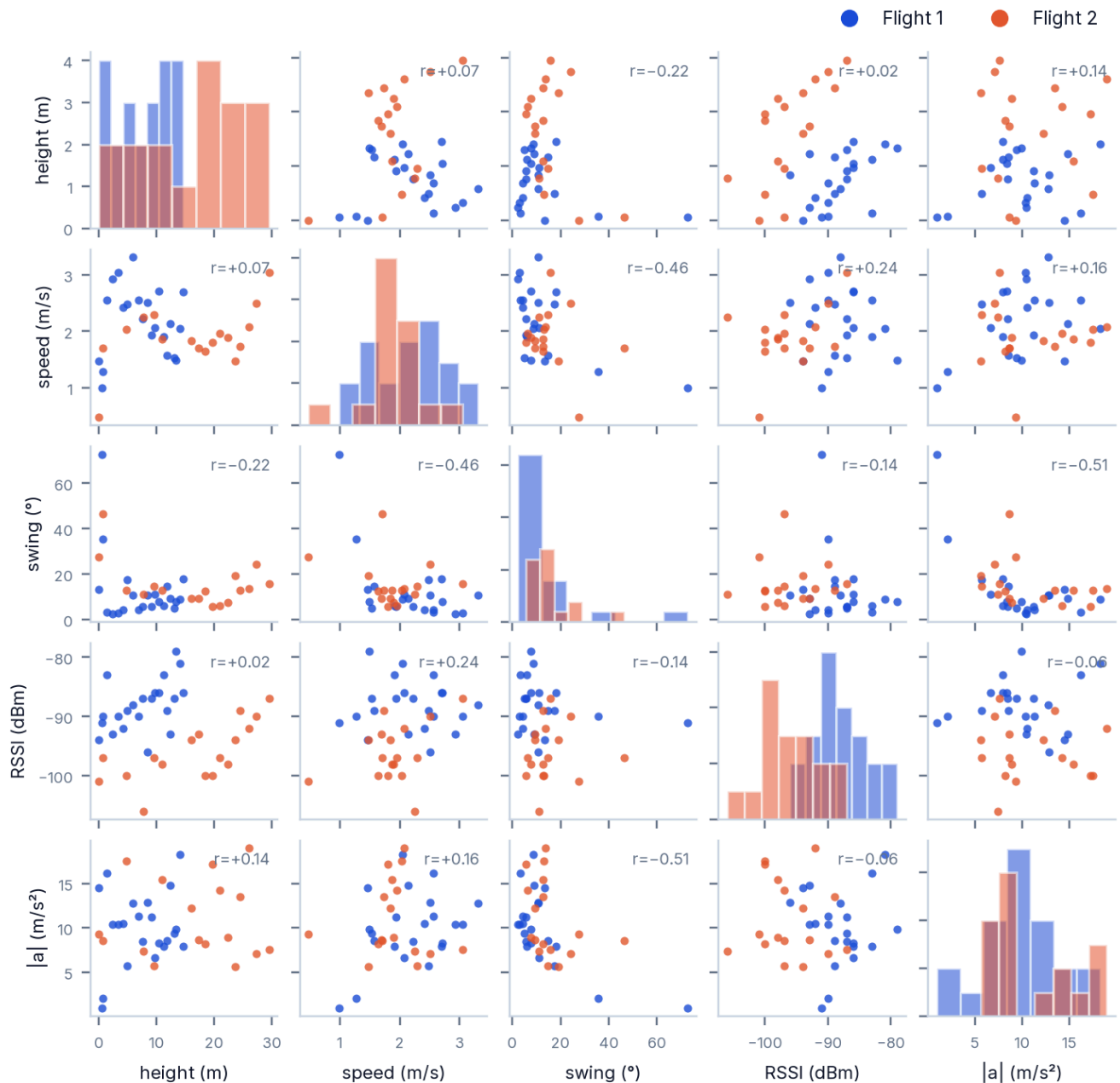
Figure 48 · Pair plot of height above the last sample, descent speed, swing angle, RSSI and specific force, both flights. The diagonal shows each variable's distribution.
