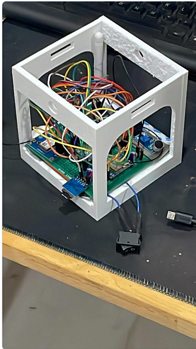
Figure 15 · The assembled CanSat. The white PETG frame carries the universal board with the GPS module, microphone module, radio and sensor modules; the 433 MHz antenna stands up through the frame; the rocker ON/OFF switch is on short leads outside, and the USB lead (right) is used for programming and bench work only.
