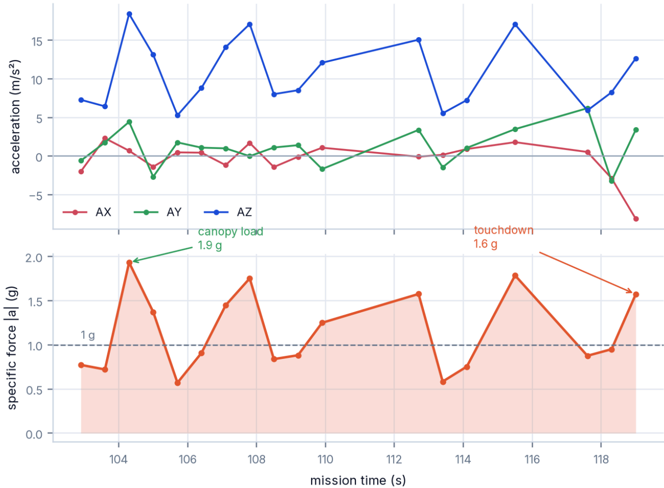
Figure 41 · Flight 2 — acceleration. Specific force stays within a band around 1 g, with the canopy load of 1.9 g at P-150 and a touchdown reading of 1.6 g.
