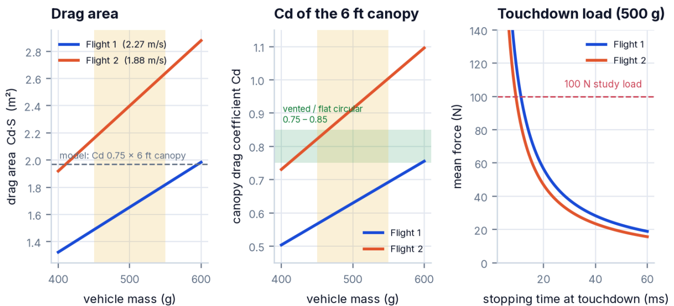
Figure 17 · Left: drag area ( C_d \cdot S ) implied by each flight's steady rate against vehicle mass, with the model's value for the 6 ft canopy. Centre: the drag coefficient of the 6 ft canopy that each flight implies. Right: mean touchdown force against stopping time, with the 100 N study load.
