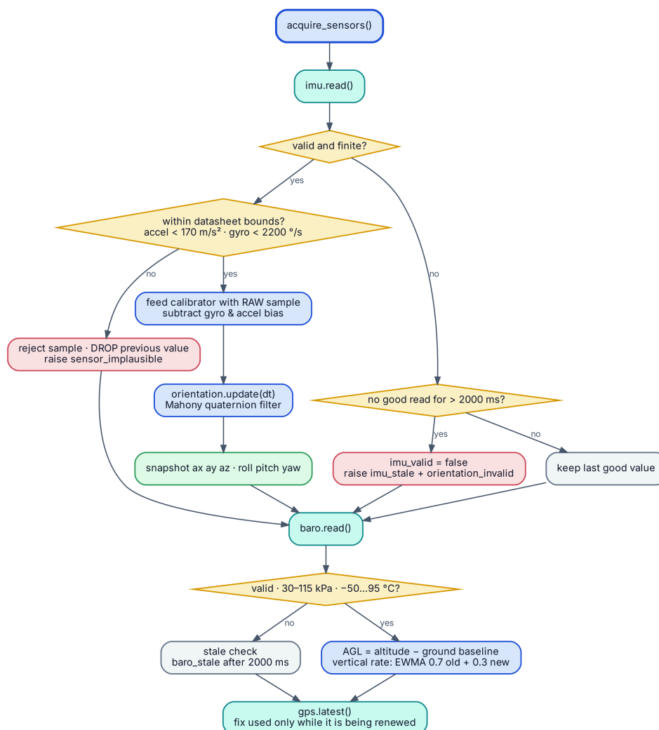
Figure 20 · Sensor acquisition every 33 ms: plausibility gating, staleness and the vertical-rate estimate.
