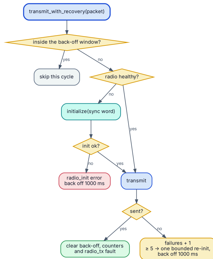
Figure 24 · Transmit with bounded recovery. A dead radio costs one initialisation per back-off window, never a blocking retry loop.
