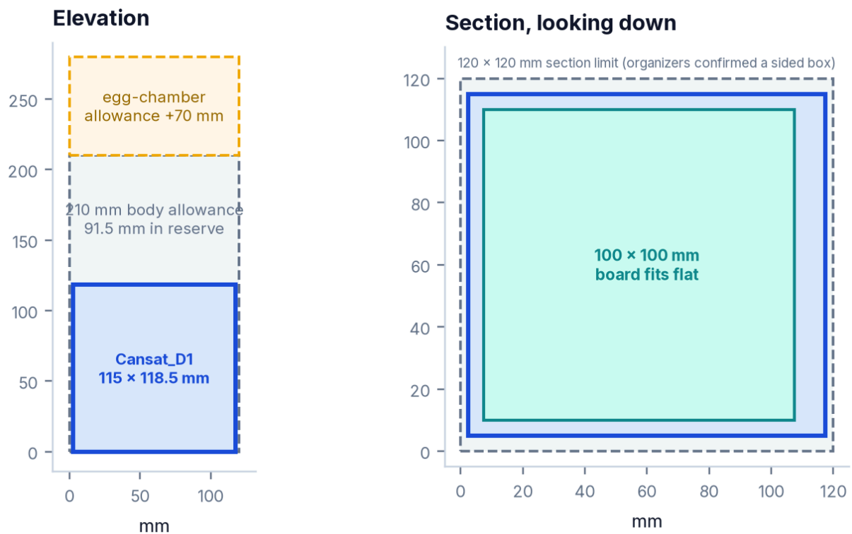
Figure 13 · The vehicle against the rulebook envelope: elevation (left) and the section looking down (right).
