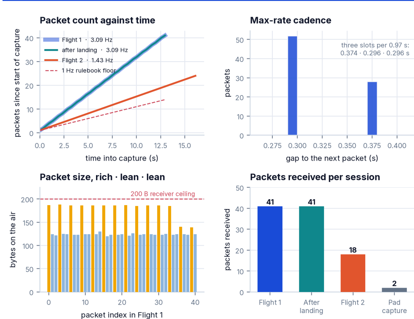
Figure 34 · Top left: packet count against time (the 1 Hz rulebook floor dashed). Top right: gaps between packets in the max-rate pattern. Bottom left: packet size by shape. Bottom right: packets received in each session.
