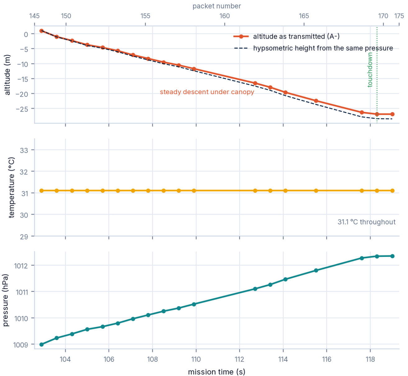
Figure 39 · Flight 2 — the three mandatory graphs. The transmitted altitude falls from +1.0 to -26.9 m relative to the vehicle's baseline; the pressure rises 335 Pa; temperature is a constant 31.1 °C.
