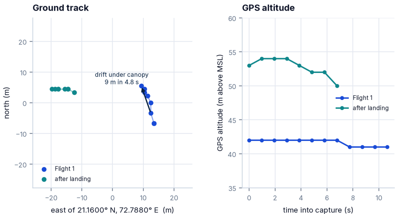
Figure 51 · Left: GPS fixes in the rich packets, in metres from a reference point, for Flight 1 and the after-landing session. Right: GPS altitude.
