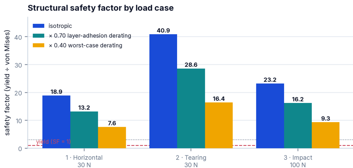
Figure 16 · Safety factor by load case: isotropic, and derated for the layered structure of a printed part.
