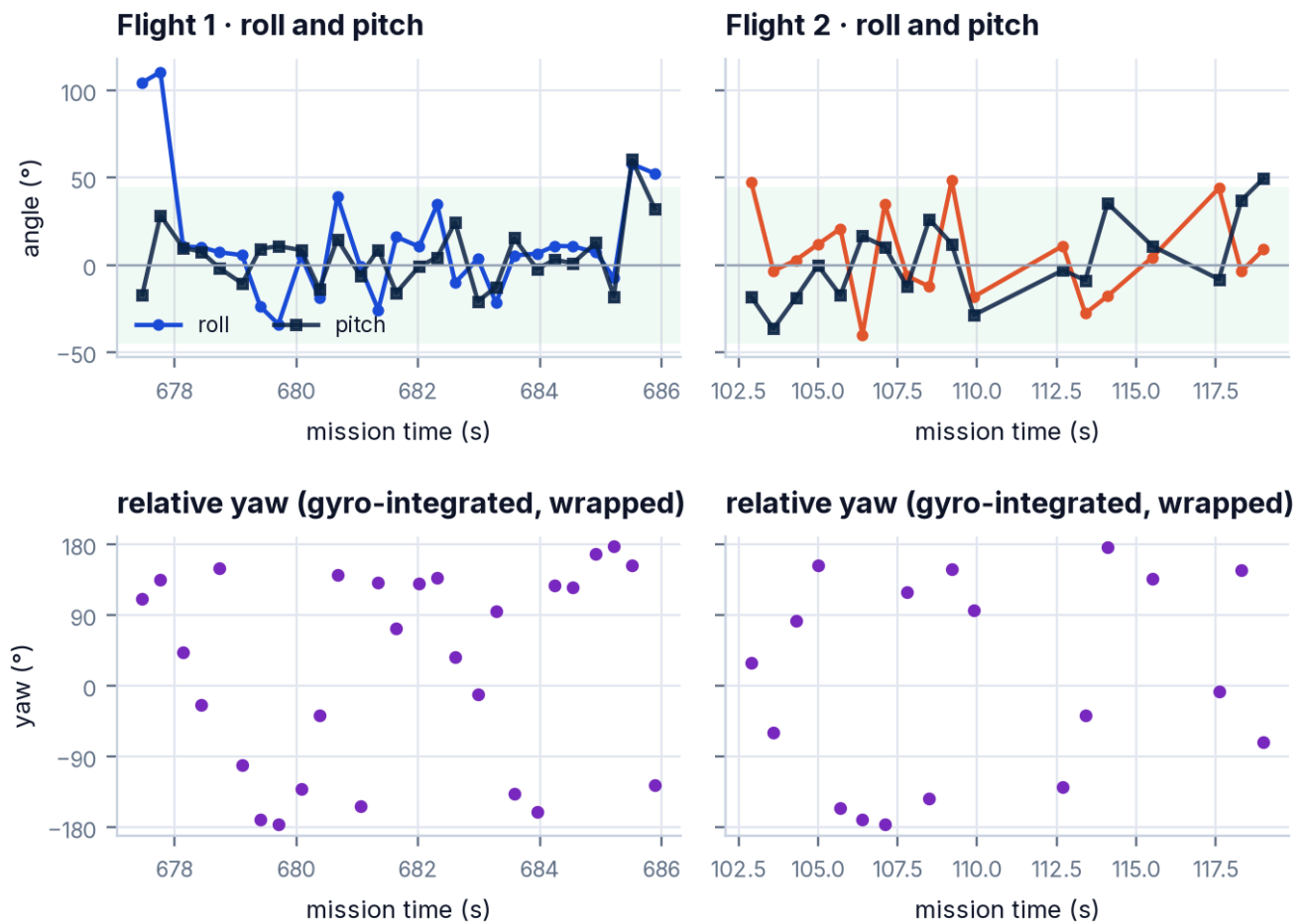
Figure 43 · Roll and pitch (top) and relative yaw (bottom) for both flights. Flight 1 starts at the throw, when the vehicle rotates from the orientation it was held in (roll \approx 110^\circ ) to upright within a packet.
