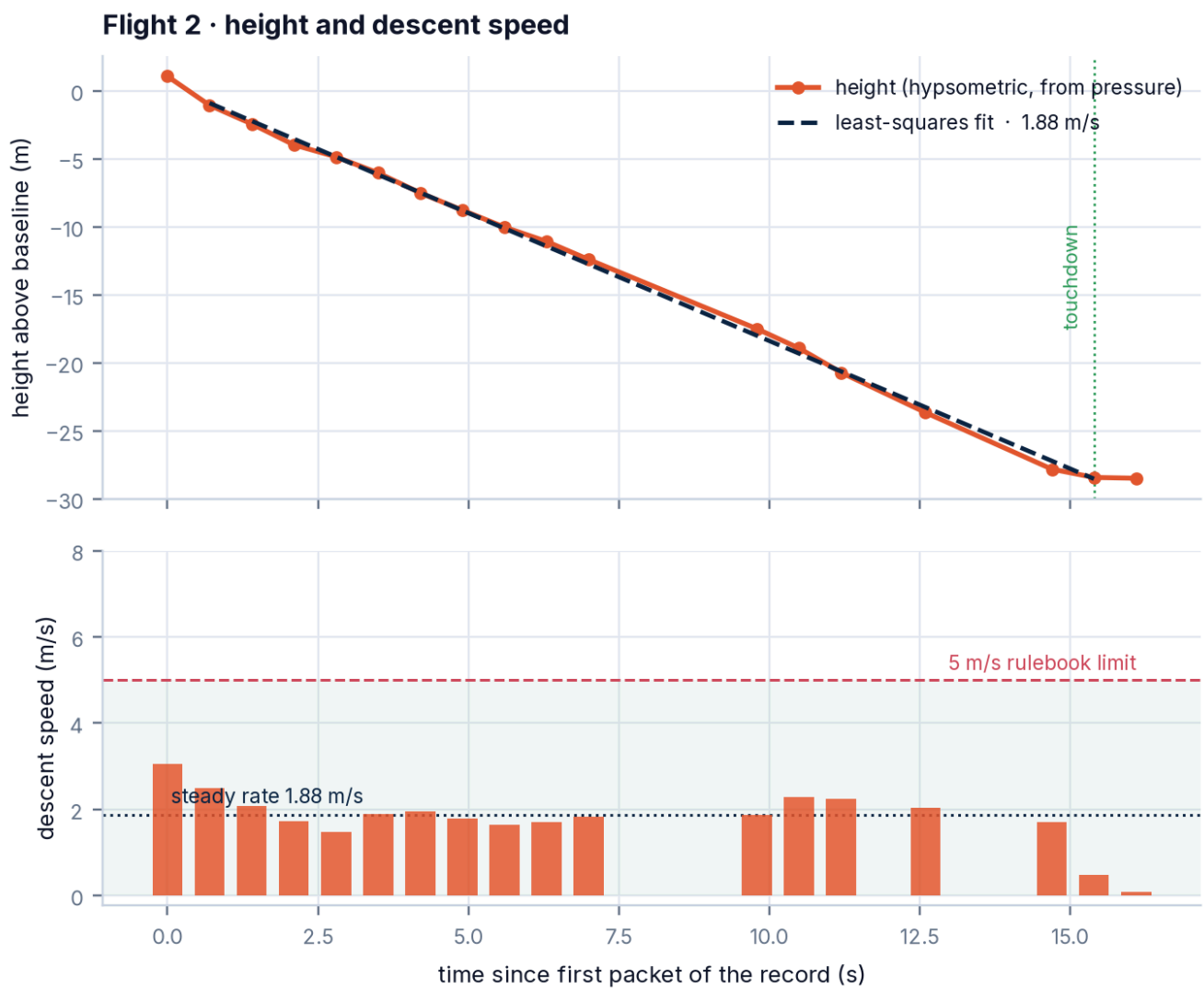
Figure 40 · Flight 2 — the descent. The least-squares line is straight to within the noise of the barometer ( R^2 = 0.999 ): the vehicle fell at constant speed from its first sample to touchdown. Bars are speeds between successive received packets.
